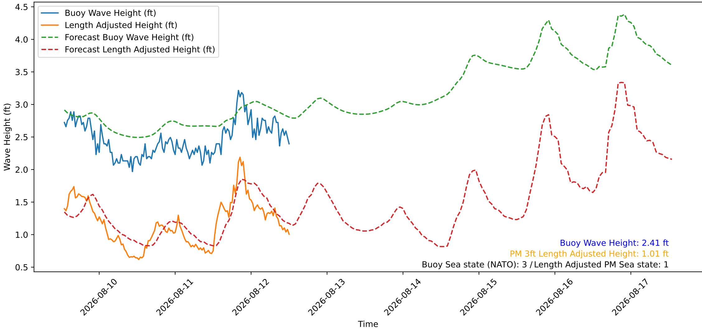
Wave Heights over Time for Green Beach at 2026-08-12 13:01:09
