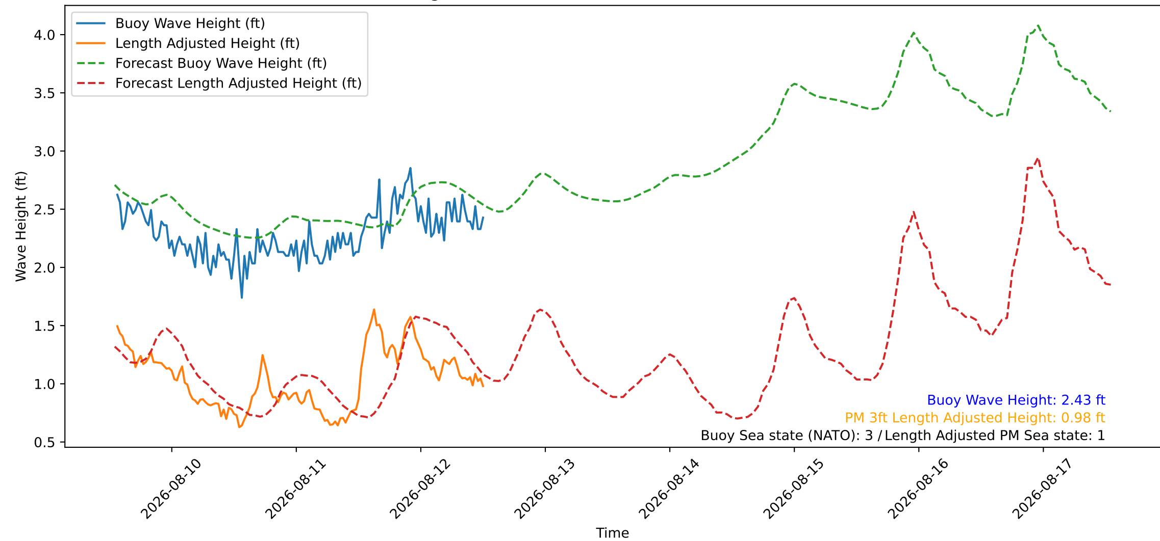
Wave Heights over Time for Red Beach at 2026-08-12 13:00:46
