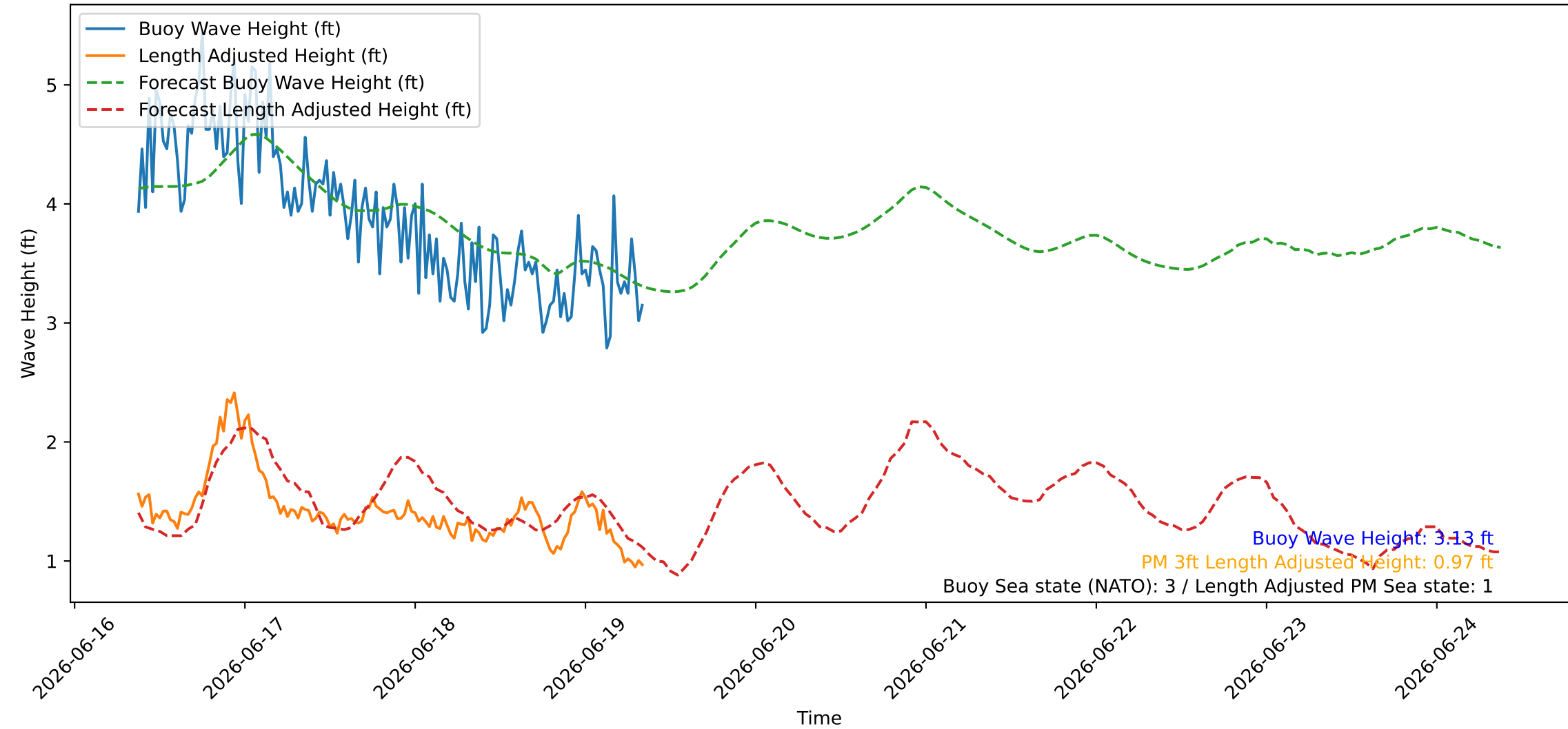
Wave Heights over Time for Oceanside Harbor at 2026-06-19 08:50:26
