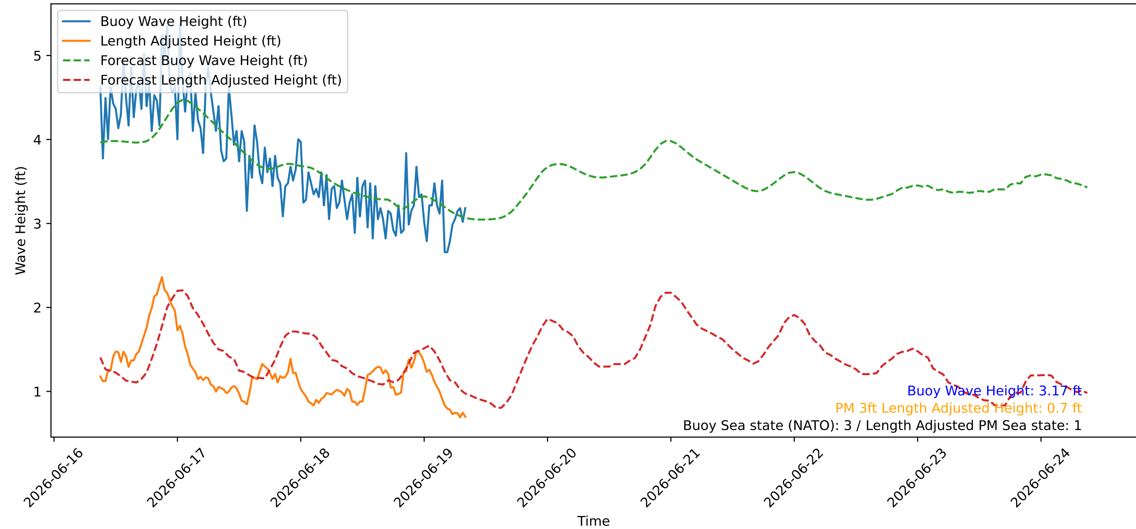
Wave Heights over Time for Red Beach at 2026-06-19 08:50:46
