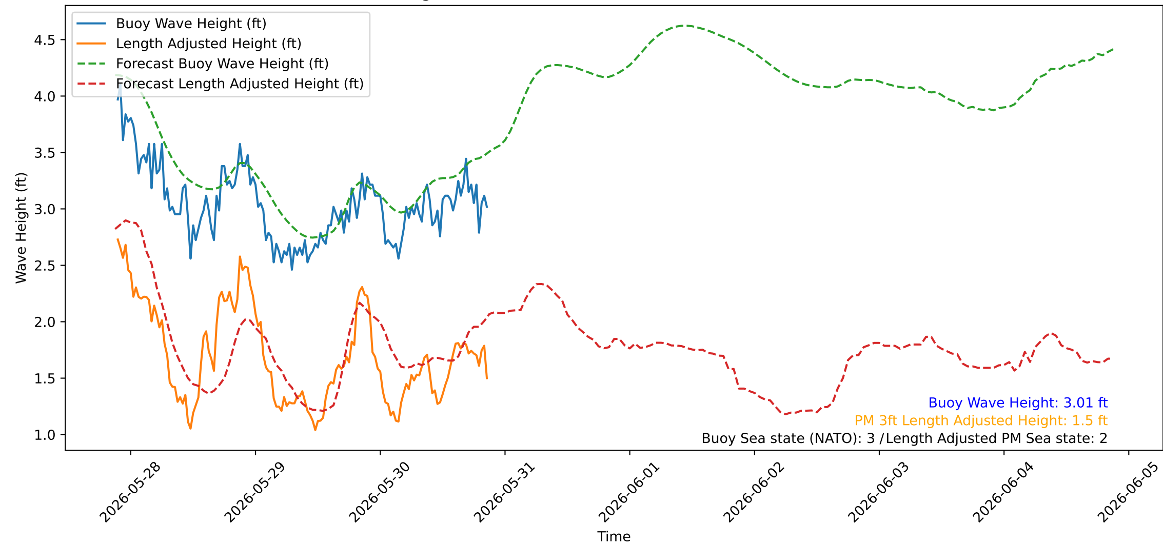
Wave Heights over Time for Green Beach at 2026-05-30 21:21:07
