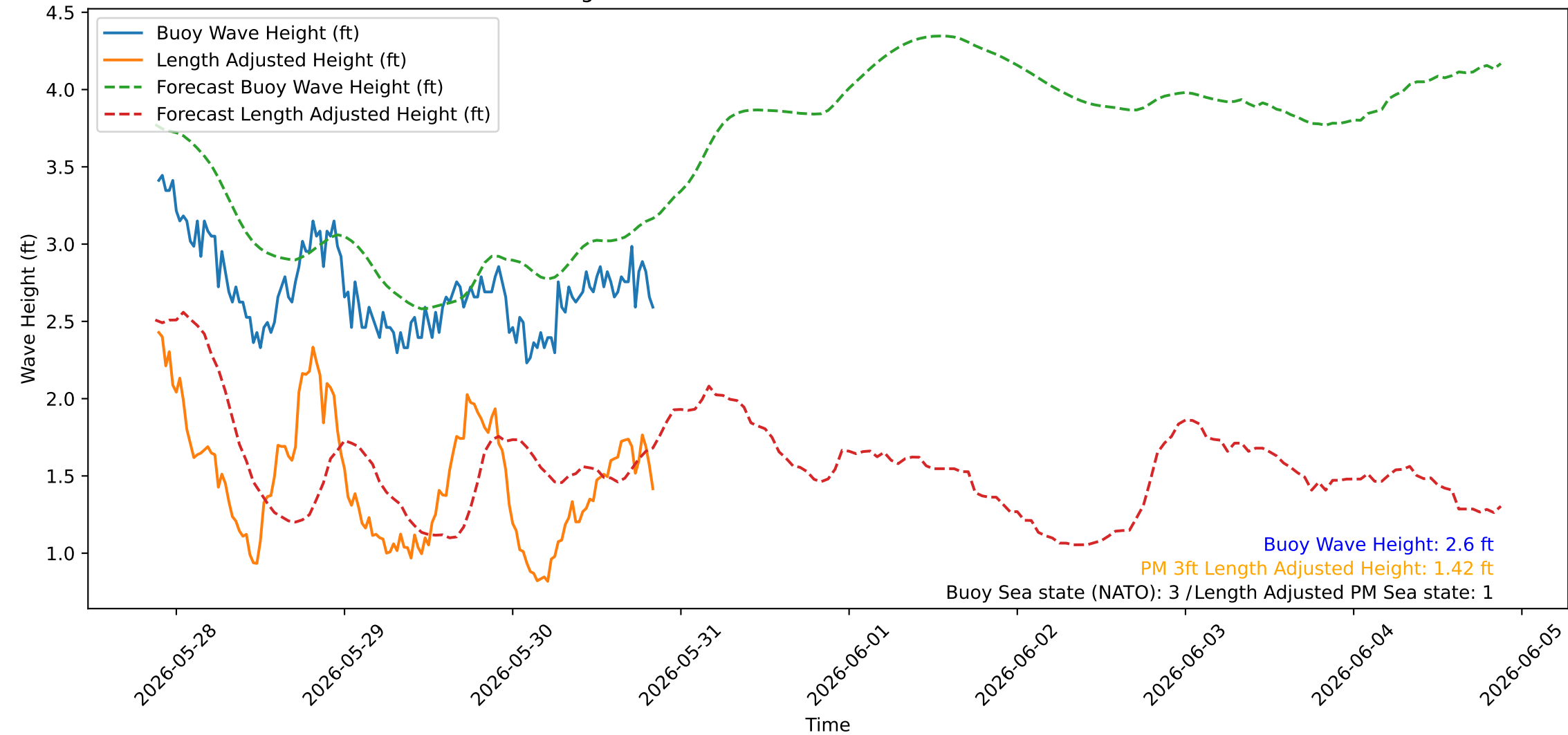
Wave Heights over Time for Red Beach at 2026-05-30 21:20:44
