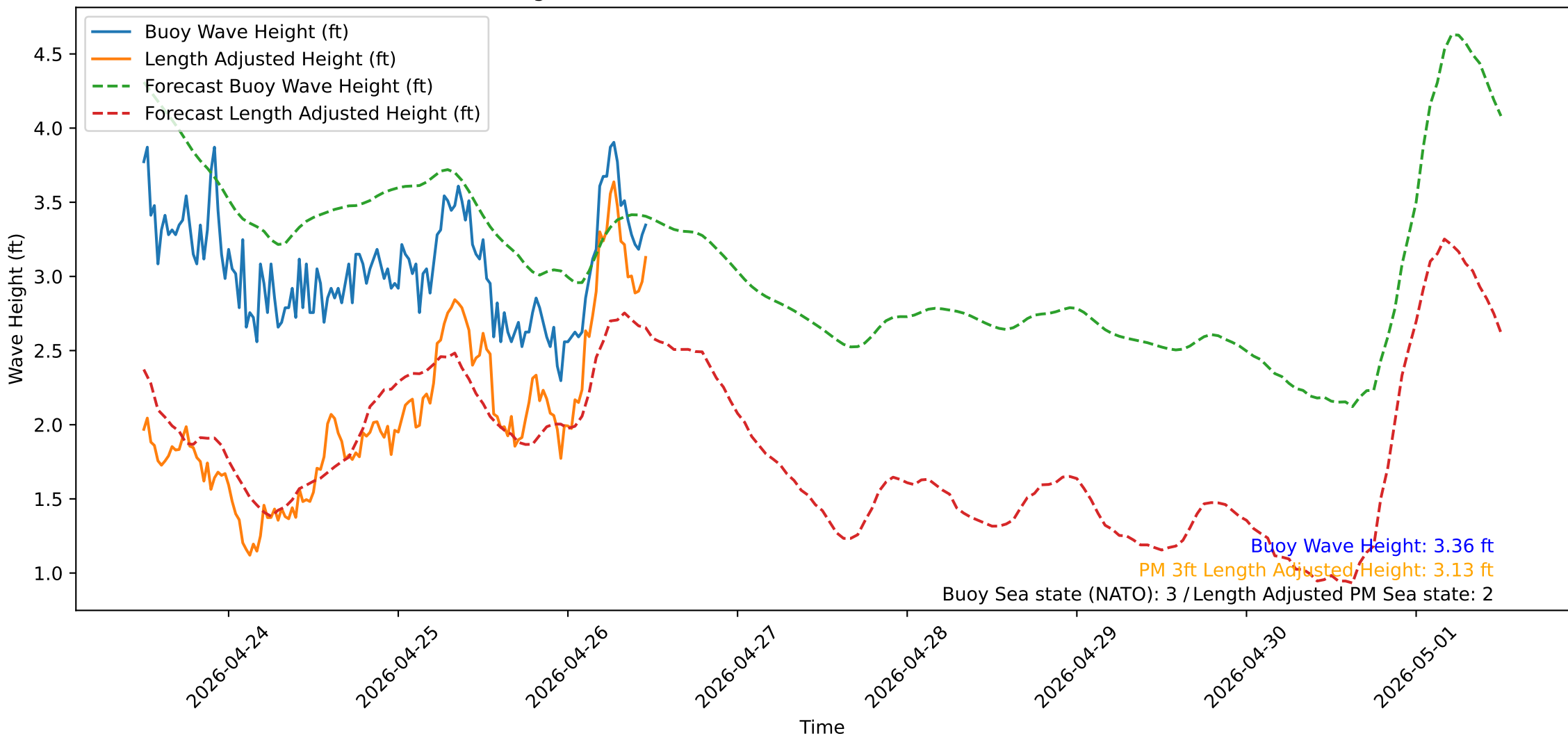
Wave Heights over Time for Oceanside Harbor at 2026-04-26 11:50:31
