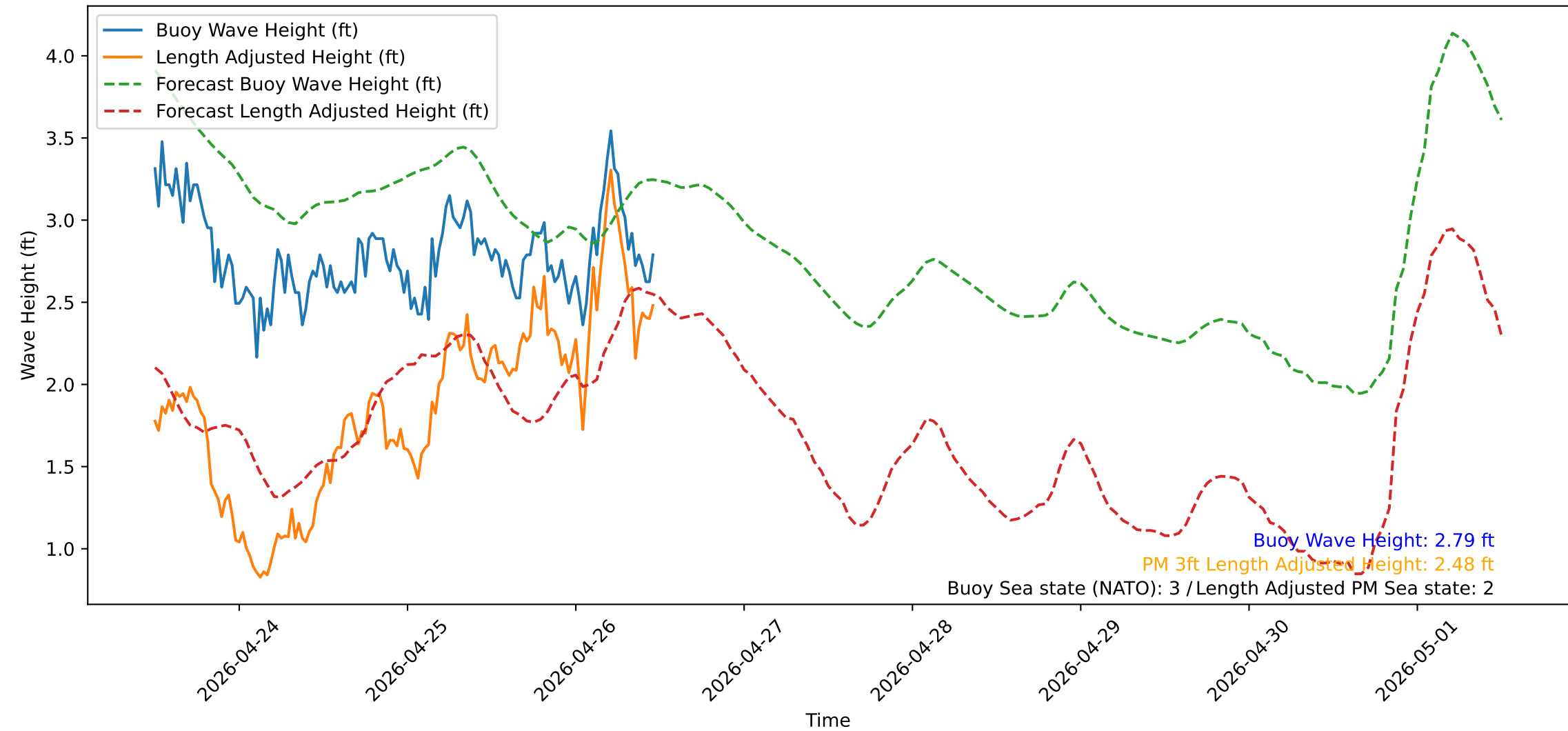
Wave Heights over Time for Red Beach at 2026-04-26 11:50:51
