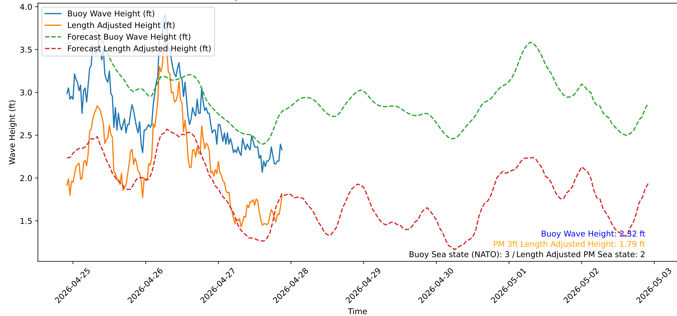
Wave Heights over Time for Oceanside Harbor at 2026-04-27 21:50:31
