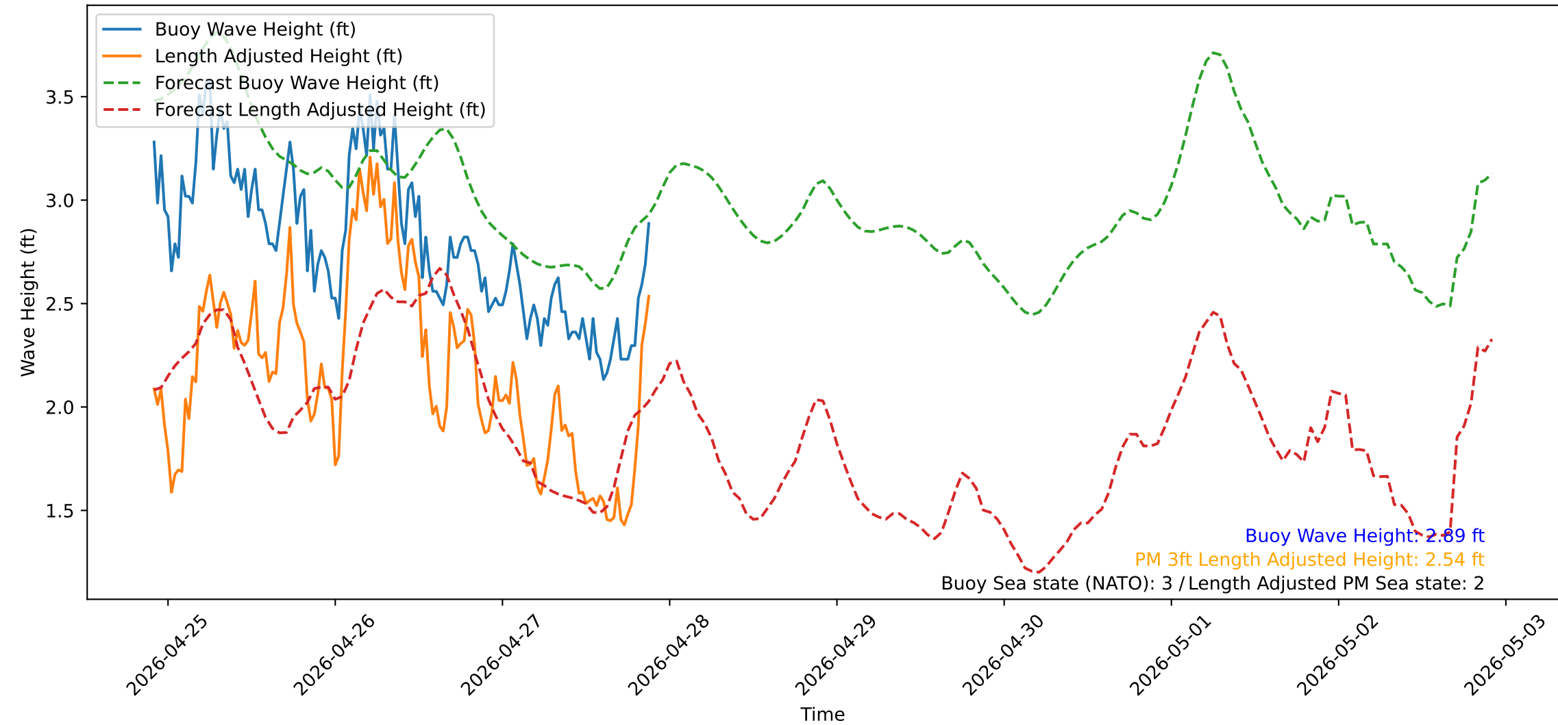
Wave Heights over Time for Green Beach at 2026-04-27 21:51:14
