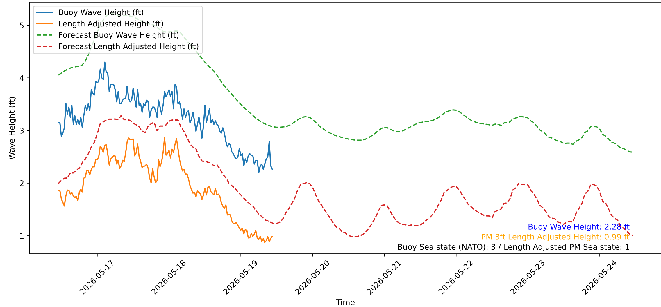
Wave Heights over Time for Oceanside Harbor at 2026-05-19 11:00:31
