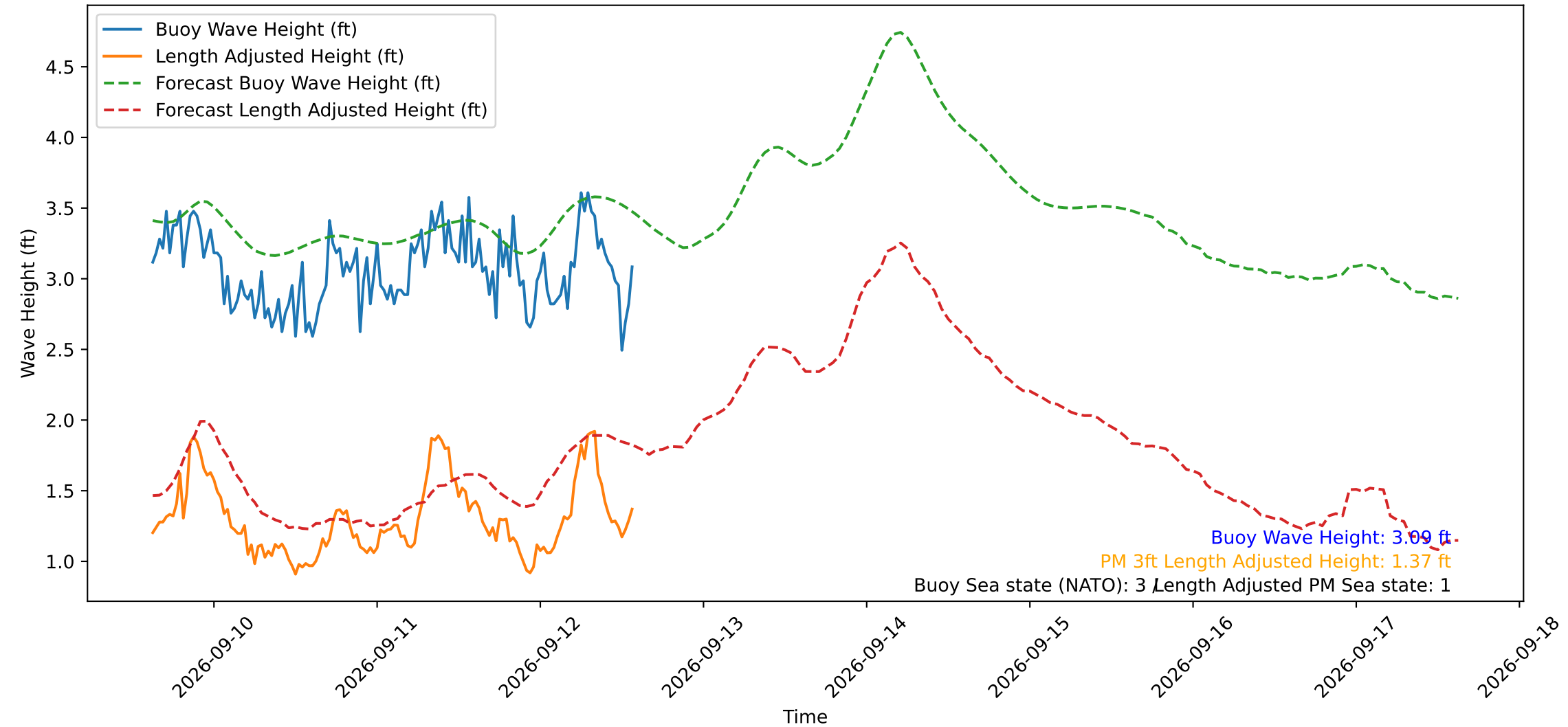
Wave Heights over Time for Green Beach at 2026-09-12 14:31:17
