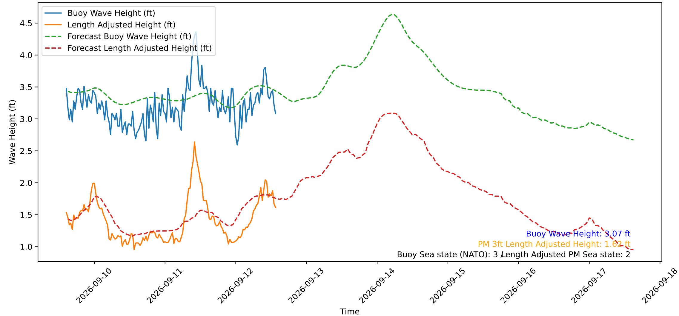
Wave Heights over Time for Oceanside Harbor at 2026-09-12 14:30:31
