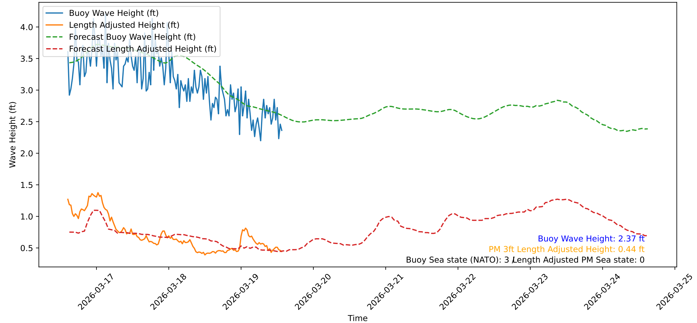
Wave Heights over Time for Green Beach at 2026-03-19 14:31:10
