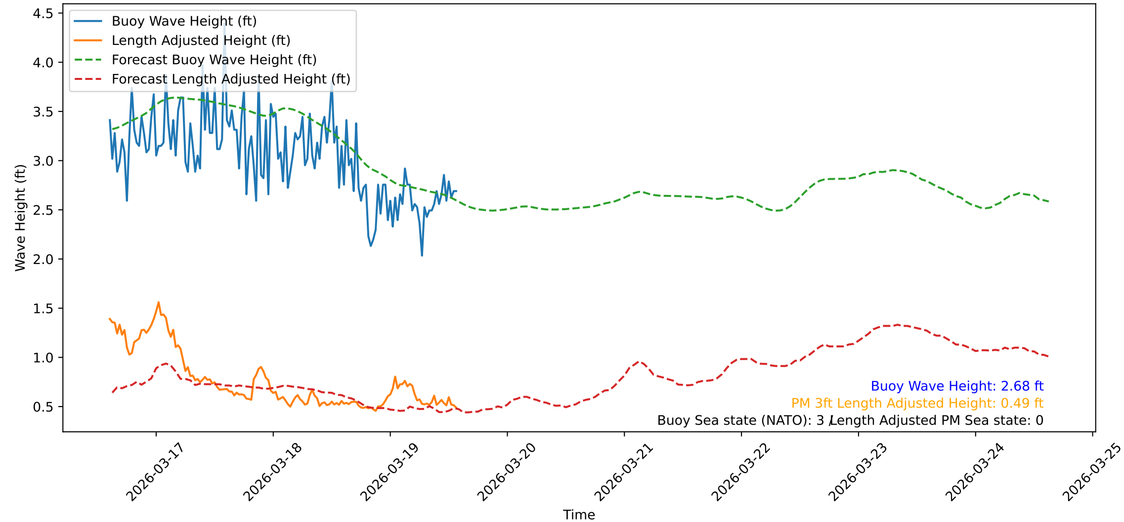
Wave Heights over Time for Oceanside Harbor at 2026-03-19 14:30:32
