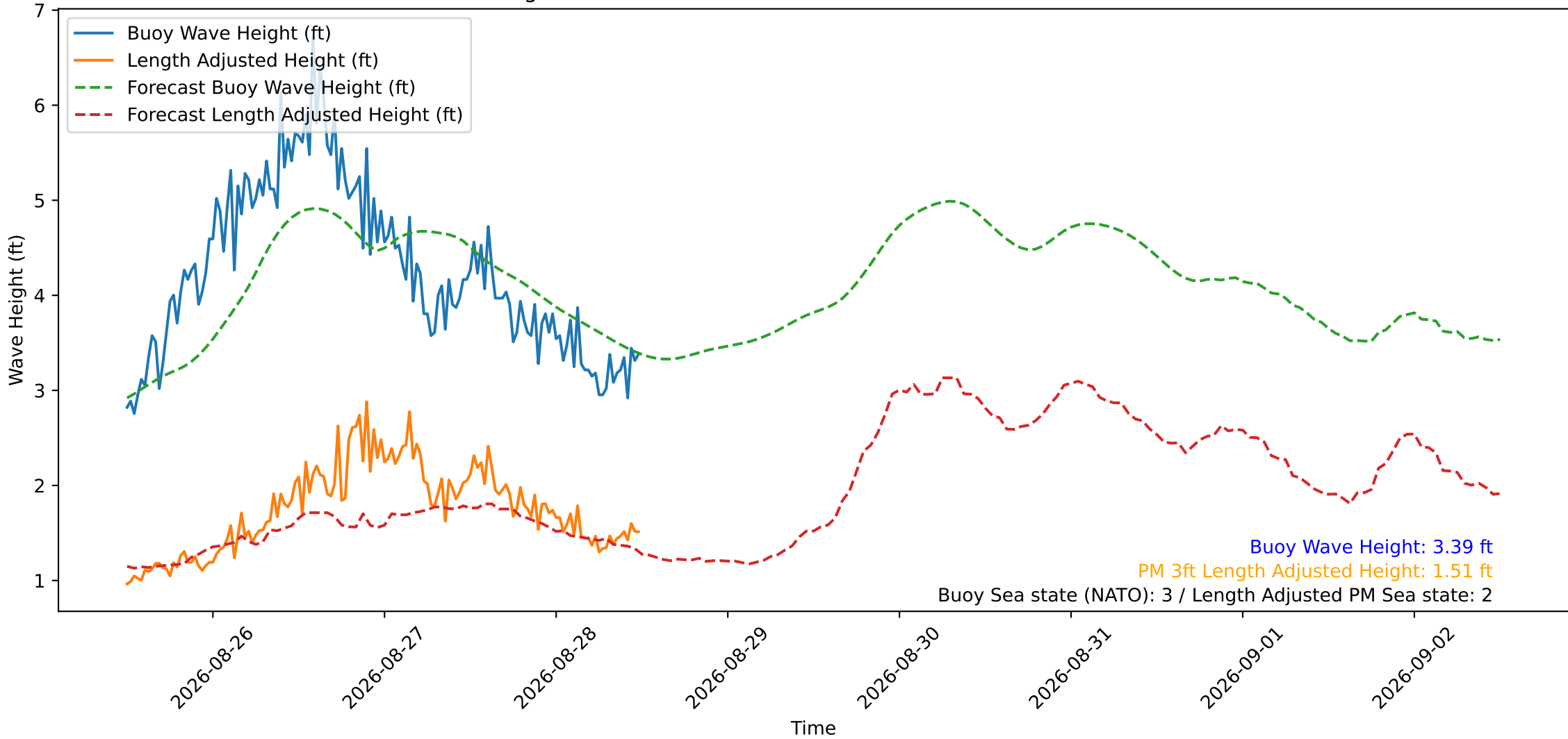
Wave Heights over Time for Oceanside Harbor at 2026-08-28 12:10:30
