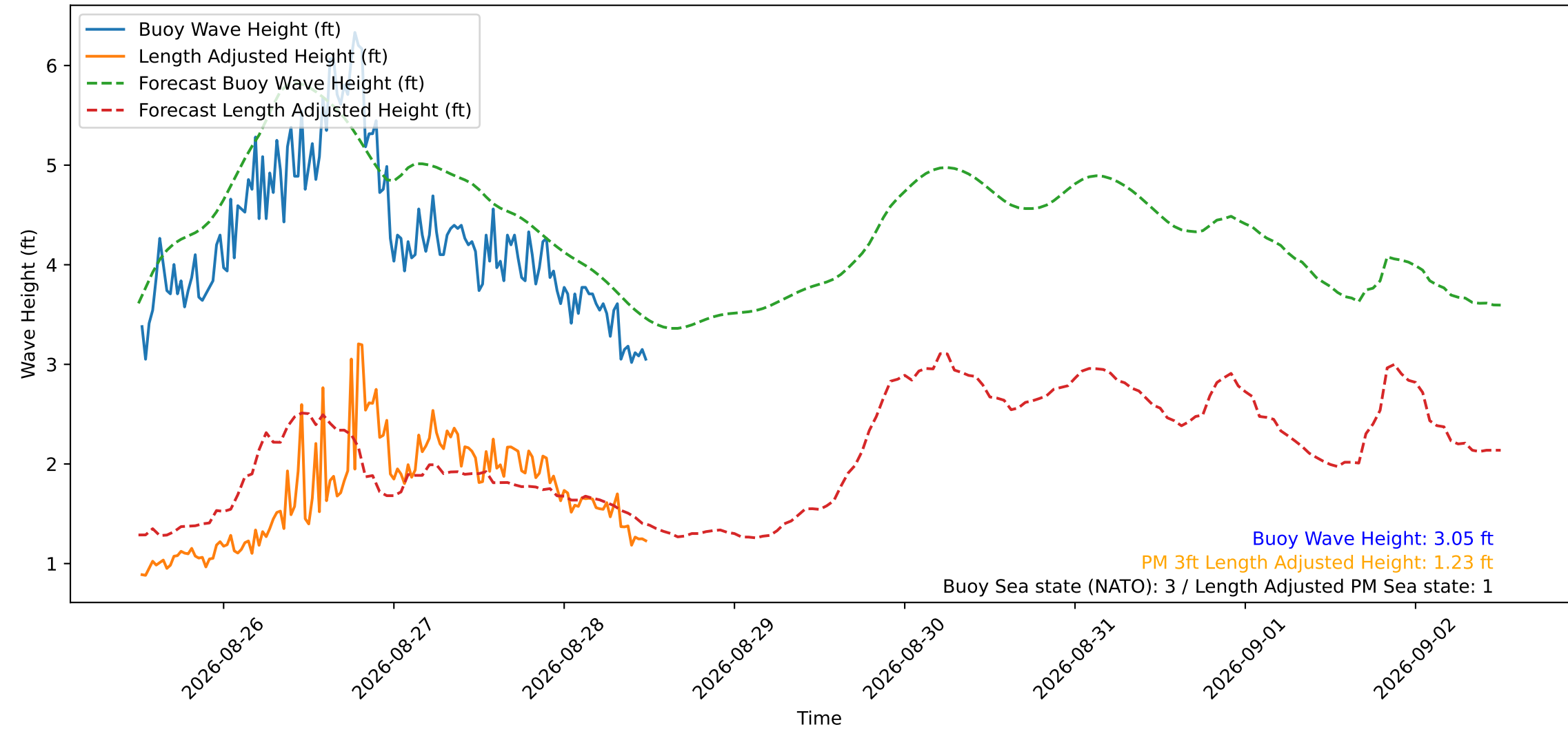
Wave Heights over Time for Green Beach at 2026-08-28 12:11:12
