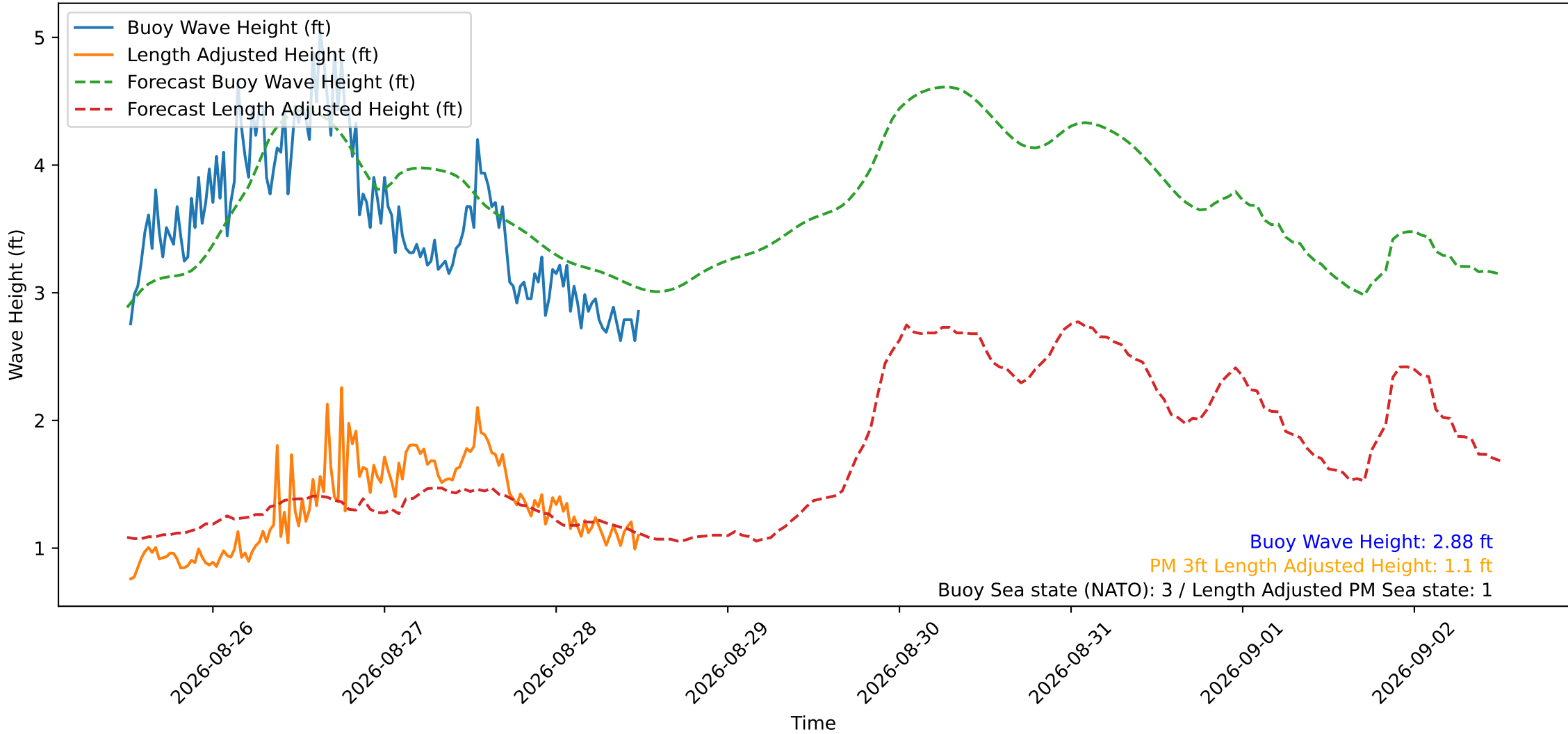
Wave Heights over Time for Red Beach at 2026-08-28 12:10:49
