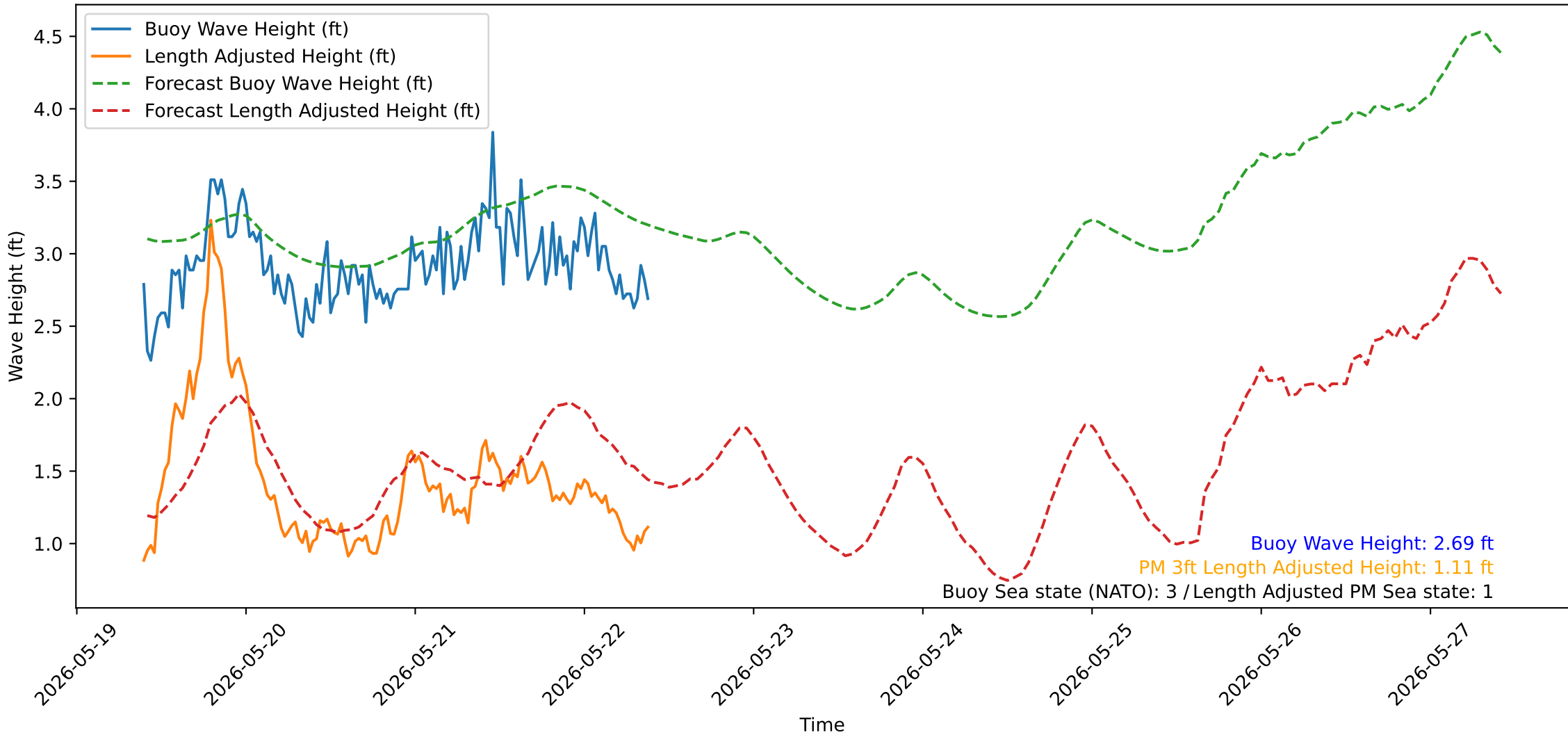
Wave Heights over Time for Oceanside Harbor at 2026-05-22 09:30:32
