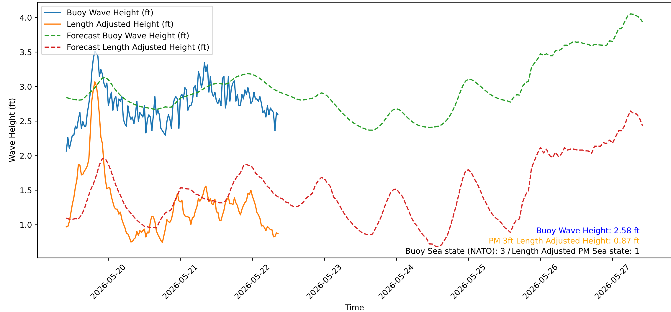
Wave Heights over Time for Red Beach at 2026-05-22 09:30:51
