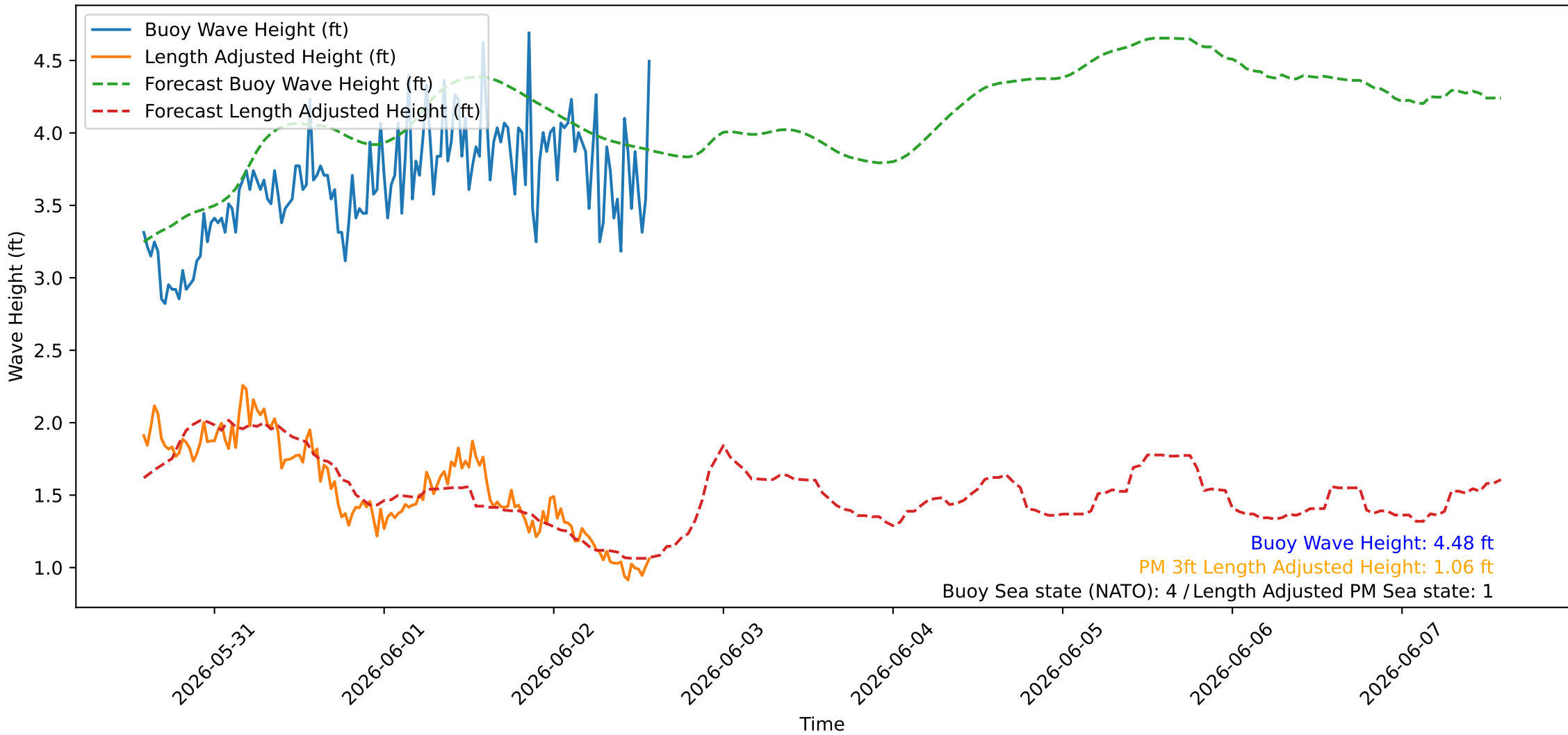
Wave Heights over Time for Oceanside Harbor at 2026-06-02 14:10:26
