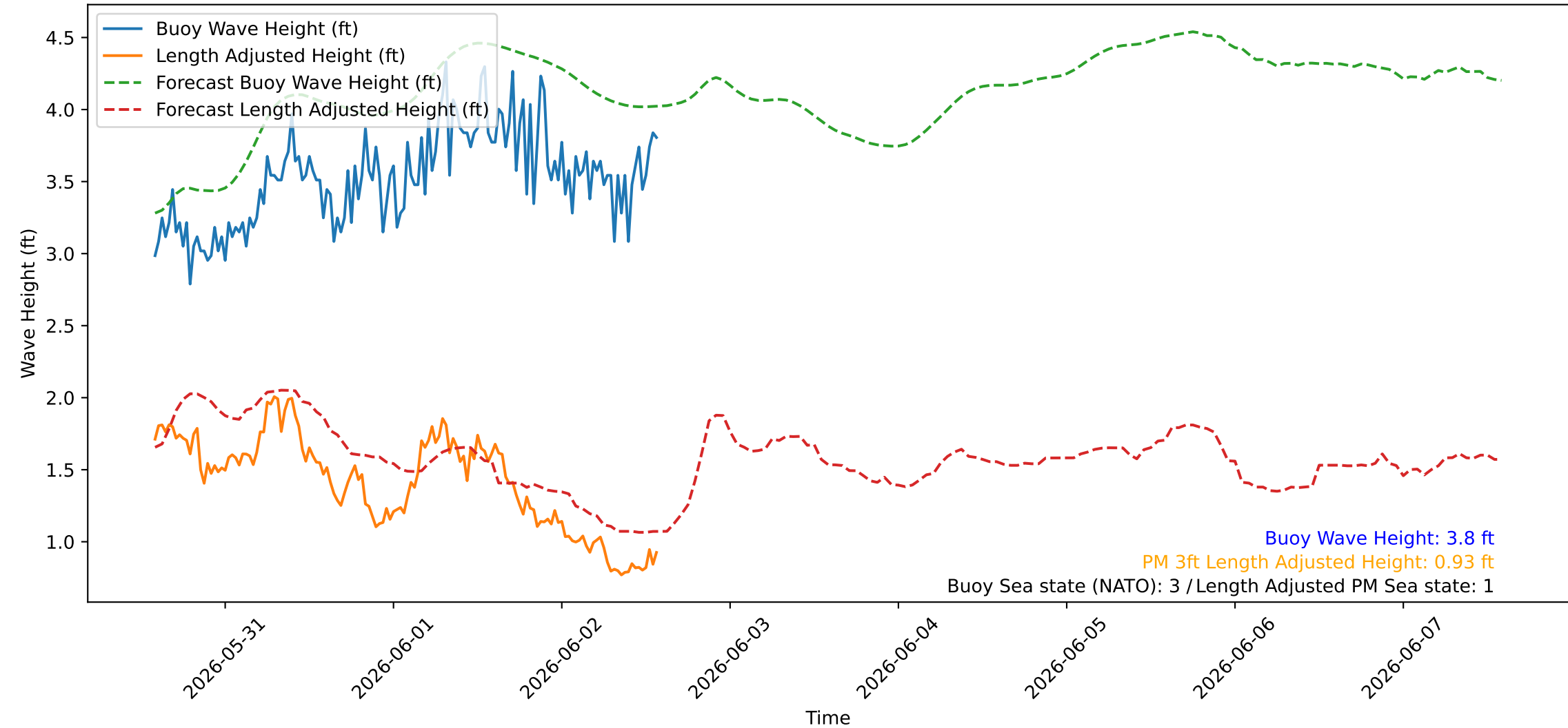
Wave Heights over Time for Green Beach at 2026-06-02 14:11:07
