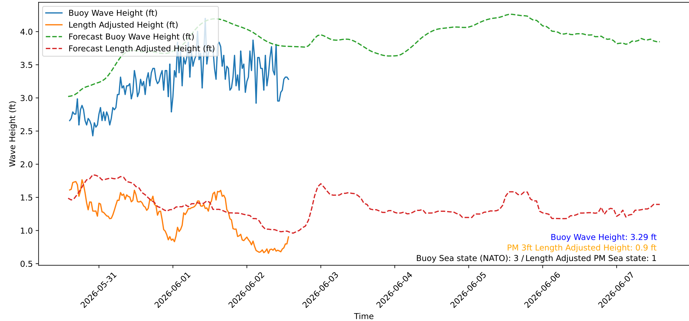
Wave Heights over Time for Red Beach at 2026-06-02 14:10:44
