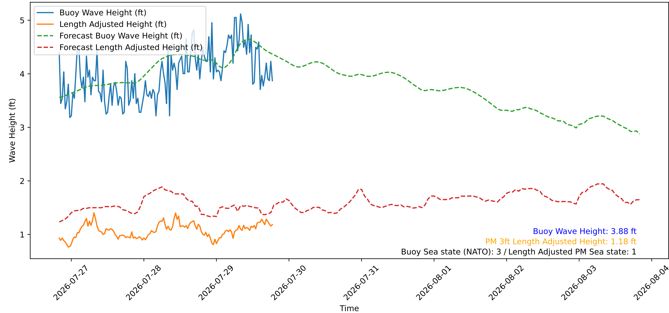
Wave Heights over Time for Red Beach at 2026-07-29 19:30:46
