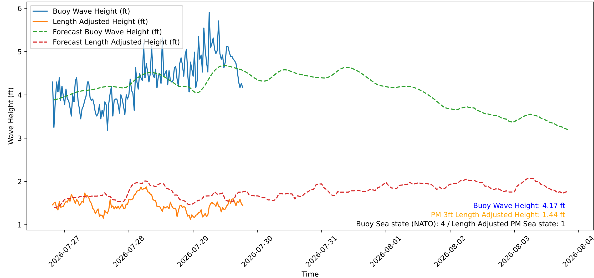
Wave Heights over Time for Oceanside Harbor at 2026-07-29 19:30:26
