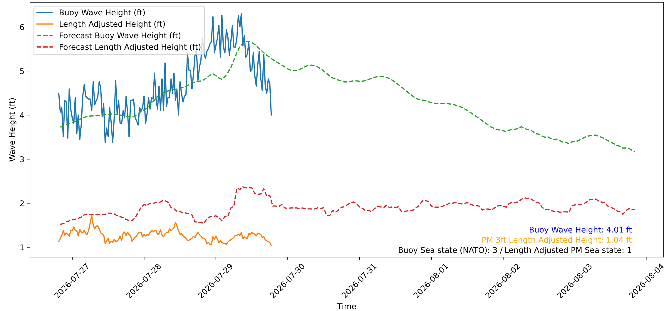
Wave Heights over Time for Green Beach at 2026-07-29 19:31:09
