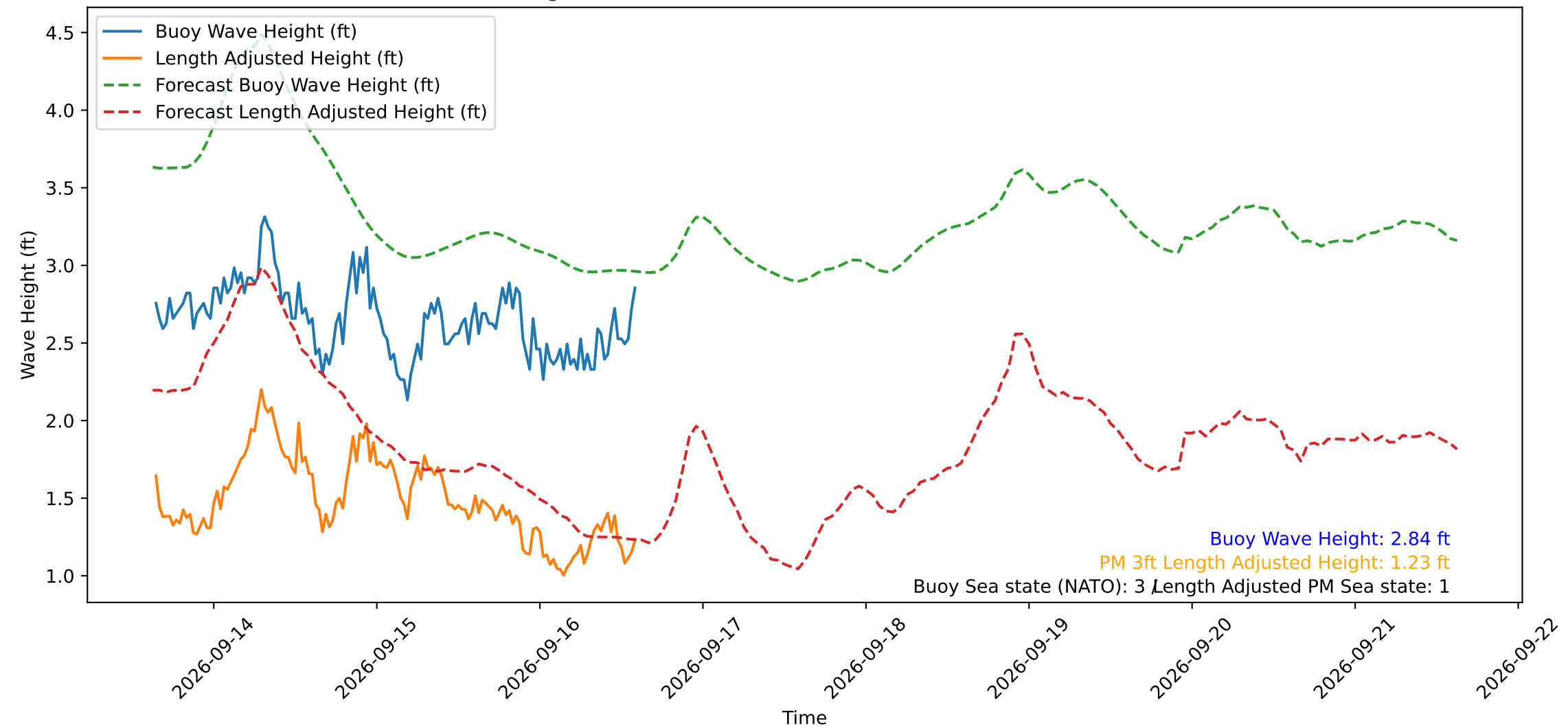
Wave Heights over Time for Green Beach at 2026-09-16 15:01:11
