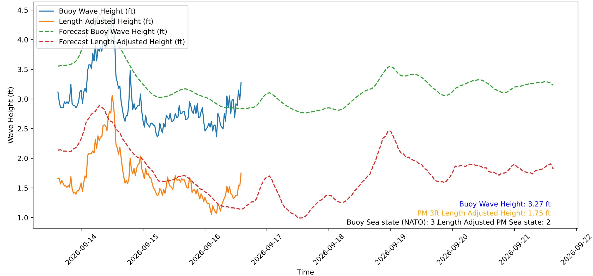
Wave Heights over Time for Oceanside Harbor at 2026-09-16 15:00:29
