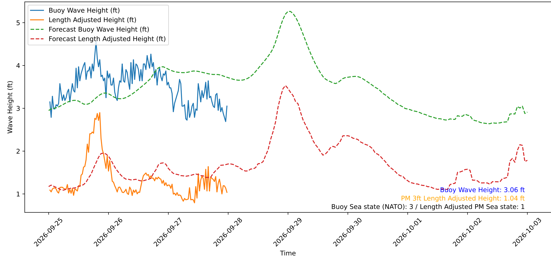
Wave Heights over Time for Green Beach at 2026-09-28 00:11:12
