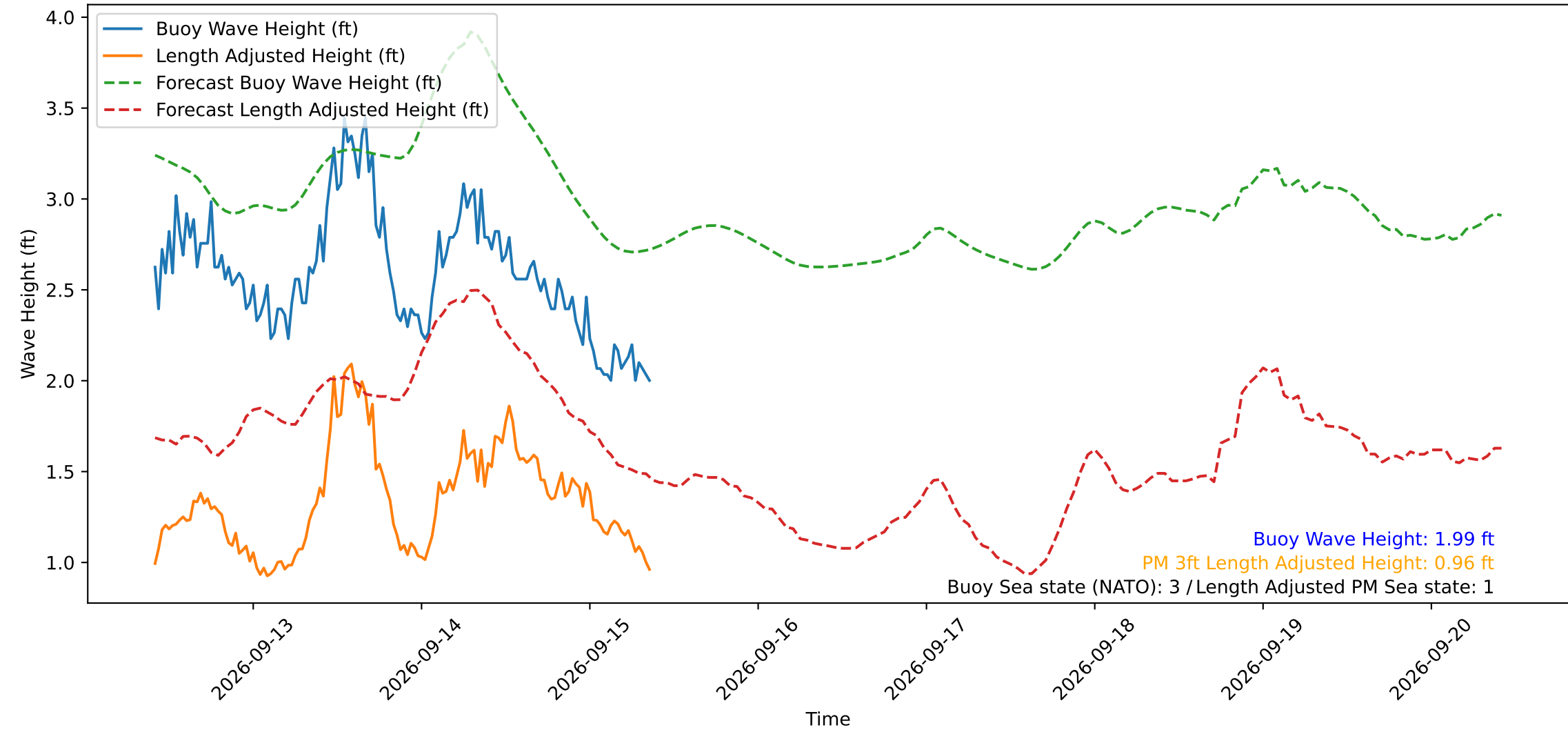
Wave Heights over Time for Red Beach at 2026-09-15 09:30:49
