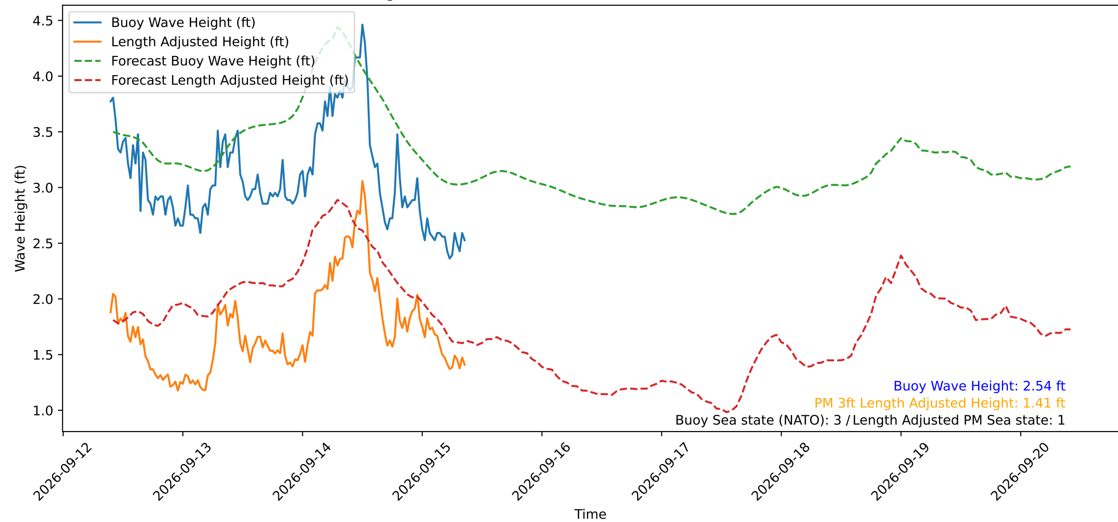
Wave Heights over Time for Oceanside Harbor at 2026-09-15 09:30:30
