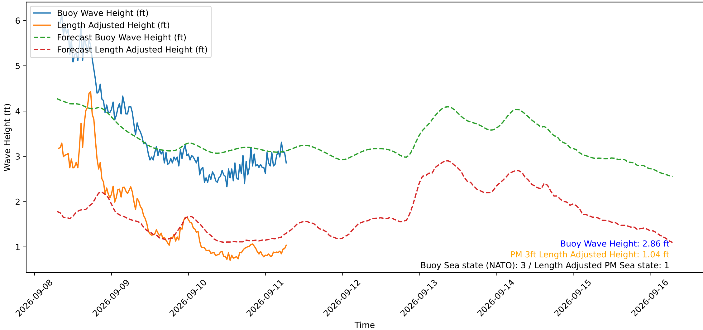
Wave Heights over Time for Red Beach at 2026-09-11 07:20:50
