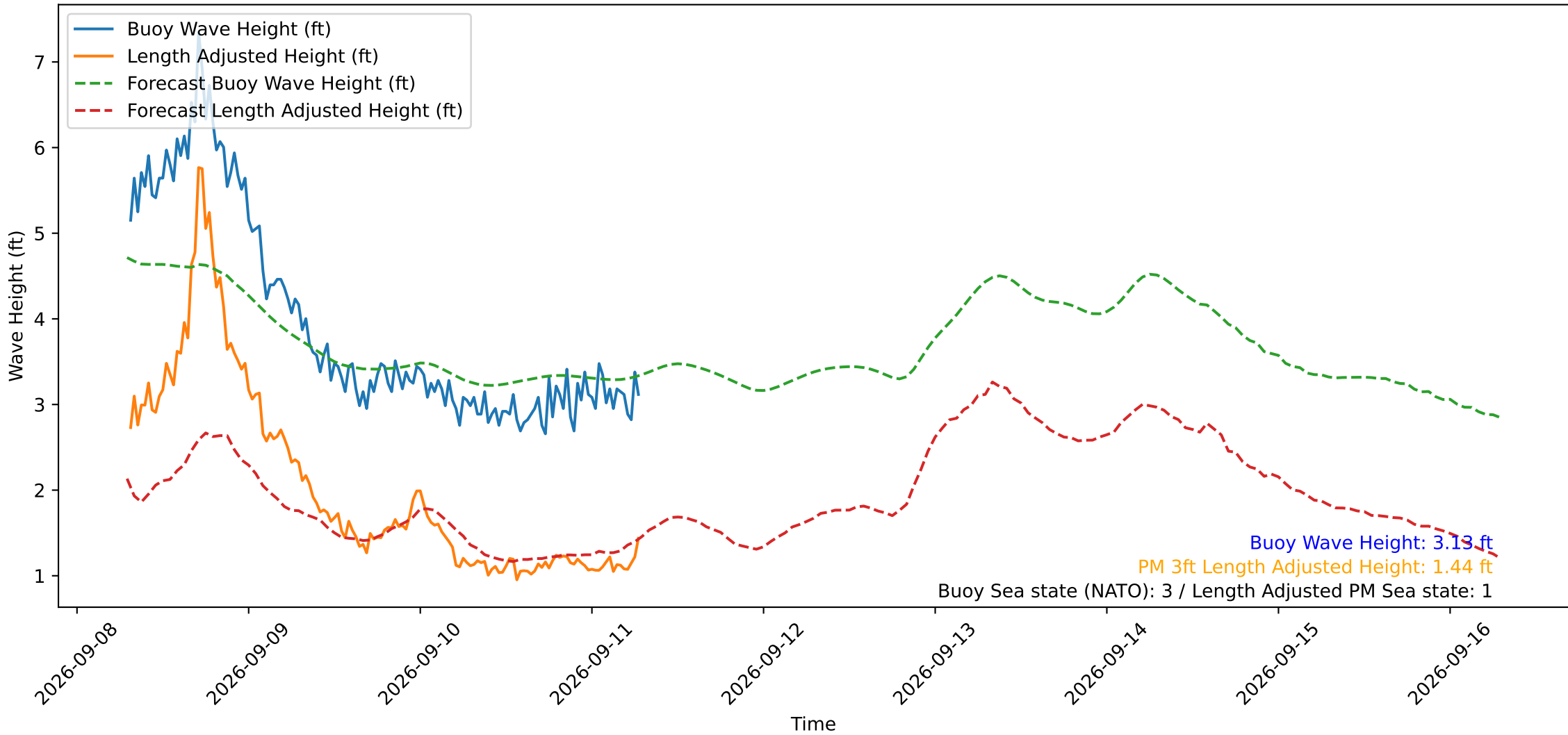
Wave Heights over Time for Oceanside Harbor at 2026-09-11 07:20:30
