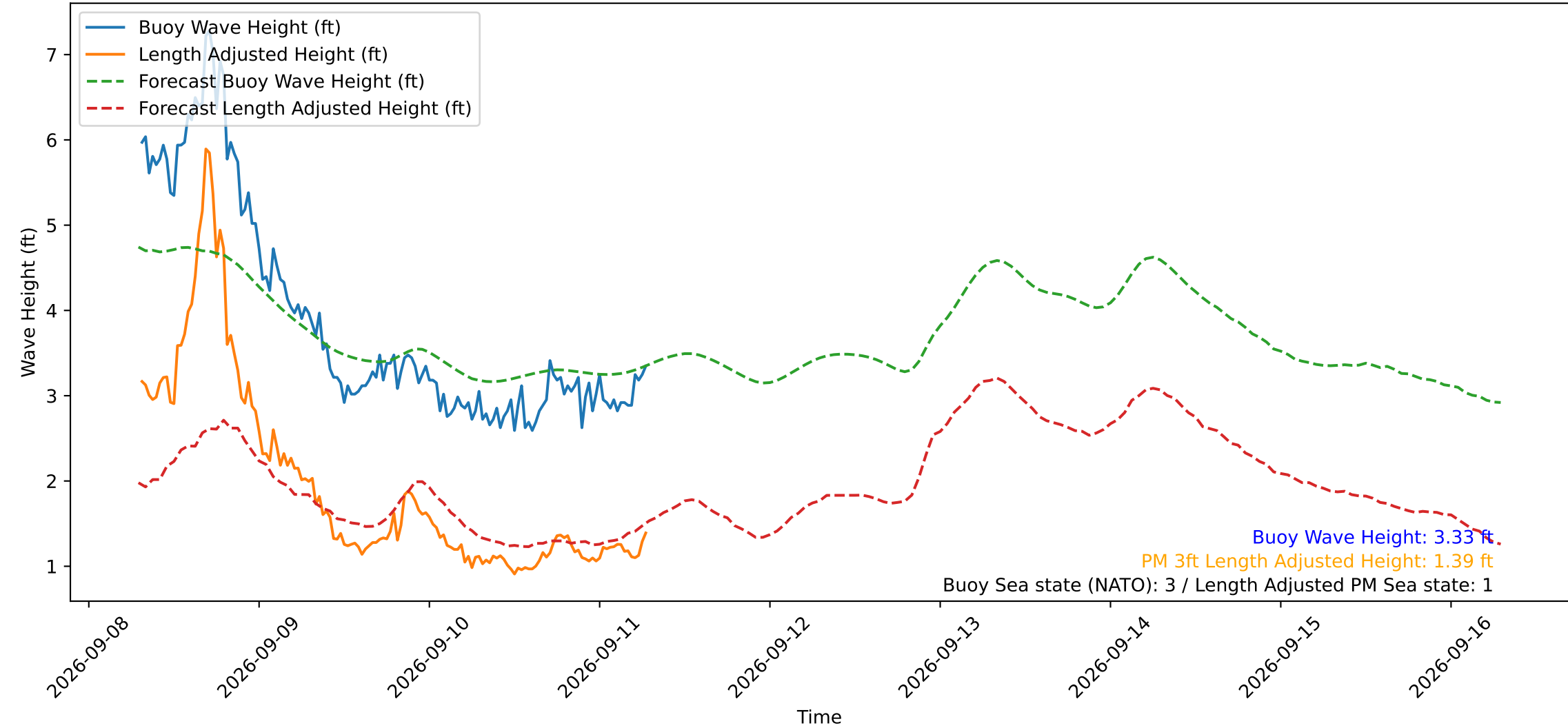
Wave Heights over Time for Green Beach at 2026-09-11 07:21:15
