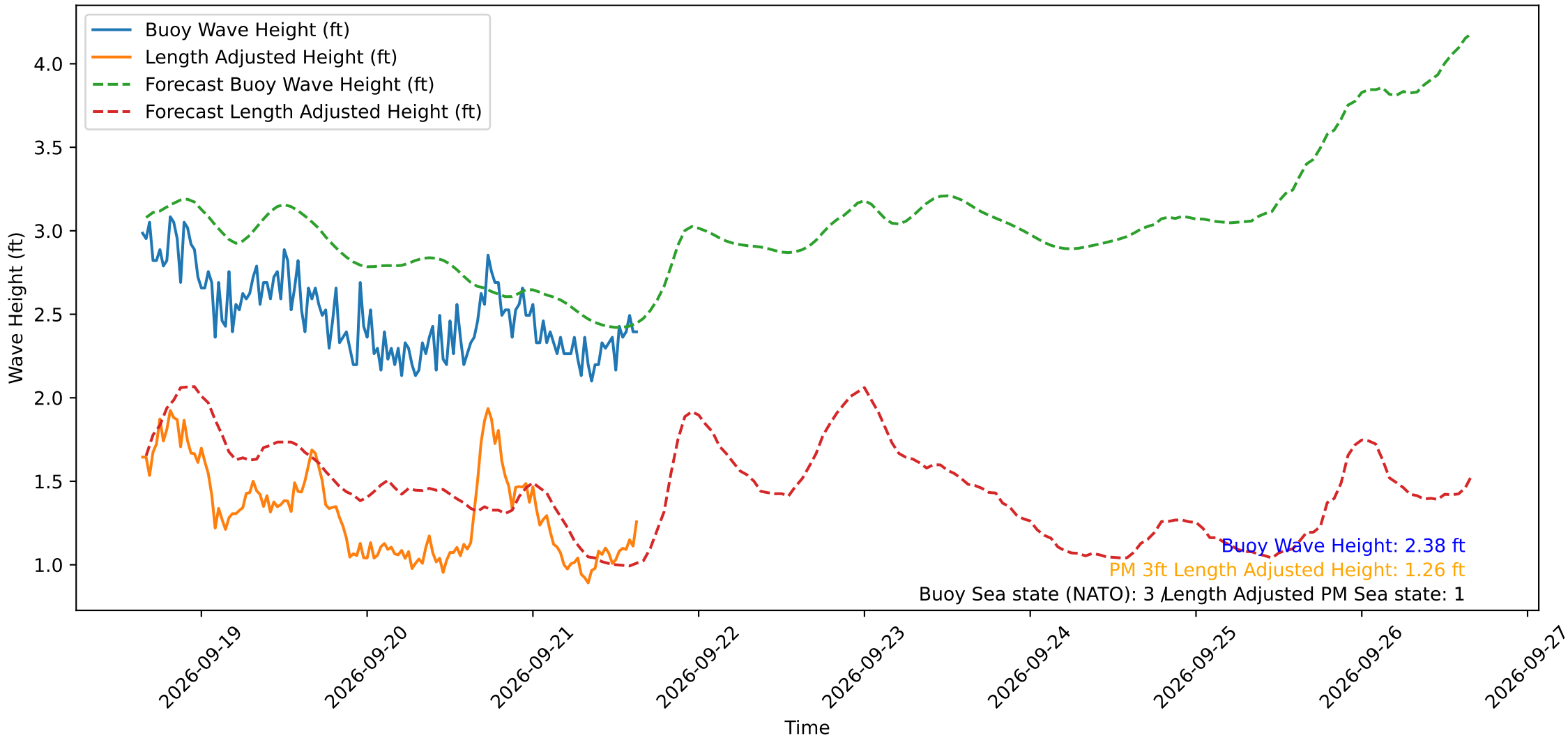
Wave Heights over Time for Oceanside Harbor at 2026-09-21 15:30:29
