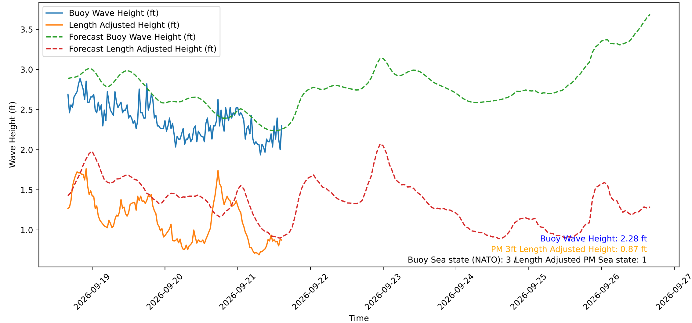
Wave Heights over Time for Red Beach at 2026-09-21 15:30:49
