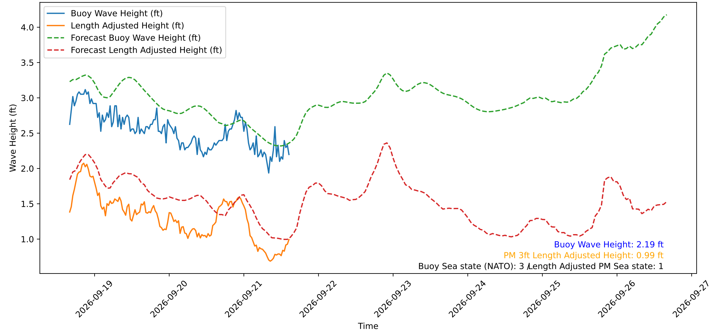
Wave Heights over Time for Green Beach at 2026-09-21 15:31:11
