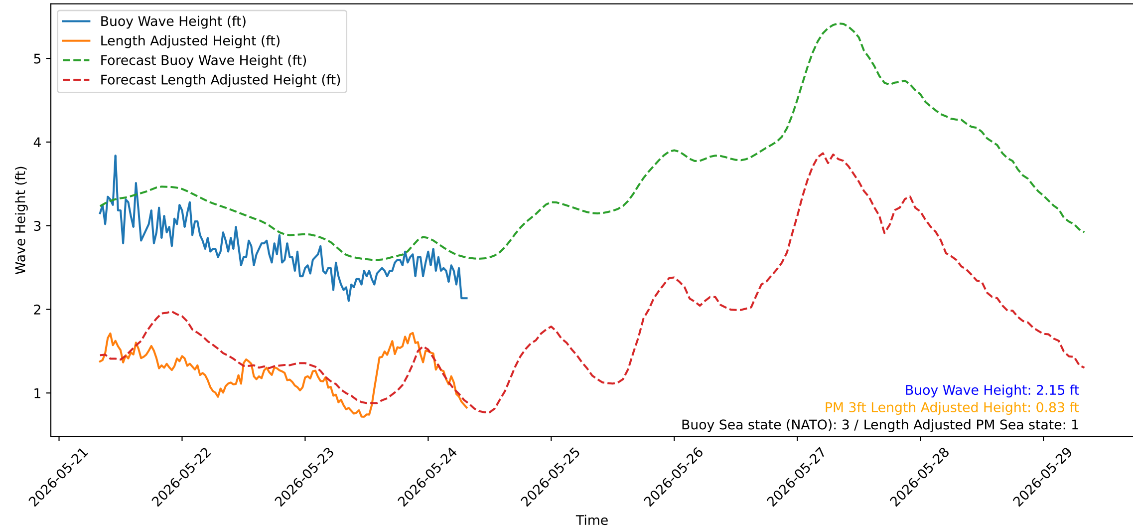
Wave Heights over Time for Oceanside Harbor at 2026-05-24 08:10:32
