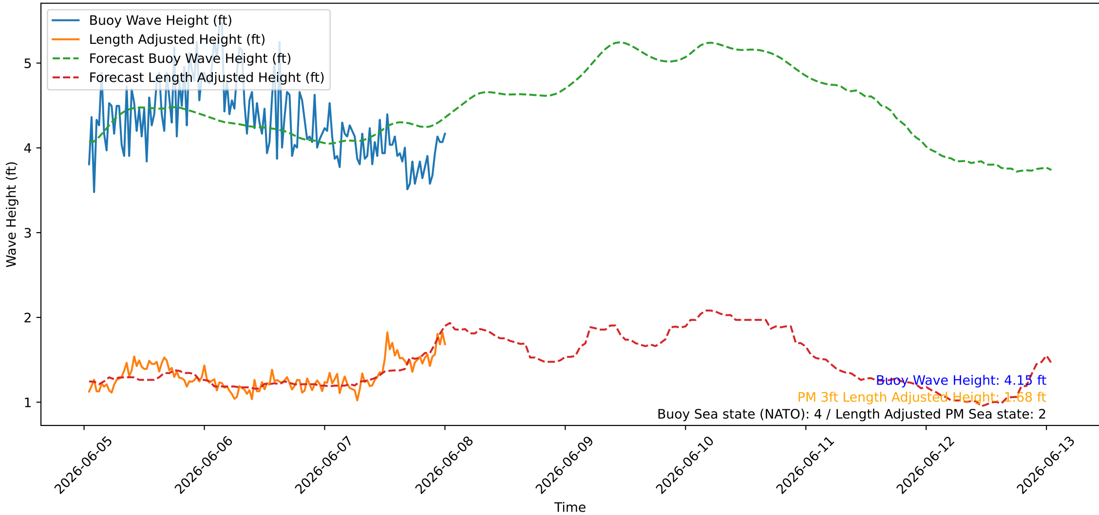
Wave Heights over Time for Oceanside Harbor at 2026-06-08 01:00:26
