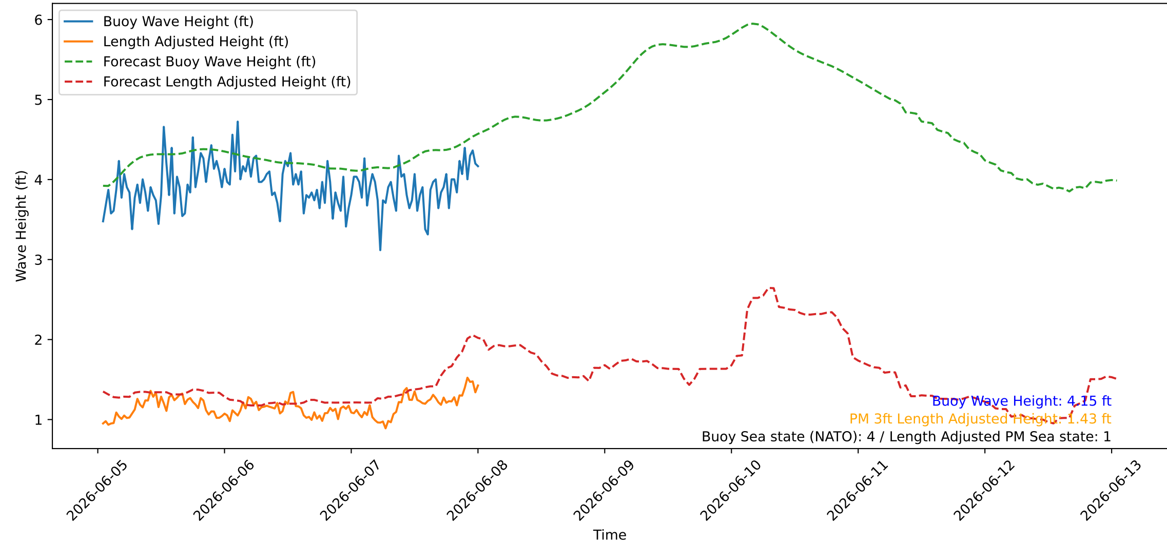
Wave Heights over Time for Green Beach at 2026-06-08 01:01:08
