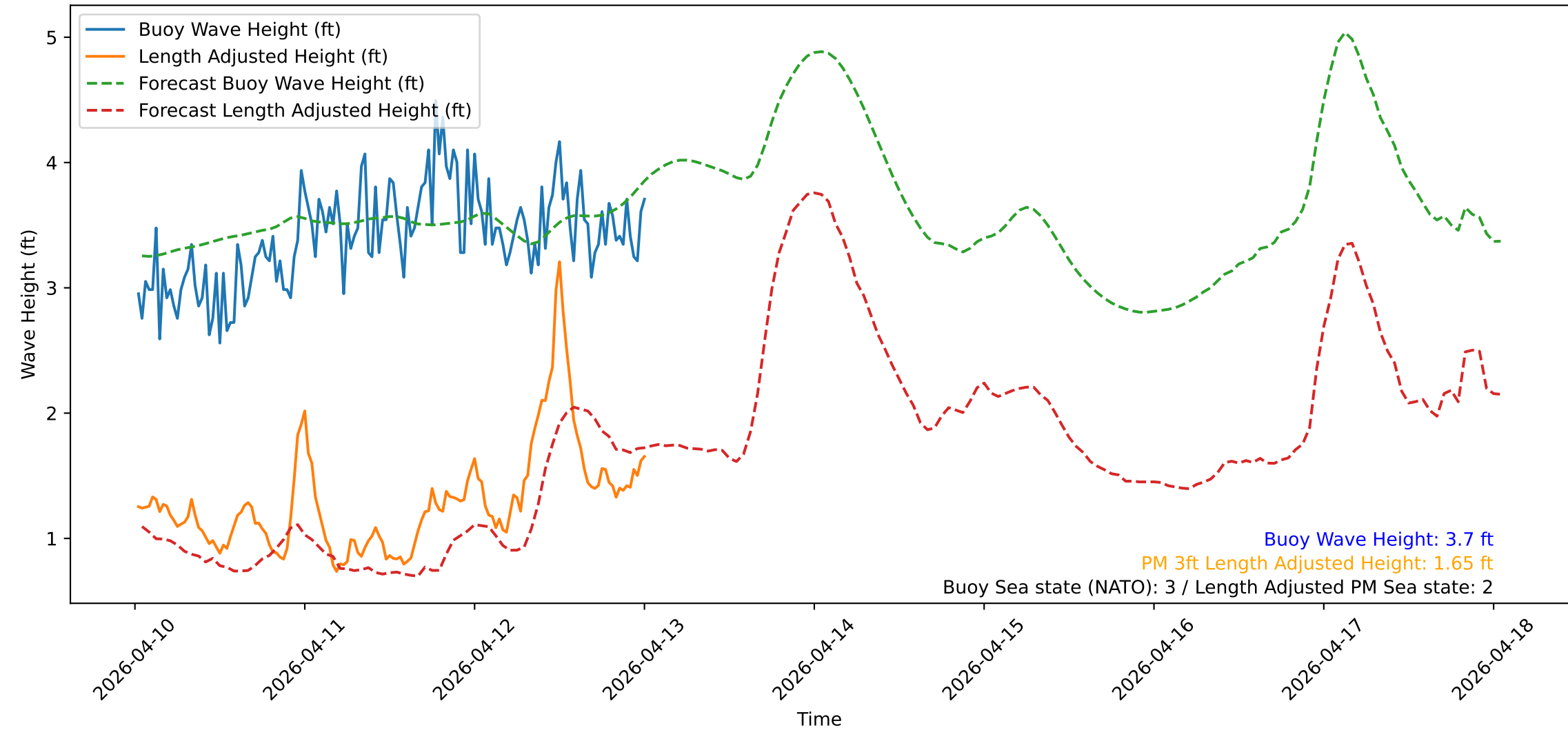
Wave Heights over Time for Green Beach at 2026-04-13 00:41:13
