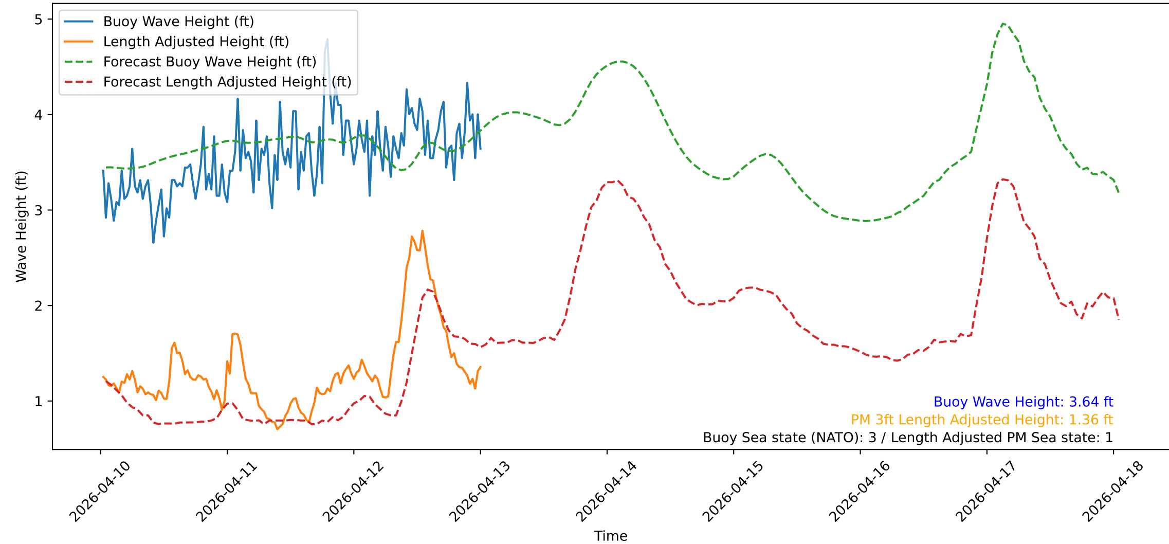
Wave Heights over Time for Oceanside Harbor at 2026-04-13 00:40:31
