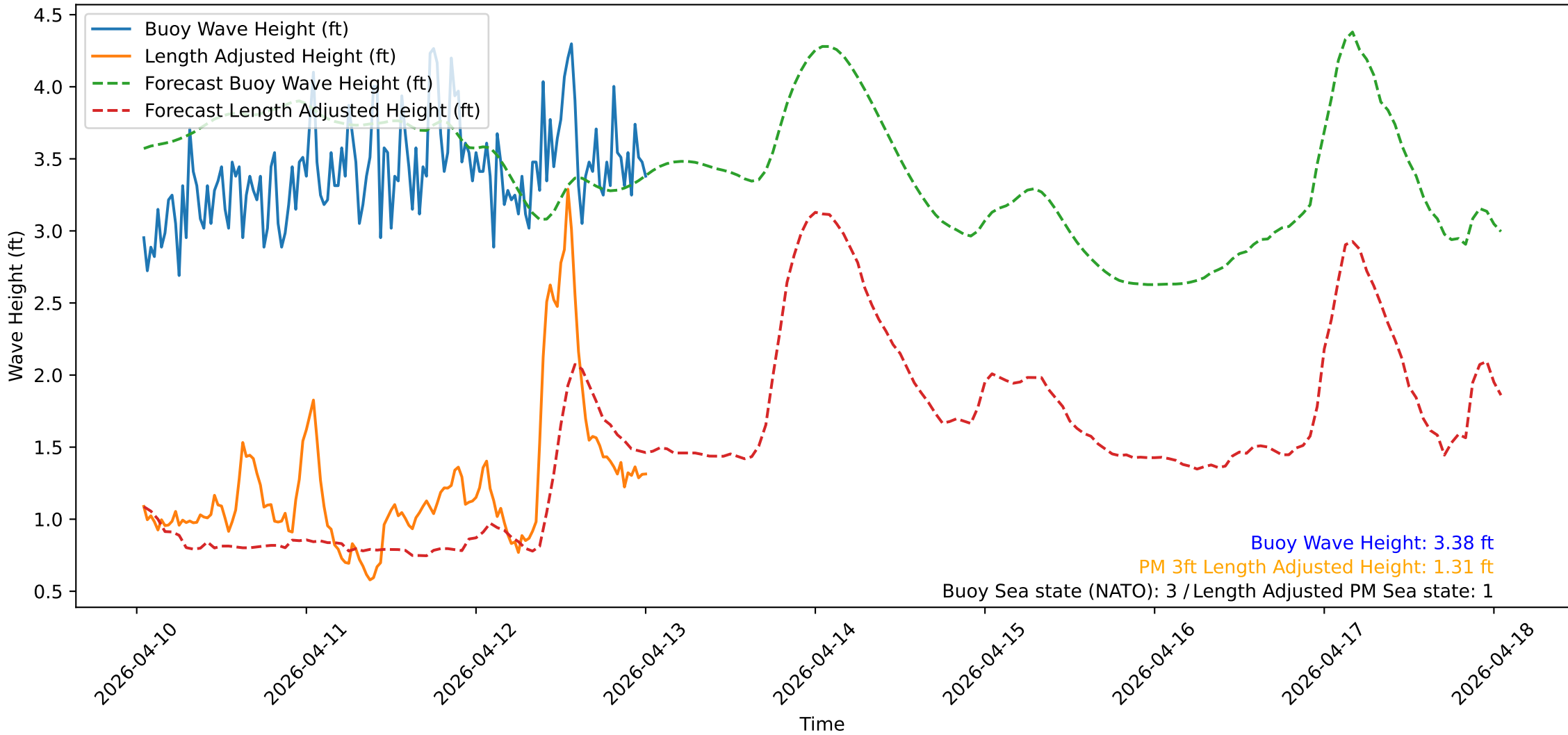
Wave Heights over Time for Red Beach at 2026-04-13 00:40:50
