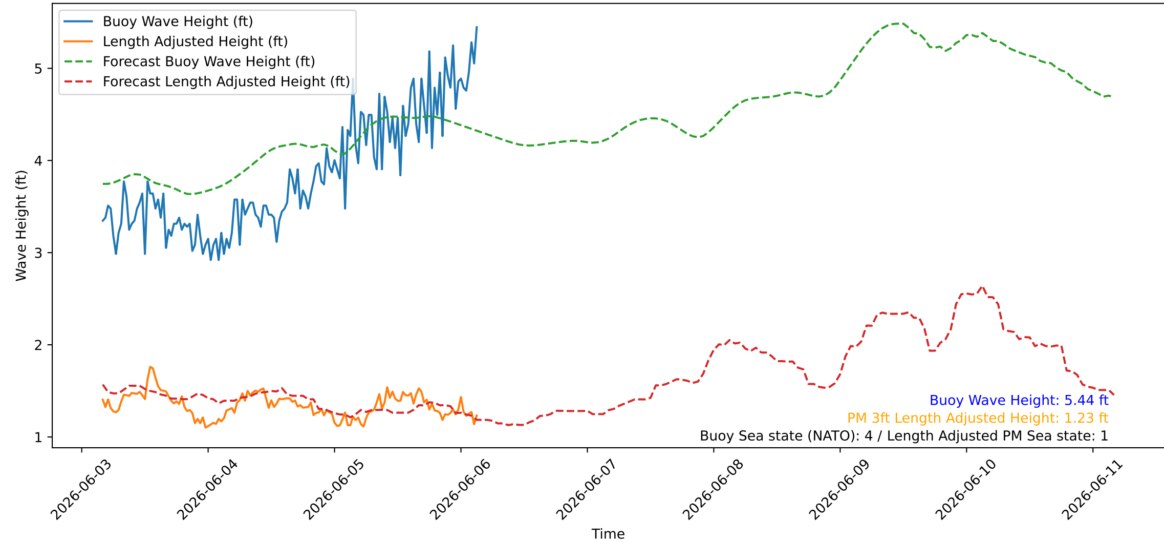
Wave Heights over Time for Oceanside Harbor at 2026-06-06 03:50:26
