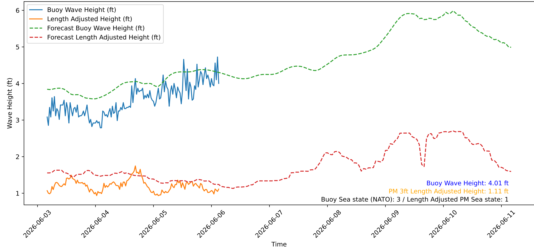
Wave Heights over Time for Green Beach at 2026-06-06 03:51:09
