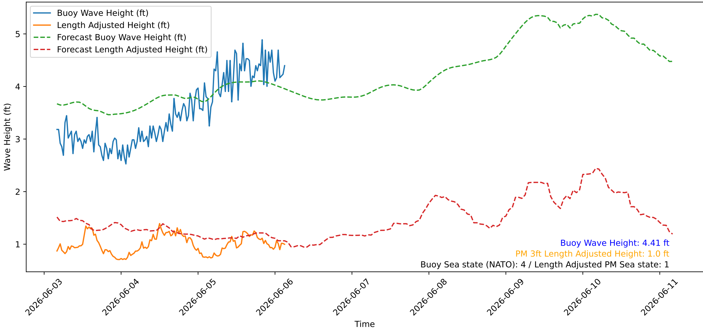
Wave Heights over Time for Red Beach at 2026-06-06 03:50:46
