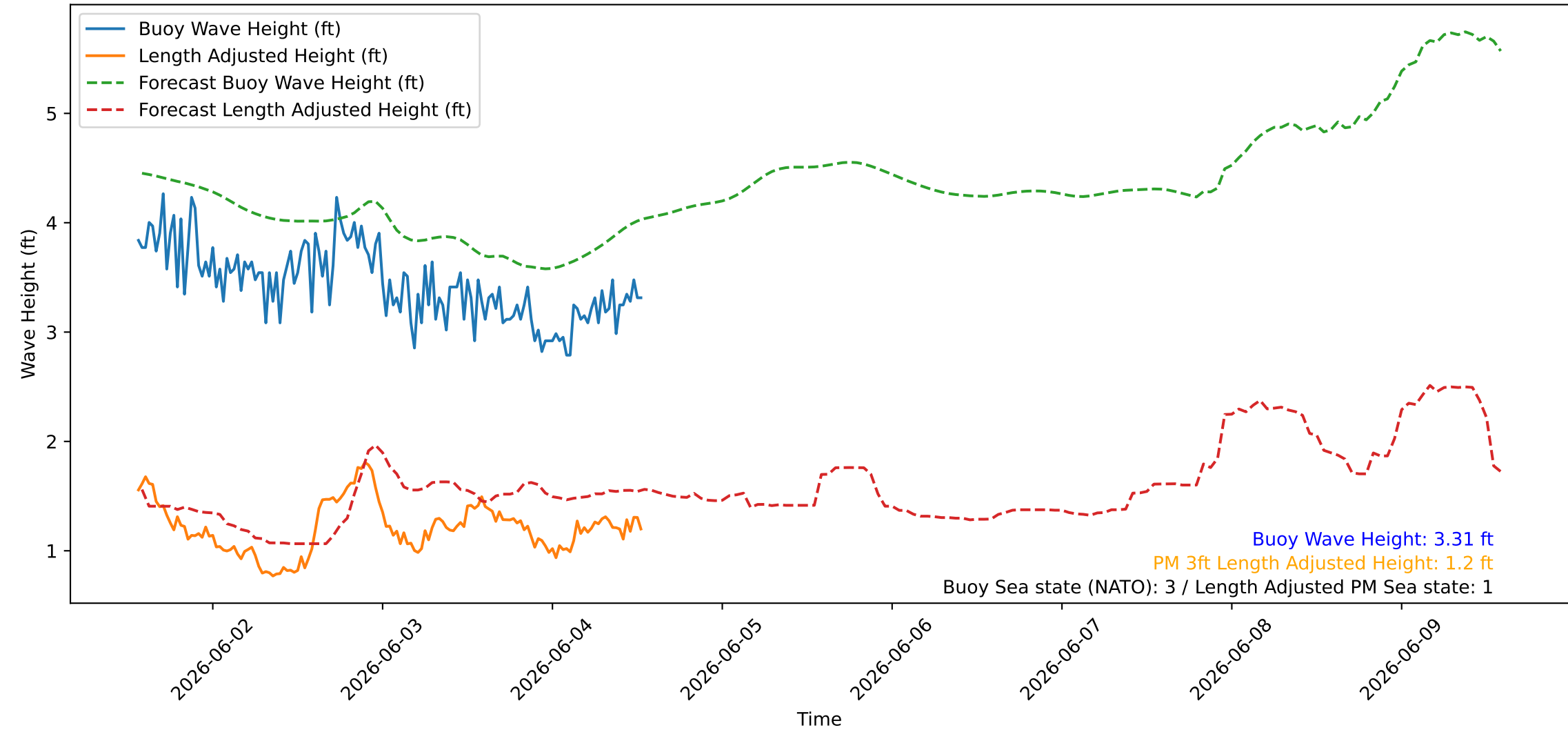
Wave Heights over Time for Green Beach at 2026-06-04 13:31:08
