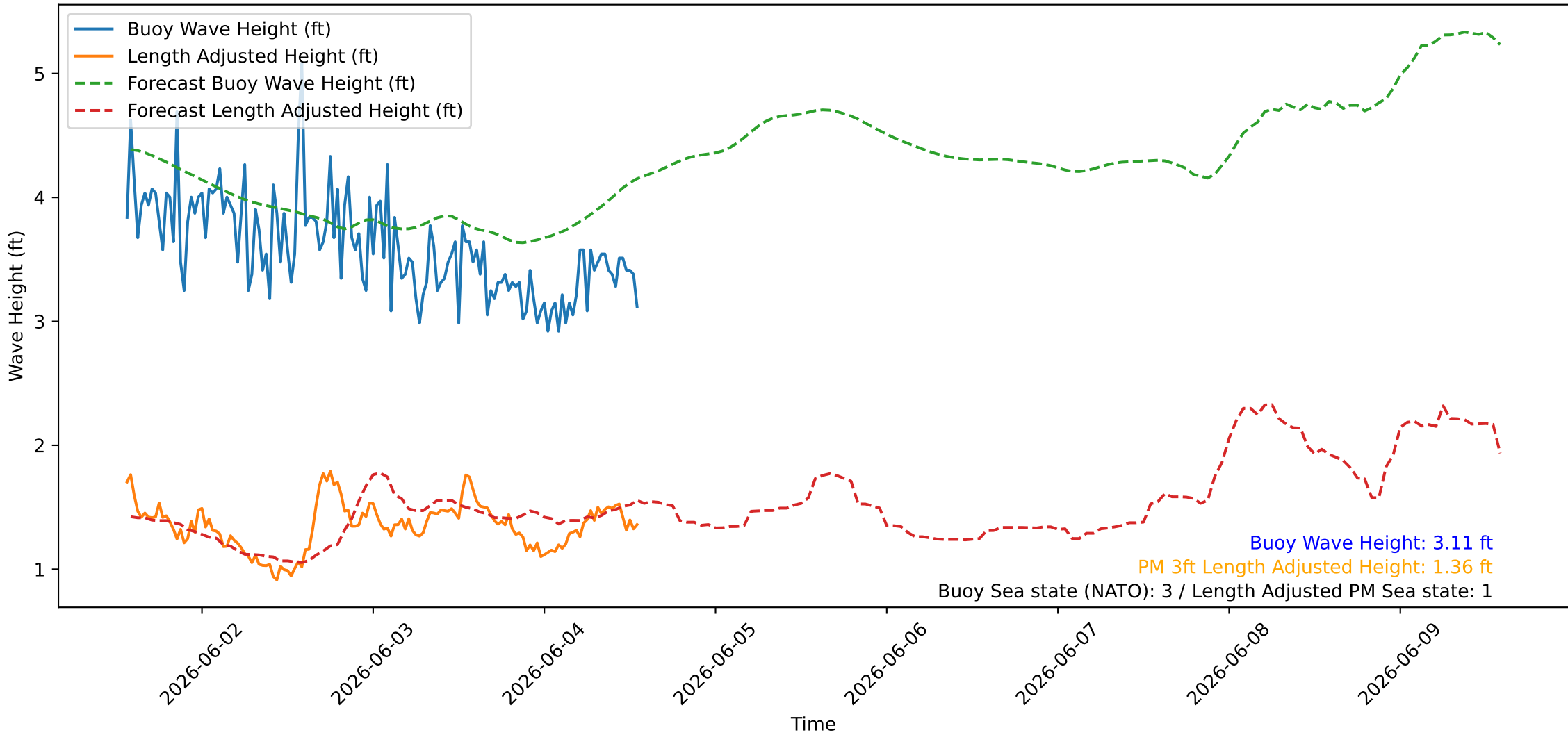
Wave Heights over Time for Oceanside Harbor at 2026-06-04 13:30:26
