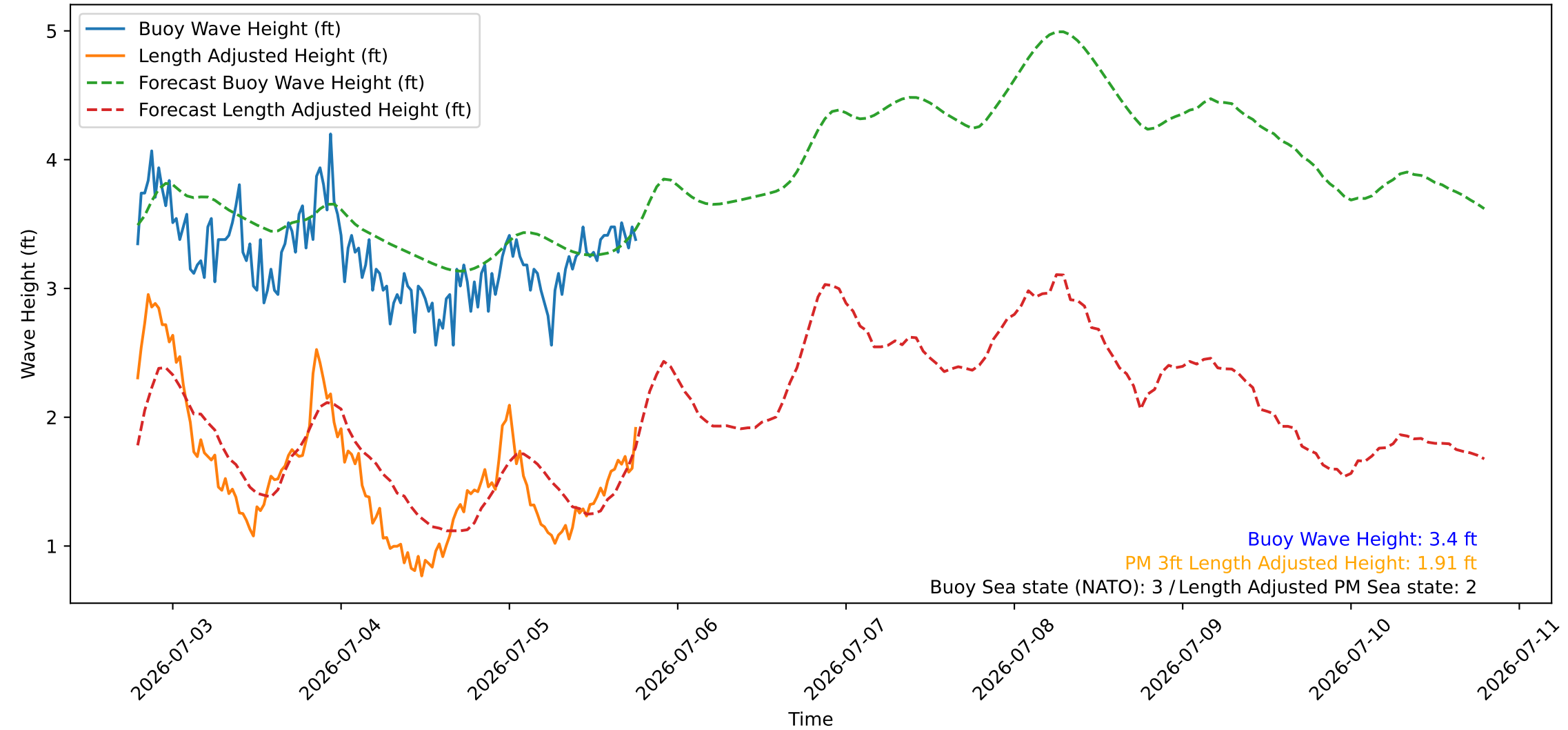
Wave Heights over Time for Green Beach at 2026-07-05 19:01:08
