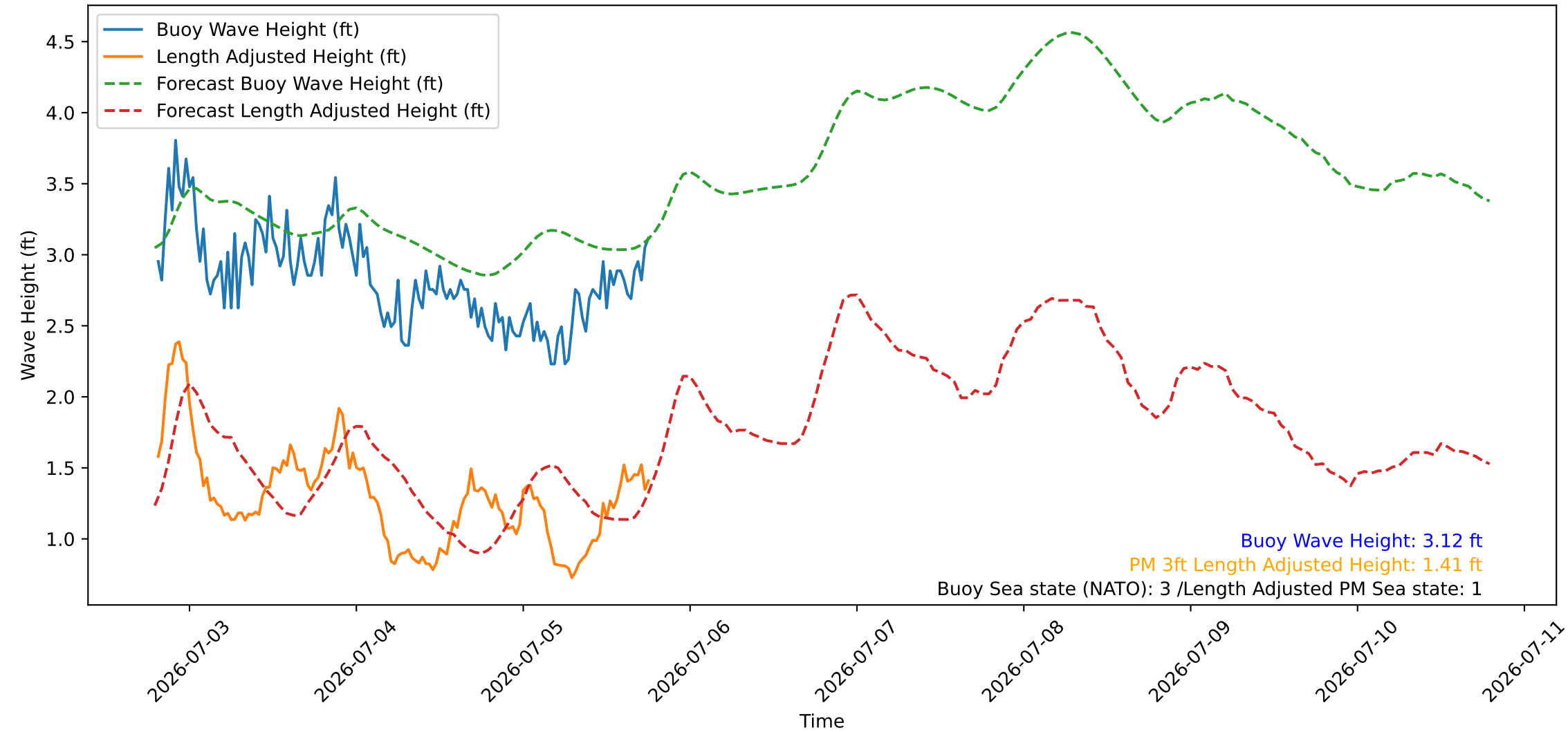
Wave Heights over Time for Red Beach at 2026-07-05 19:00:46
