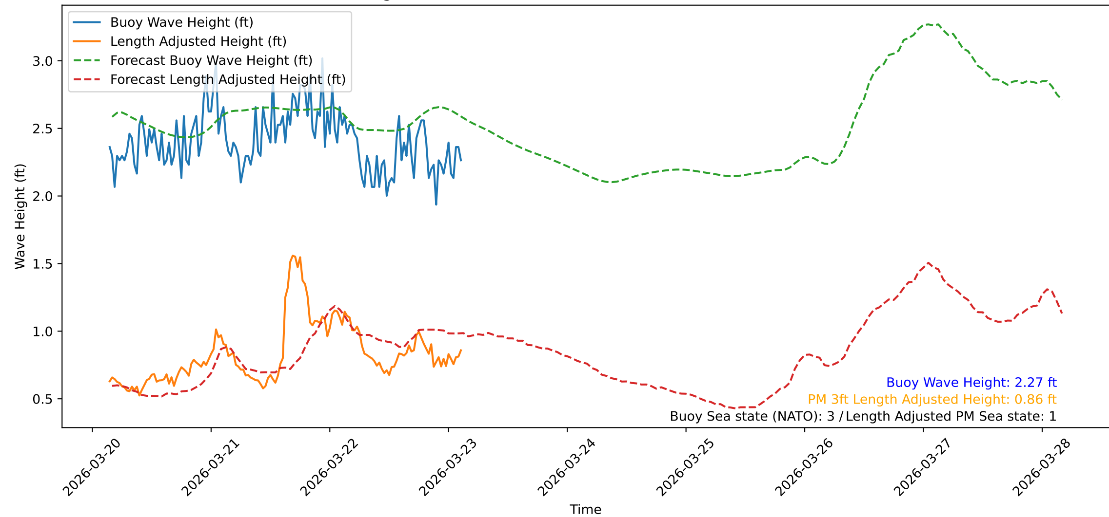
Wave Heights over Time for Oceanside Harbor at 2026-03-23 03:40:32
