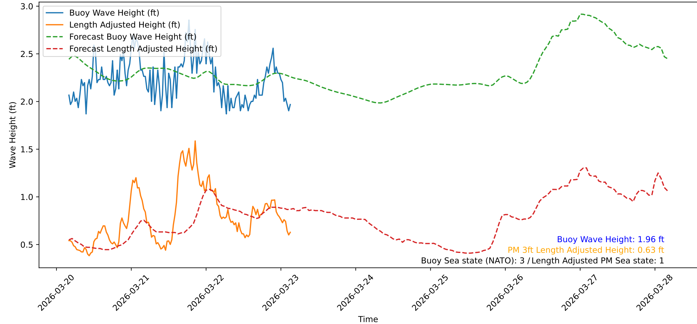
Wave Heights over Time for Red Beach at 2026-03-23 03:40:48
