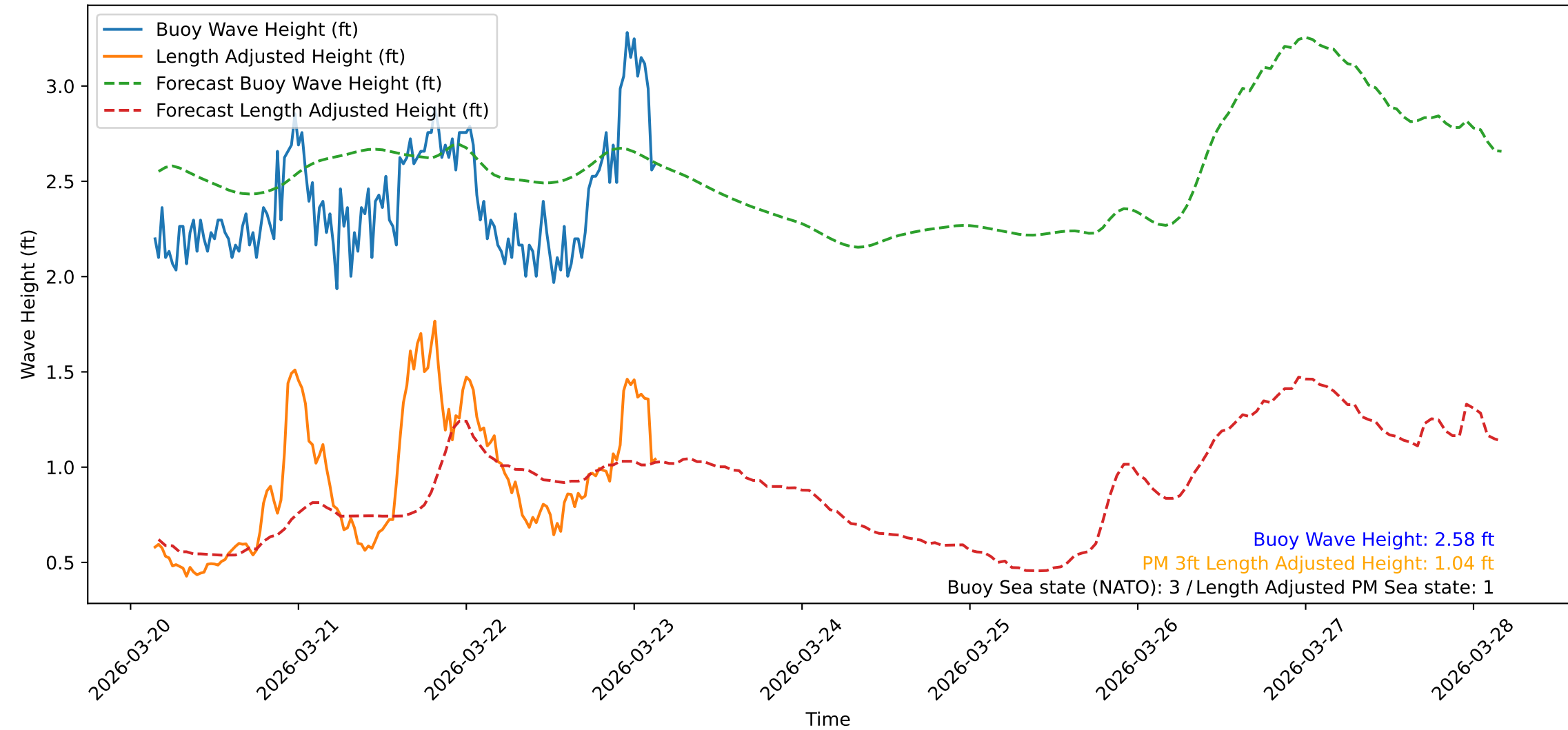
Wave Heights over Time for Green Beach at 2026-03-23 03:41:11
