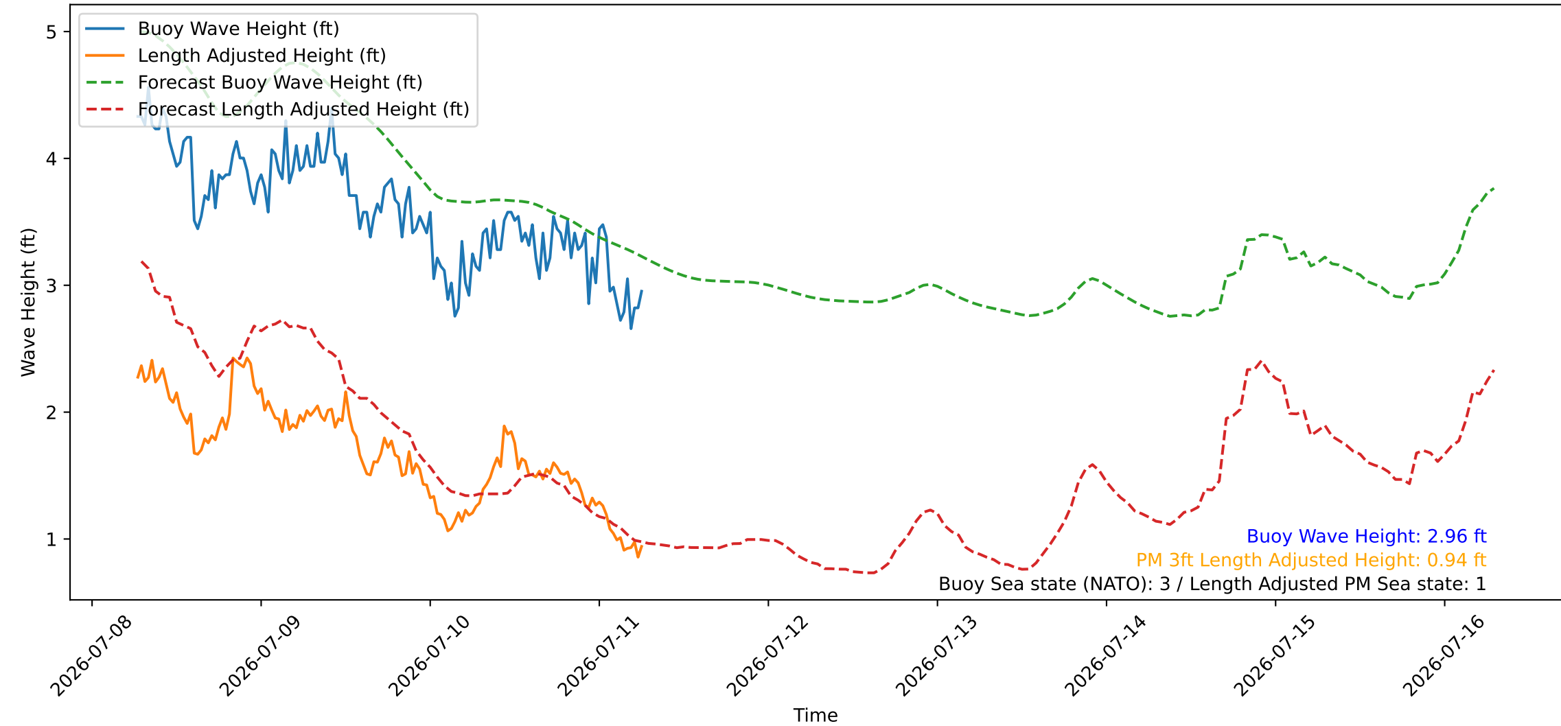
Wave Heights over Time for Green Beach at 2026-07-11 06:41:08
