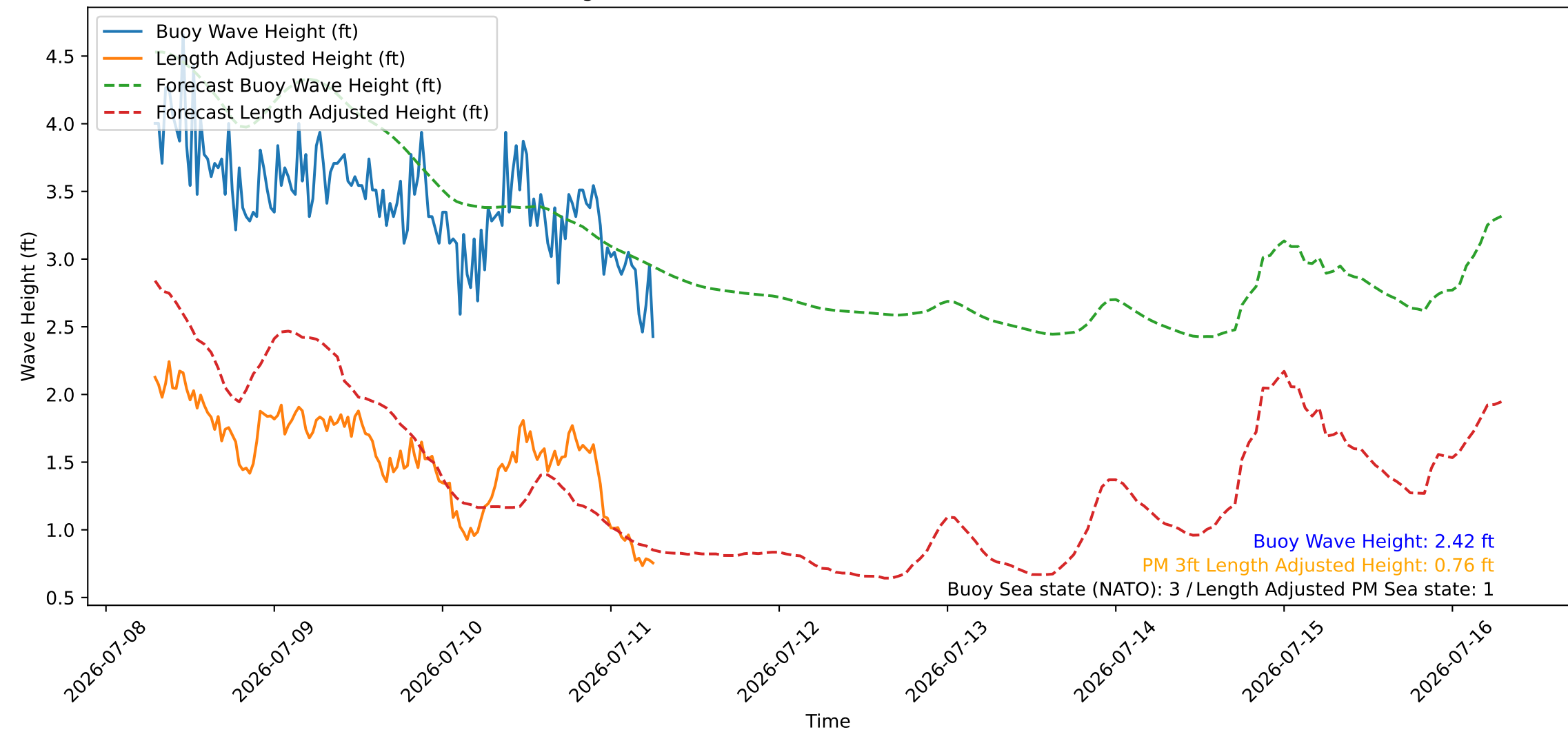
Wave Heights over Time for Red Beach at 2026-07-11 06:40:46
