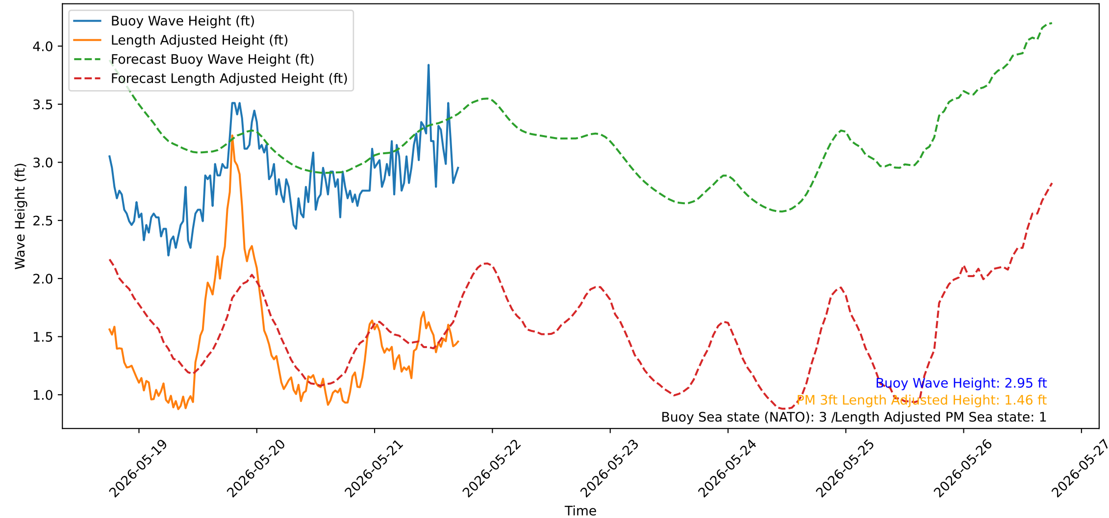
Wave Heights over Time for Oceanside Harbor at 2026-05-21 17:50:32
