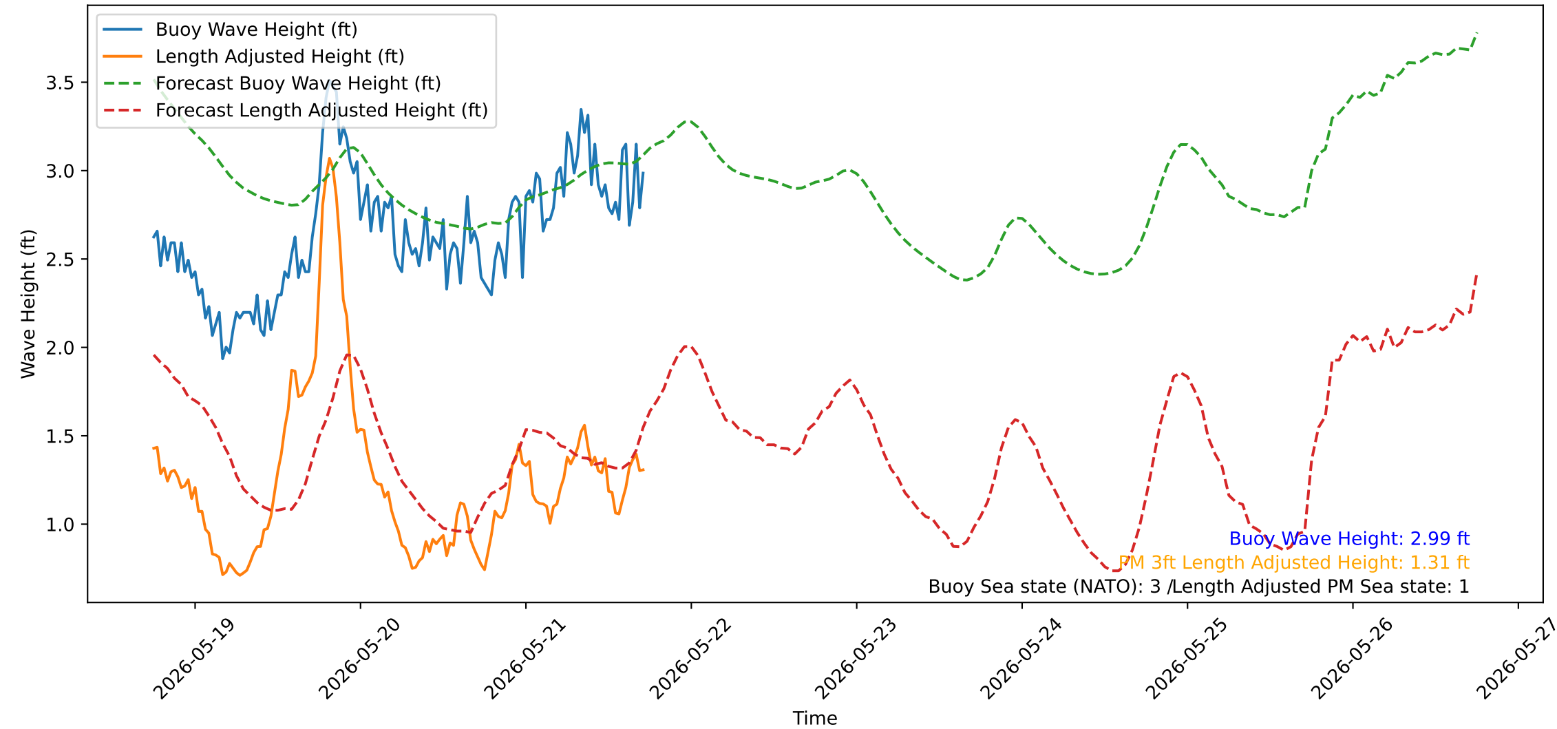
Wave Heights over Time for Red Beach at 2026-05-21 17:50:52
