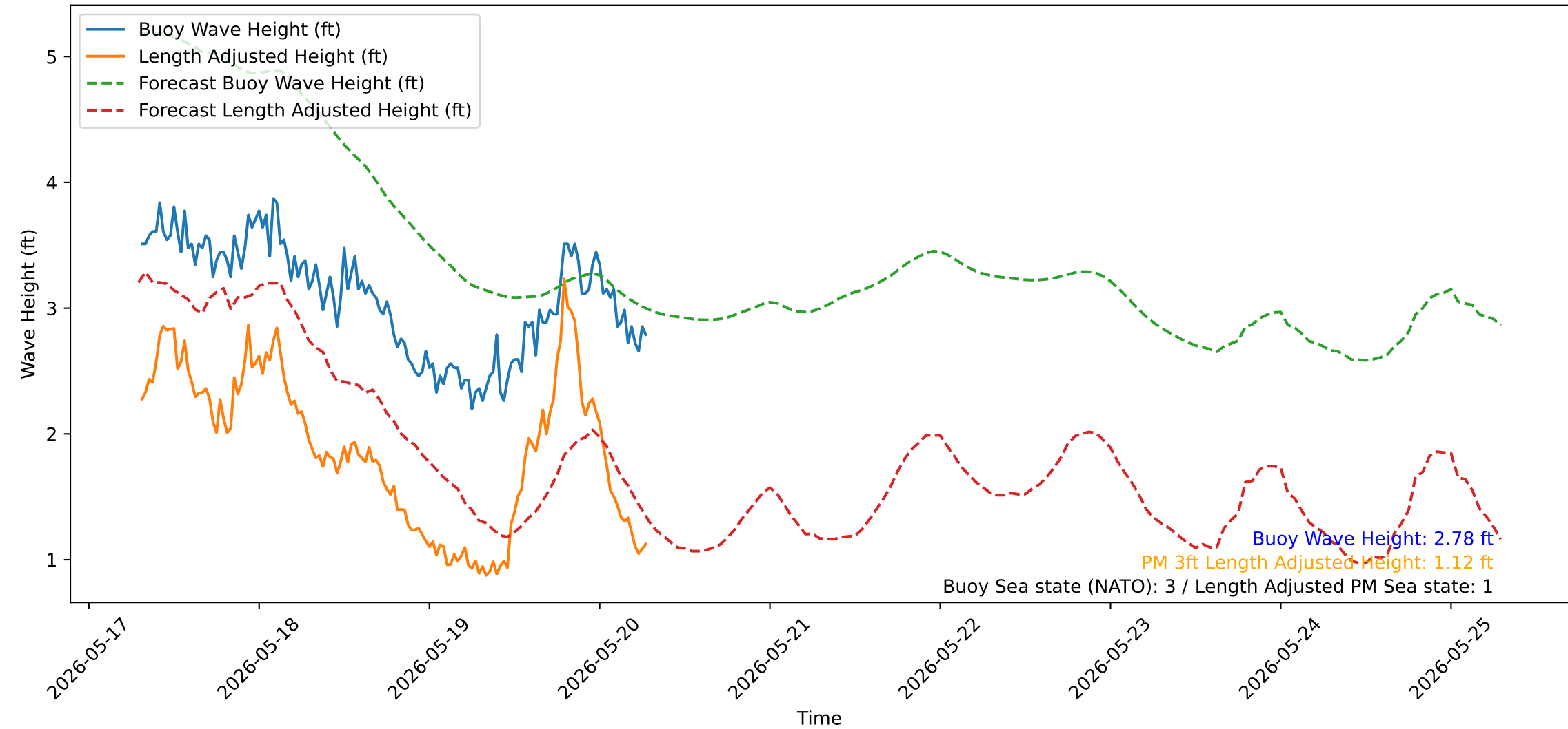
Wave Heights over Time for Oceanside Harbor at 2026-05-20 07:20:32
