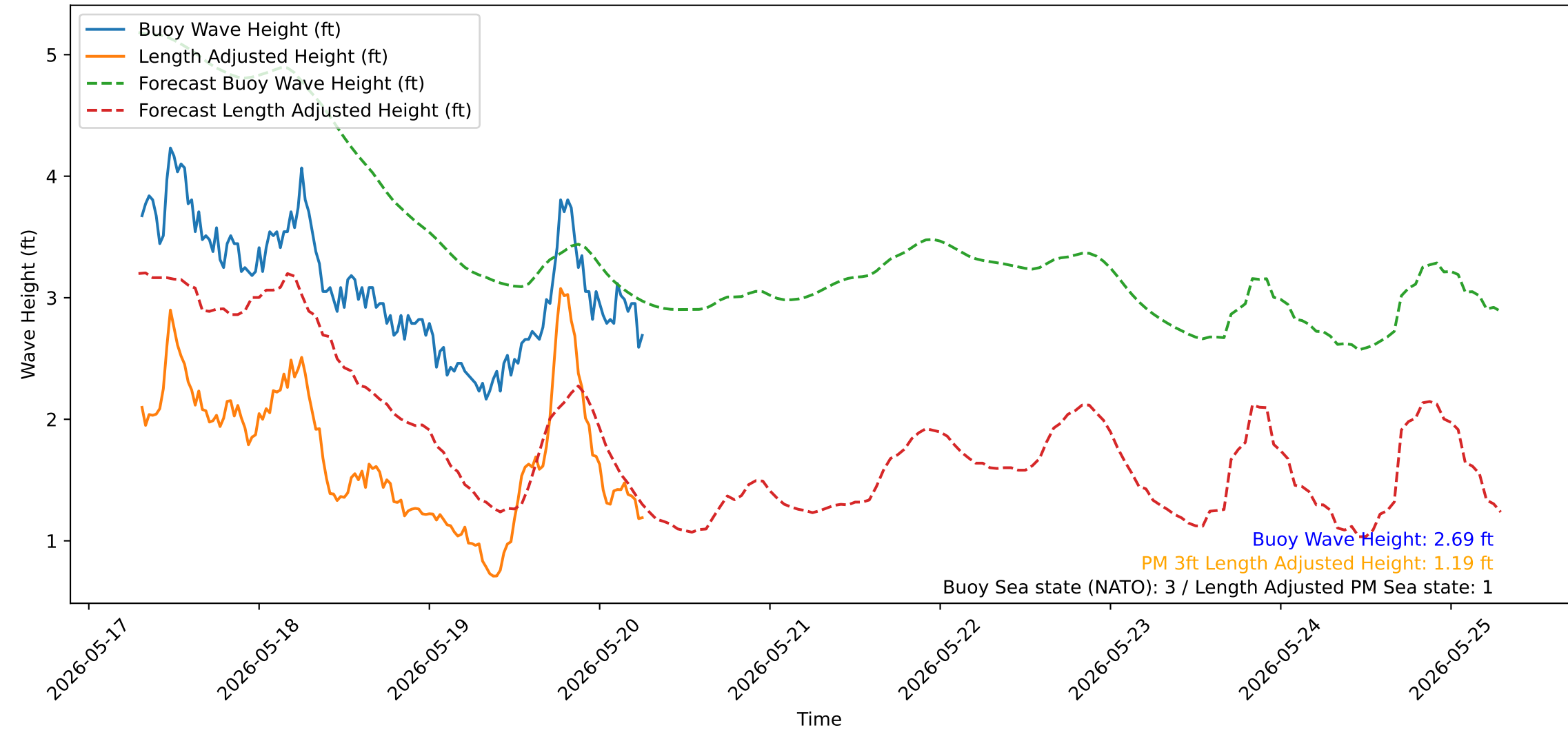
Wave Heights over Time for Green Beach at 2026-05-20 07:21:15
