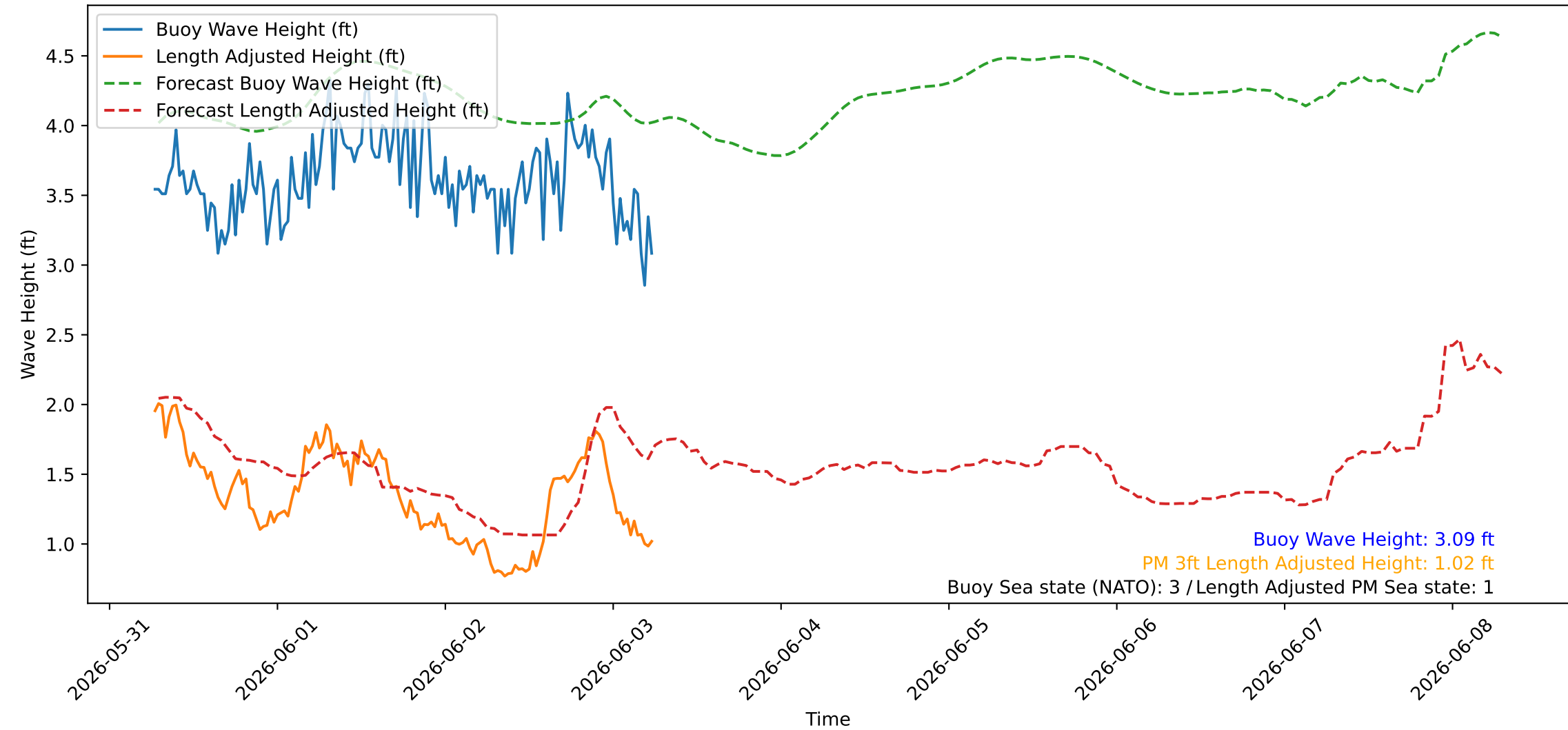
Wave Heights over Time for Green Beach at 2026-06-03 06:31:07
