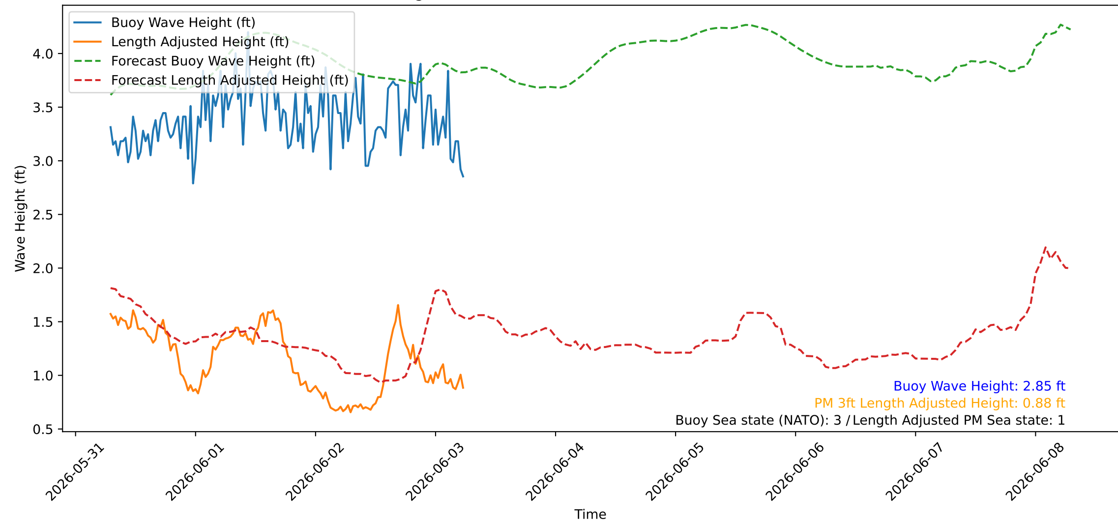
Wave Heights over Time for Red Beach at 2026-06-03 06:30:45
