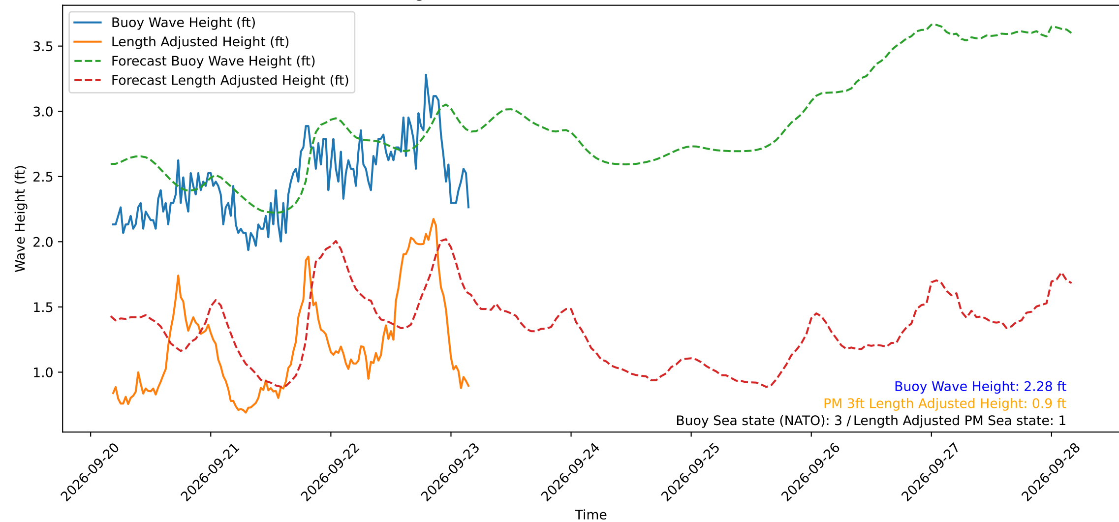
Wave Heights over Time for Red Beach at 2026-09-23 04:10:49
