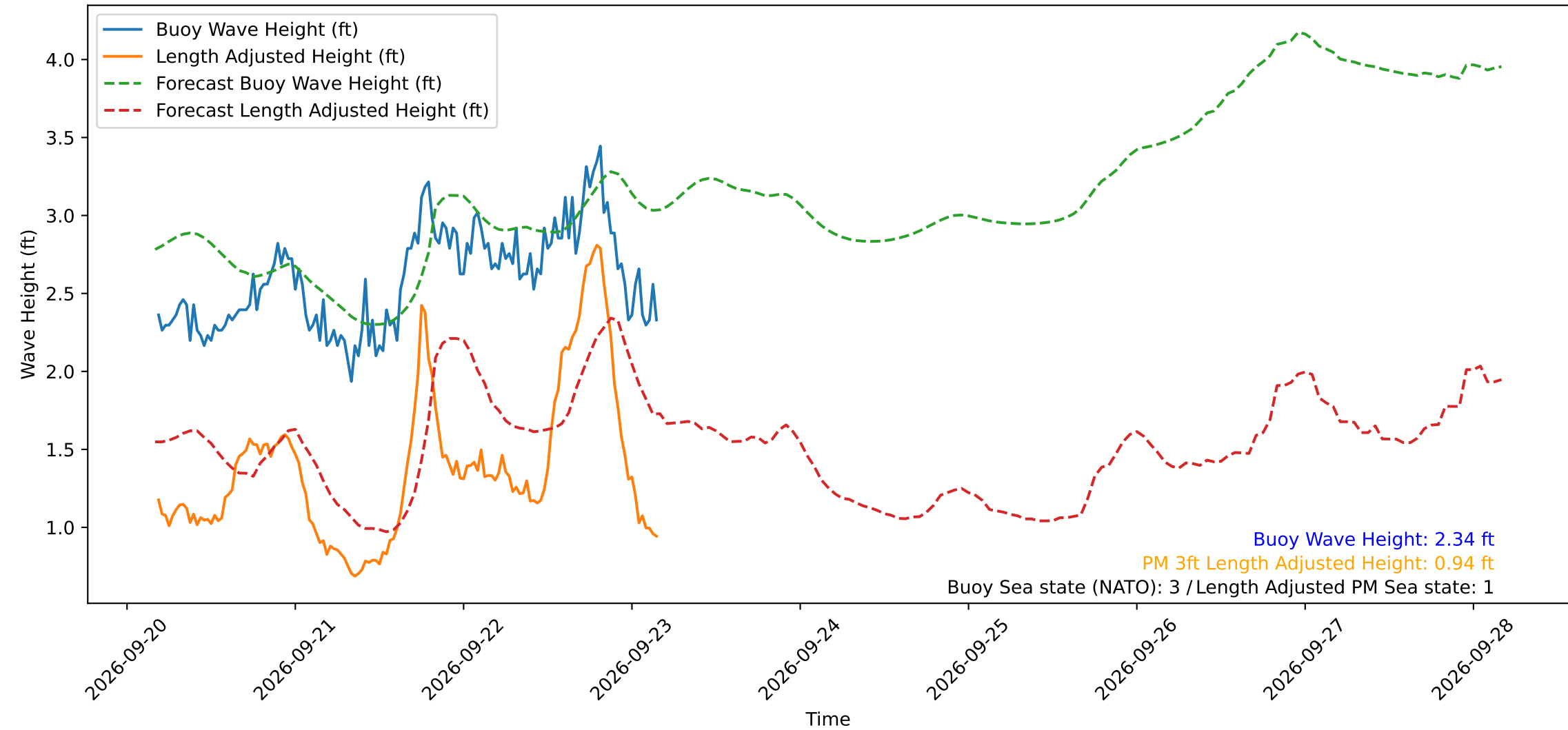
Wave Heights over Time for Green Beach at 2026-09-23 04:11:12
