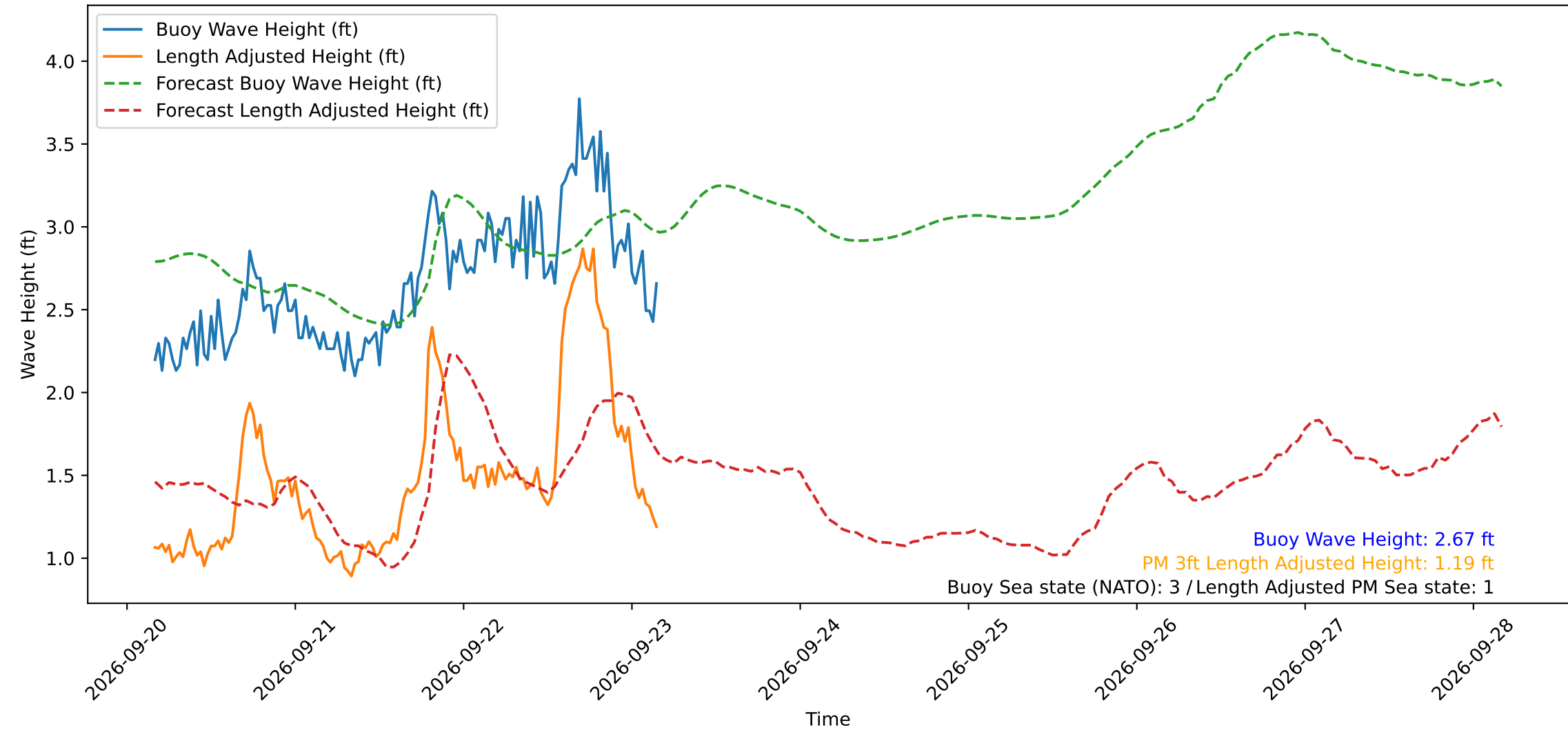
Wave Heights over Time for Oceanside Harbor at 2026-09-23 04:10:30
