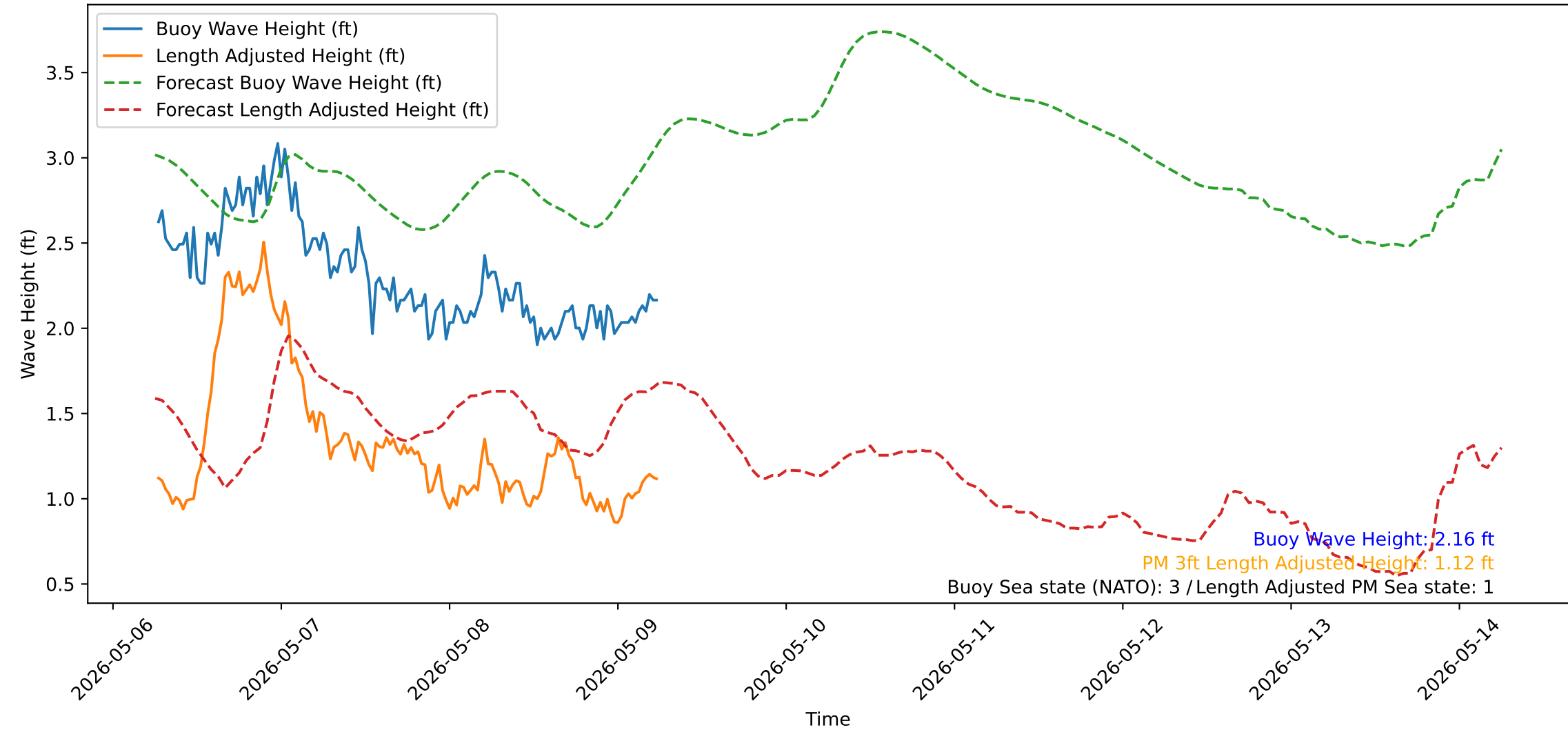
Wave Heights over Time for Red Beach at 2026-05-09 06:10:51
