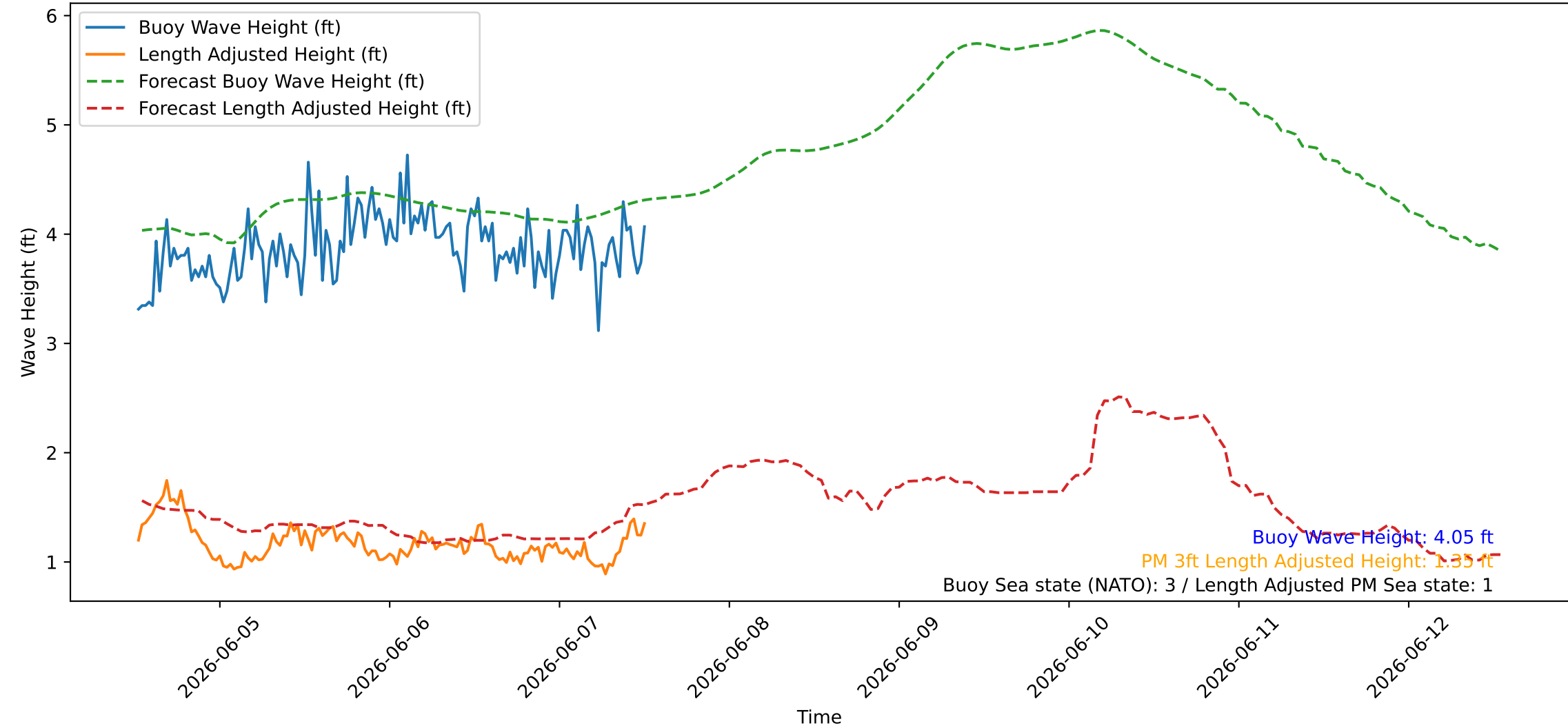
Wave Heights over Time for Green Beach at 2026-06-07 12:41:09
