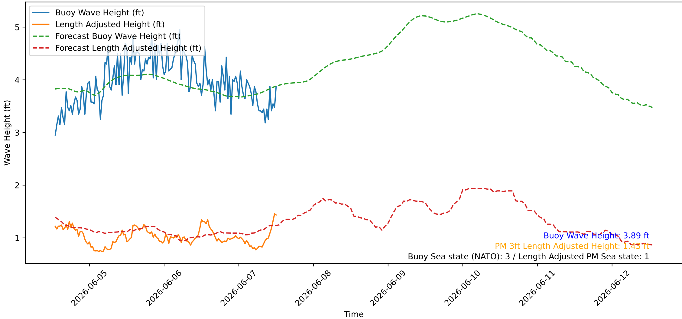
Wave Heights over Time for Red Beach at 2026-06-07 12:40:46
