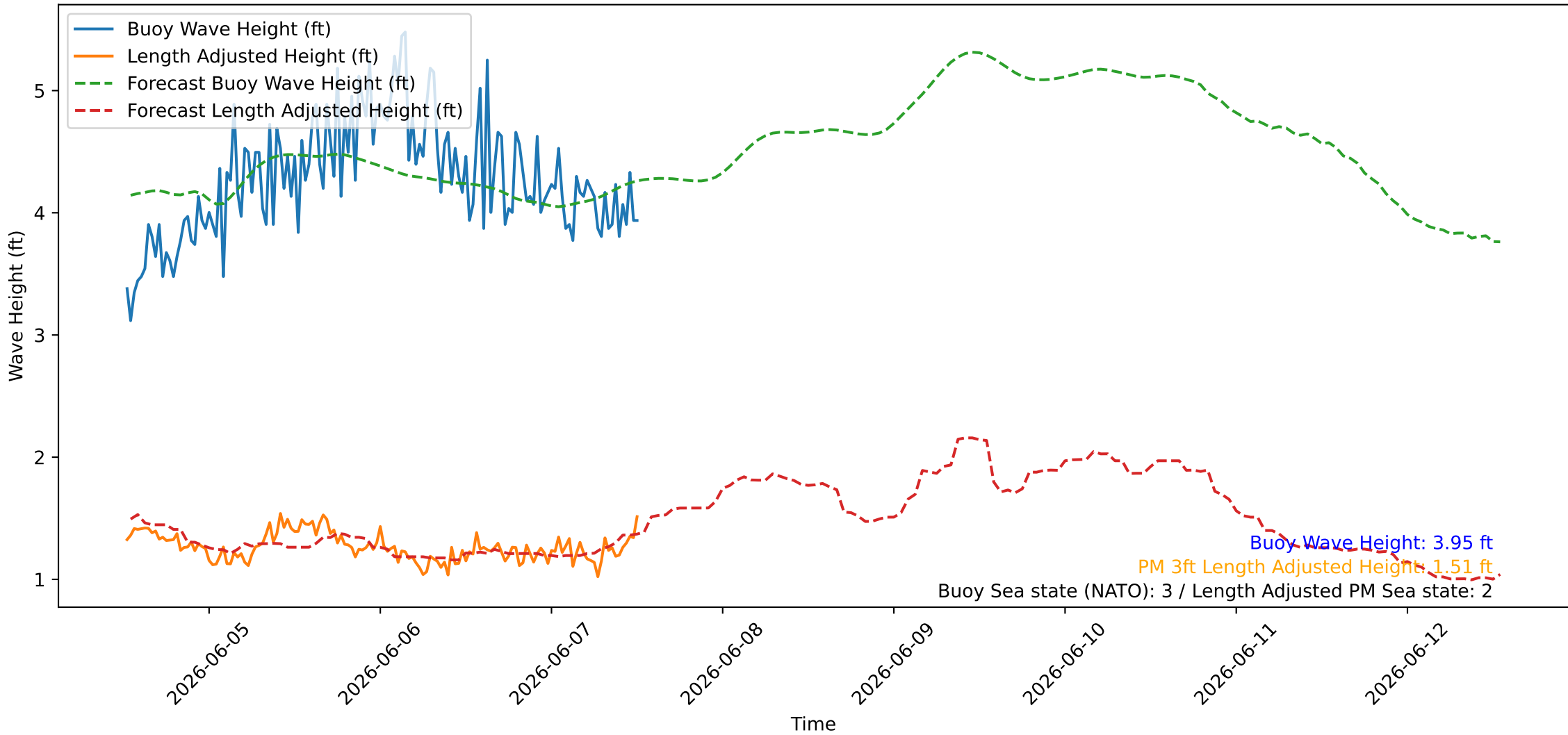
Wave Heights over Time for Oceanside Harbor at 2026-06-07 12:40:26
