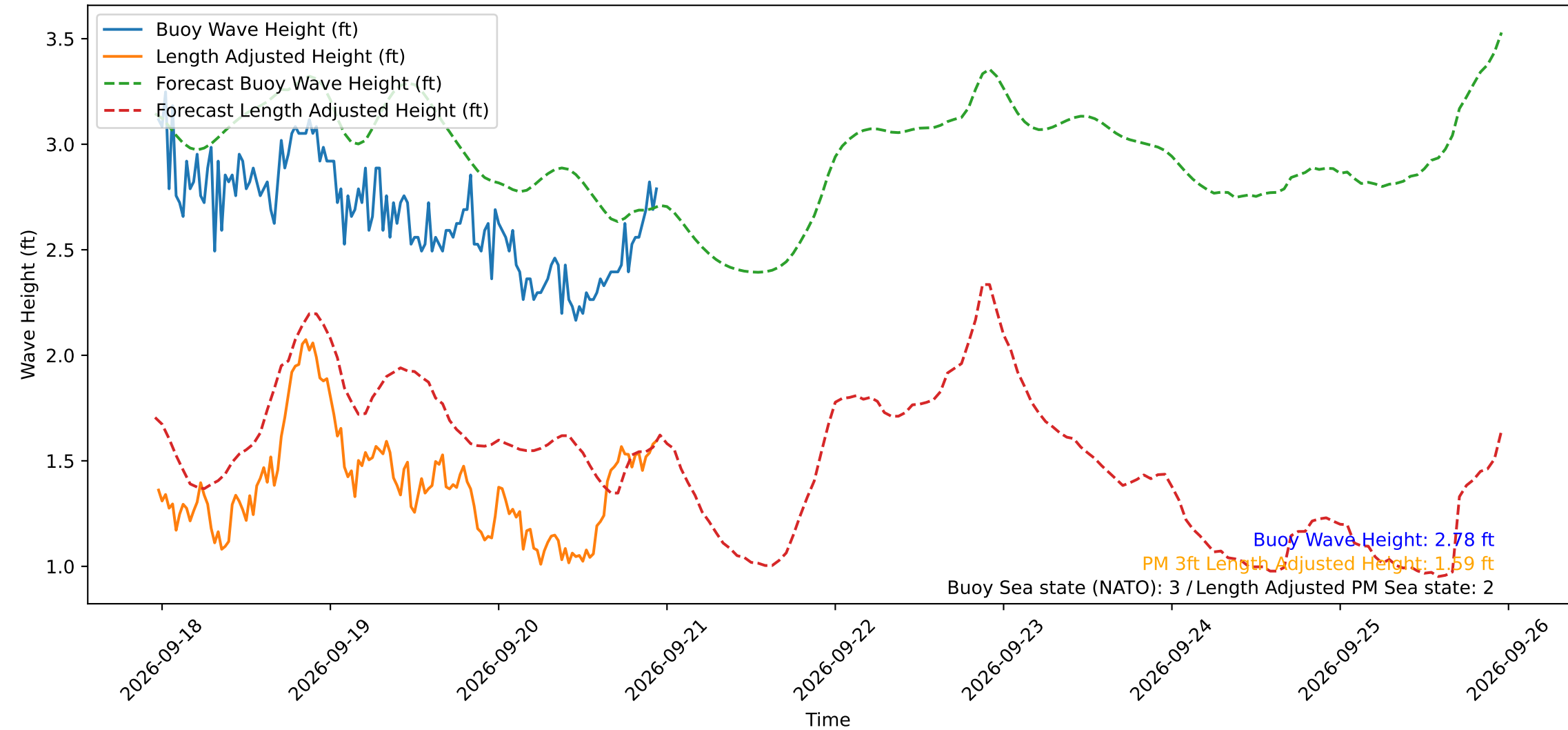
Wave Heights over Time for Green Beach at 2026-09-20 23:21:16
