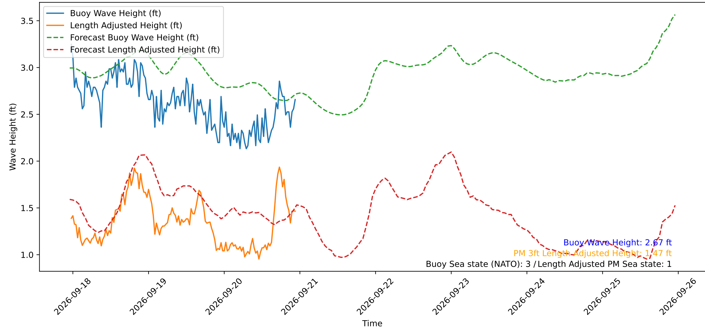
Wave Heights over Time for Oceanside Harbor at 2026-09-20 23:20:31
