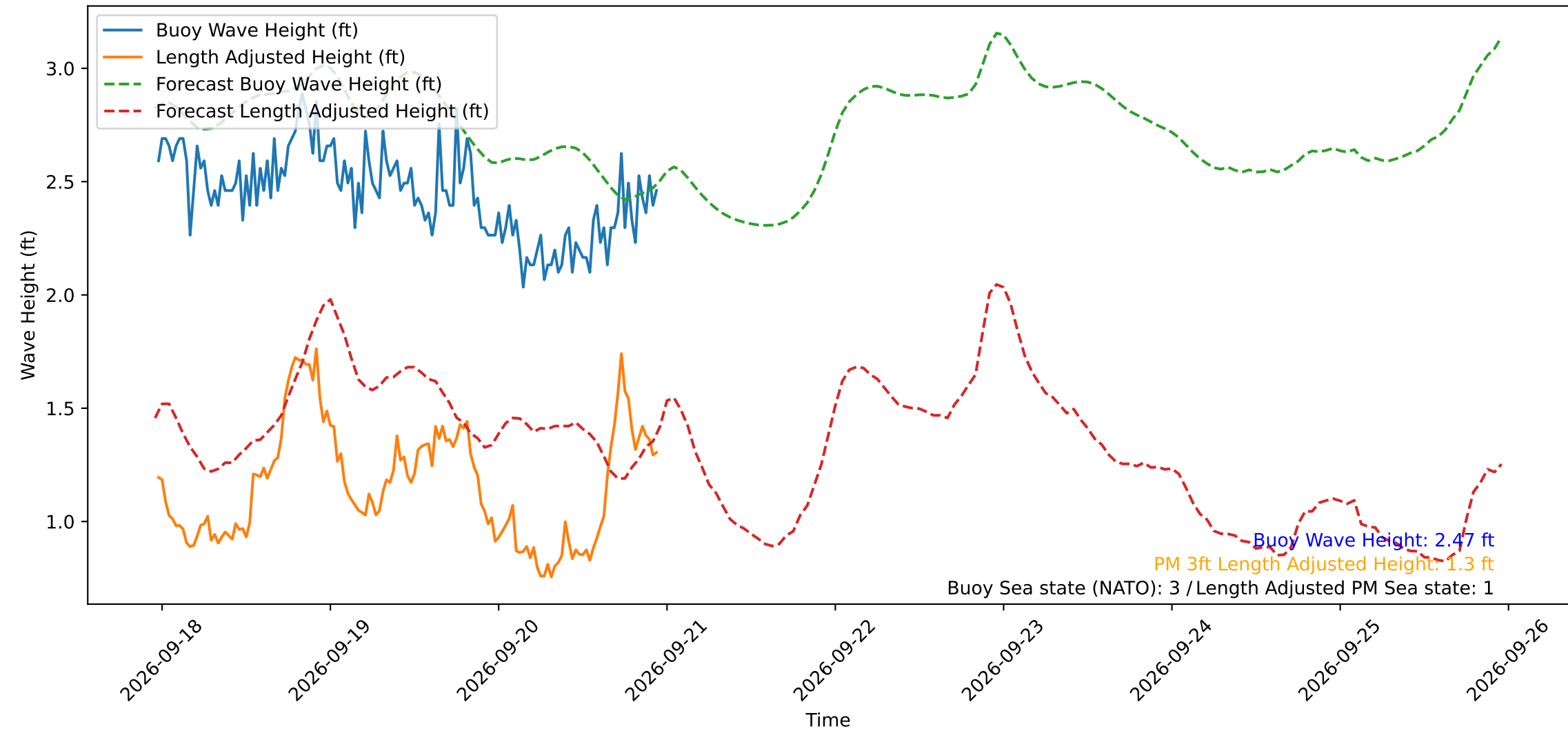
Wave Heights over Time for Red Beach at 2026-09-20 23:20:52
