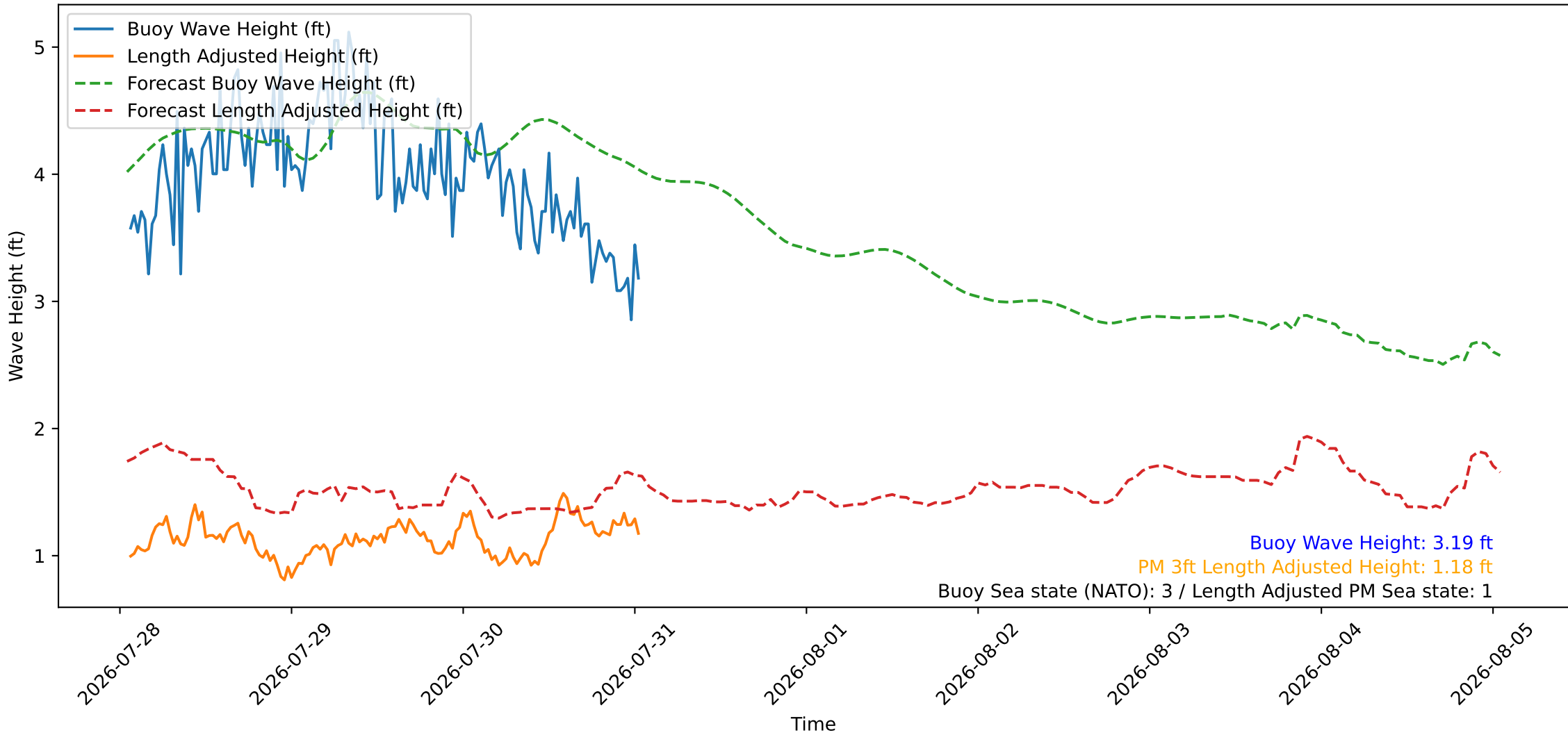
Wave Heights over Time for Red Beach at 2026-07-31 01:10:46
