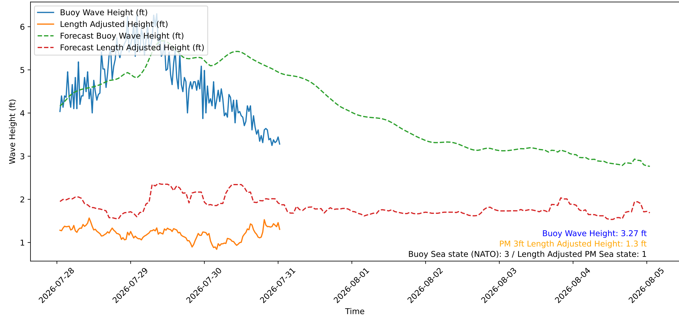
Wave Heights over Time for Green Beach at 2026-07-31 01:11:08
