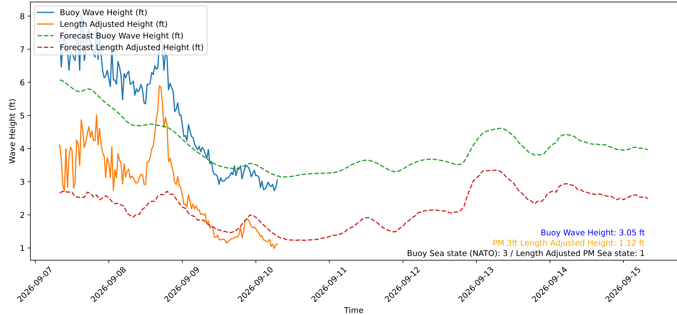
Wave Heights over Time for Green Beach at 2026-09-10 07:41:11
