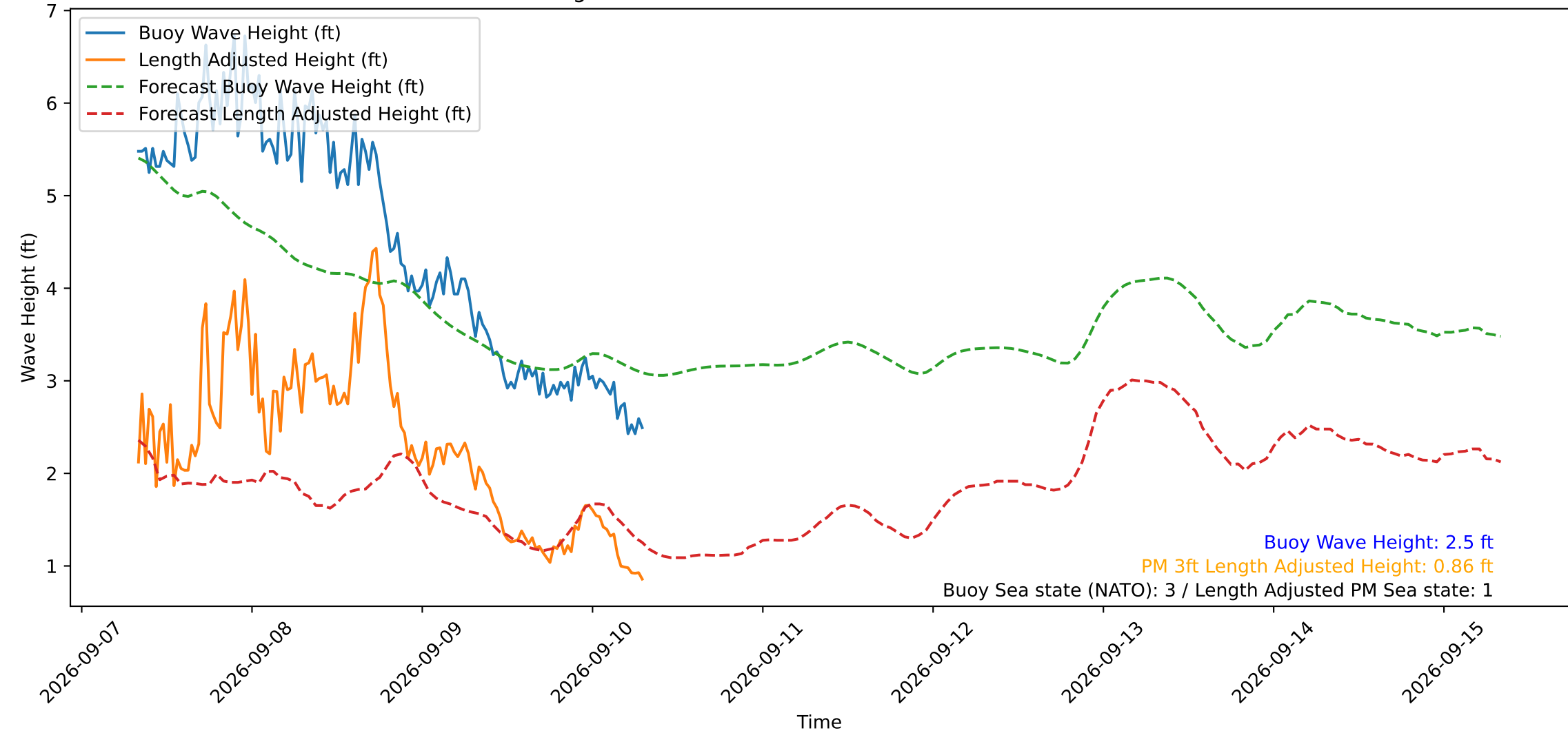
Wave Heights over Time for Red Beach at 2026-09-10 07:40:49
