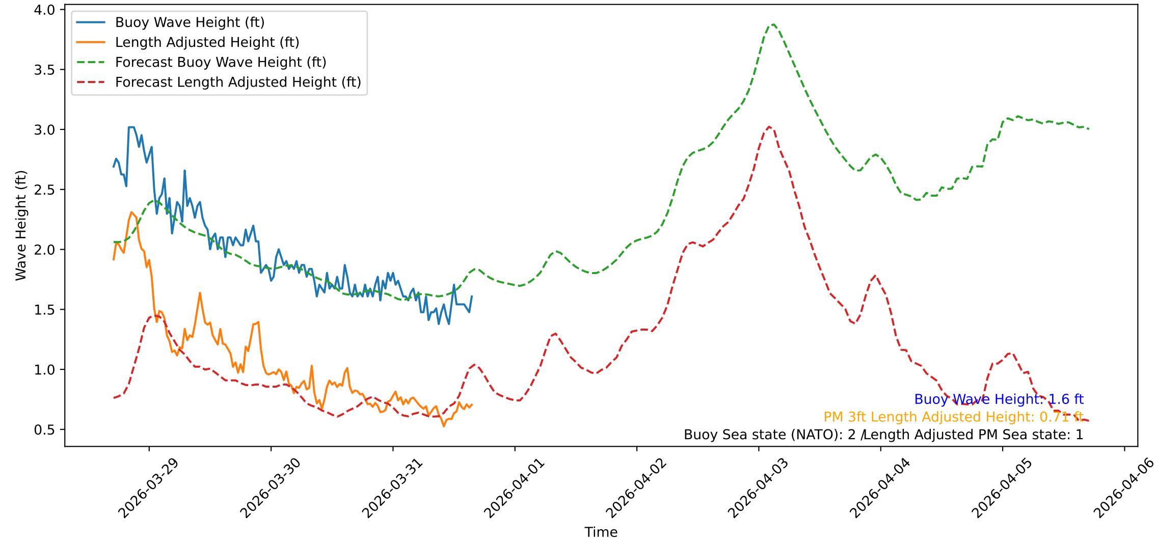
Wave Heights over Time for Red Beach at 2026-03-31 16:30:47
