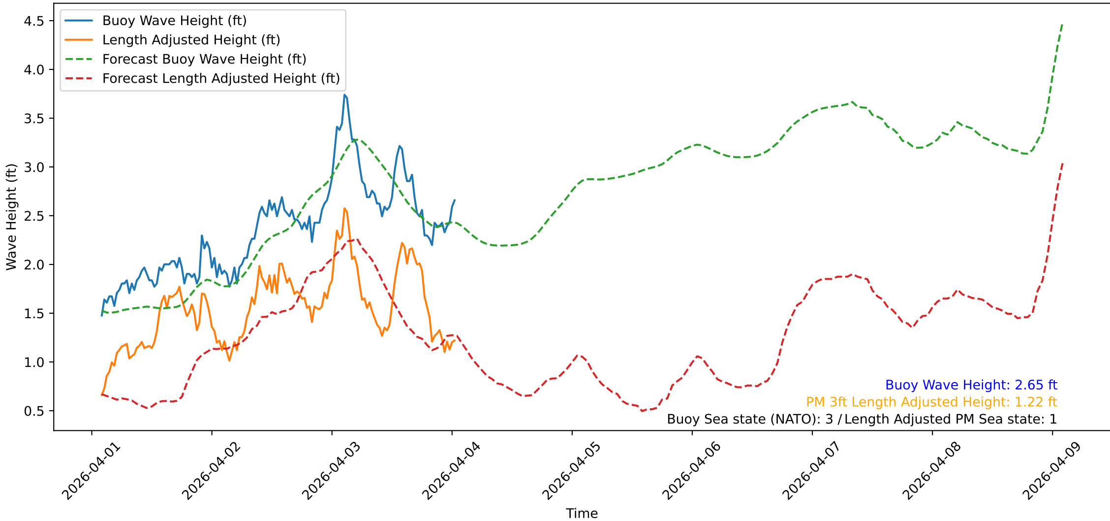
Wave Heights over Time for Red Beach at 2026-04-04 01:30:47
