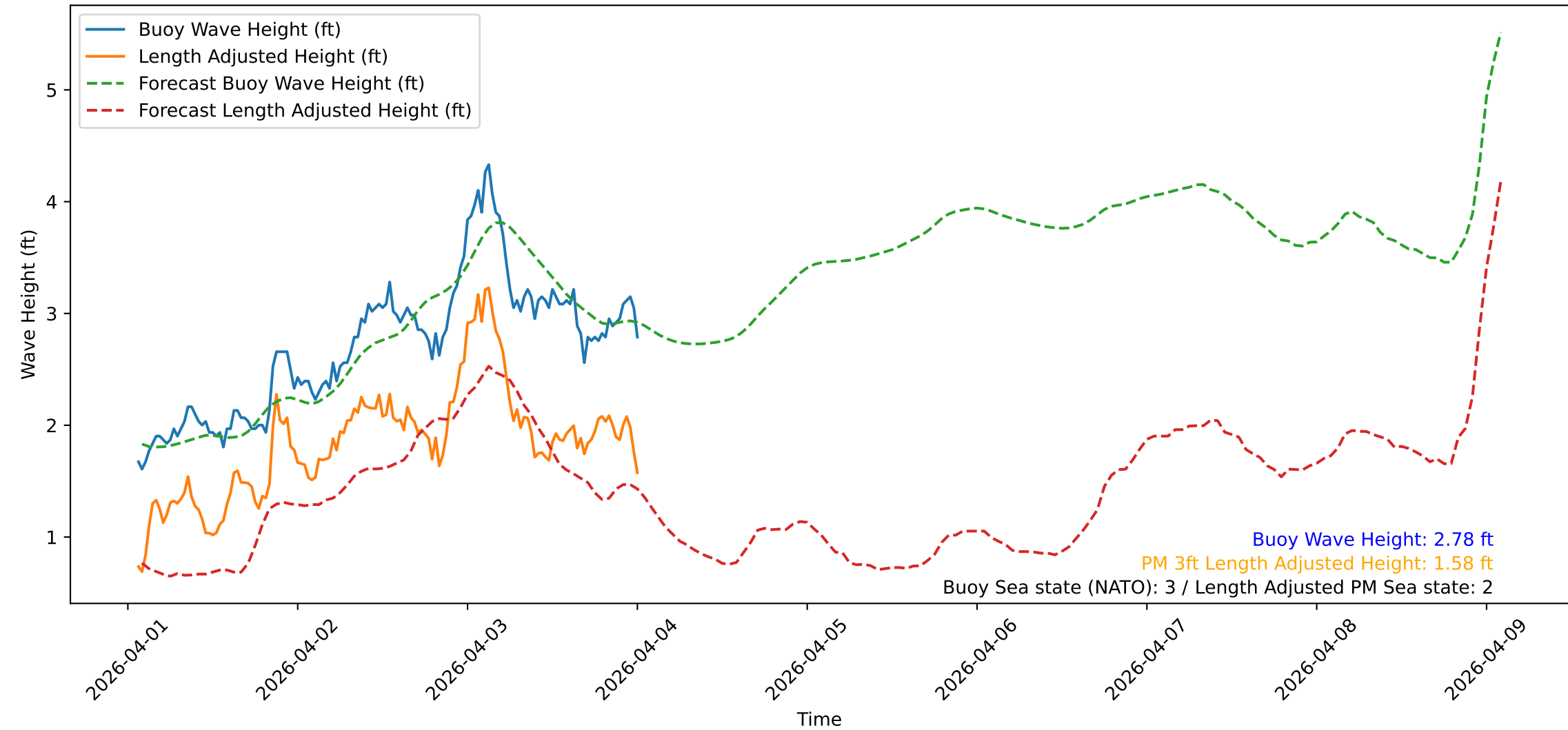
Wave Heights over Time for Green Beach at 2026-04-04 01:31:09
