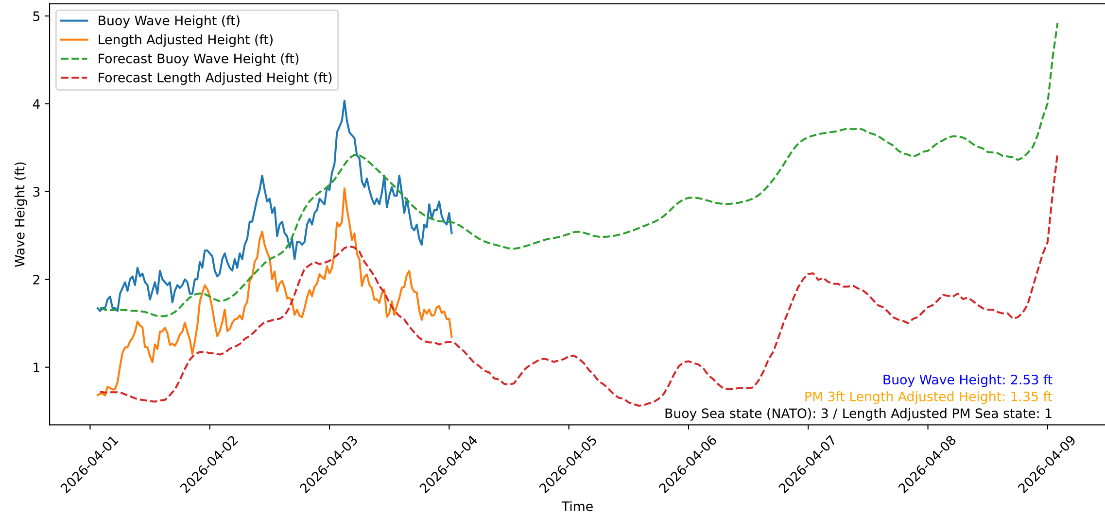
Wave Heights over Time for Oceanside Harbor at 2026-04-04 01:30:31
