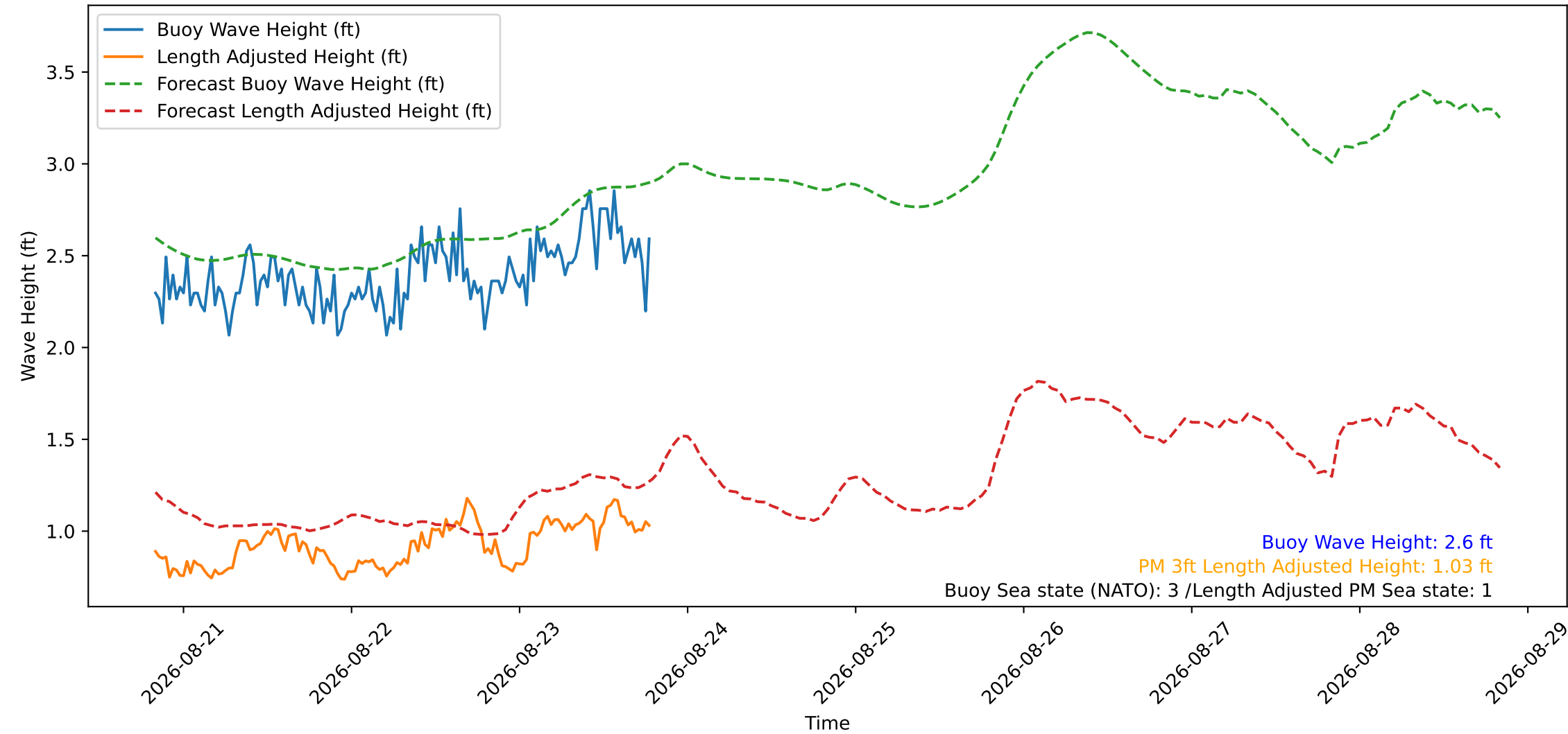
Wave Heights over Time for Red Beach at 2026-08-23 19:30:49
