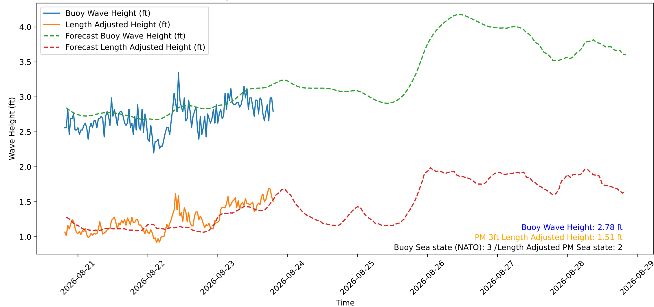
Wave Heights over Time for Oceanside Harbor at 2026-08-23 19:30:29
