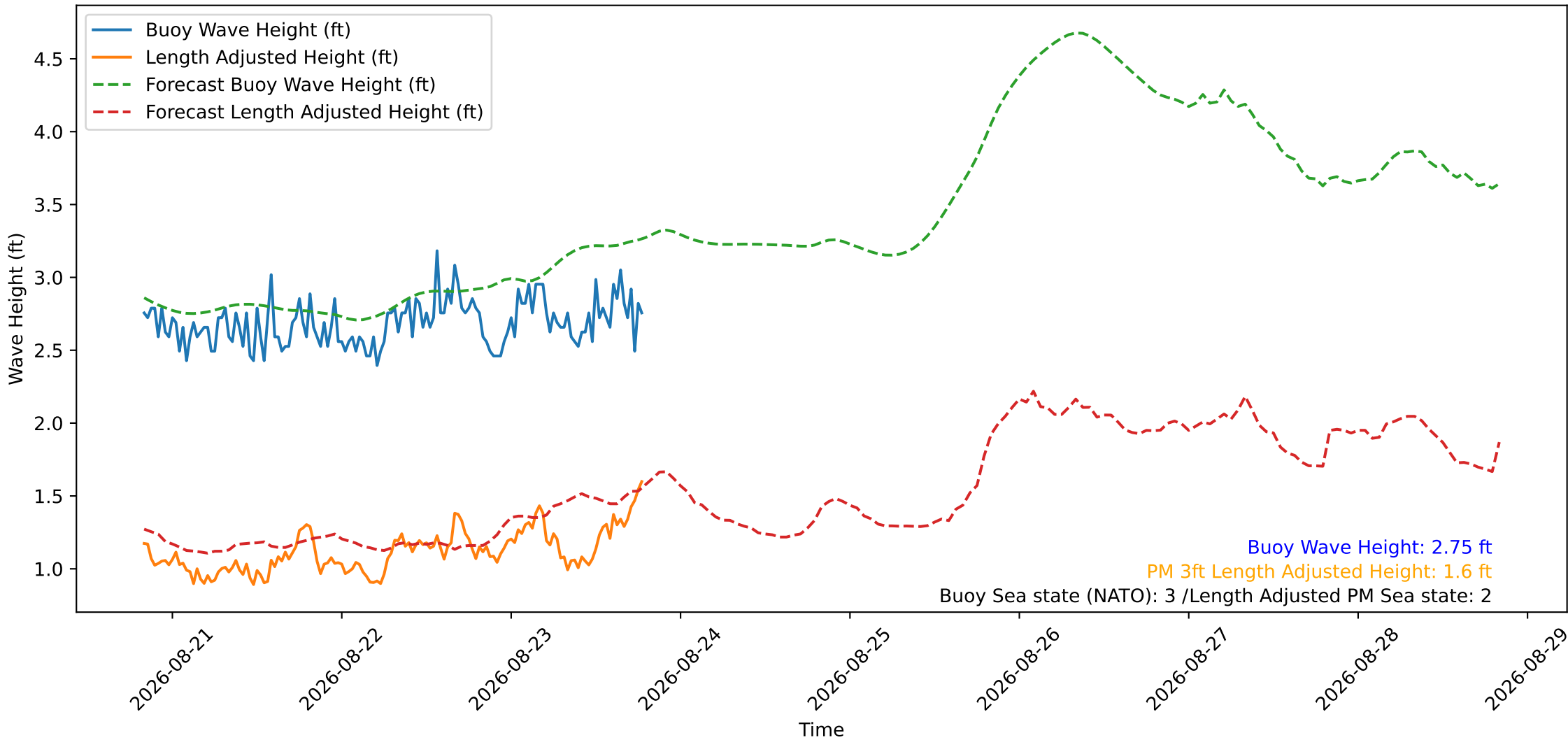
Wave Heights over Time for Green Beach at 2026-08-23 19:31:11
