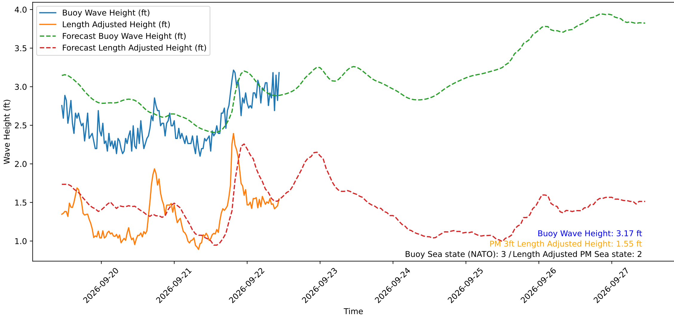
Wave Heights over Time for Oceanside Harbor at 2026-09-22 11:10:29
