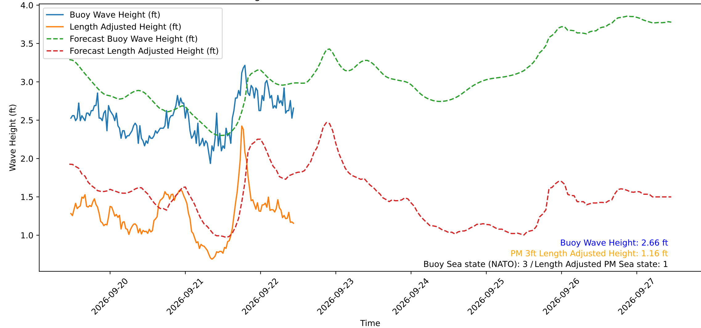
Wave Heights over Time for Green Beach at 2026-09-22 11:11:11
