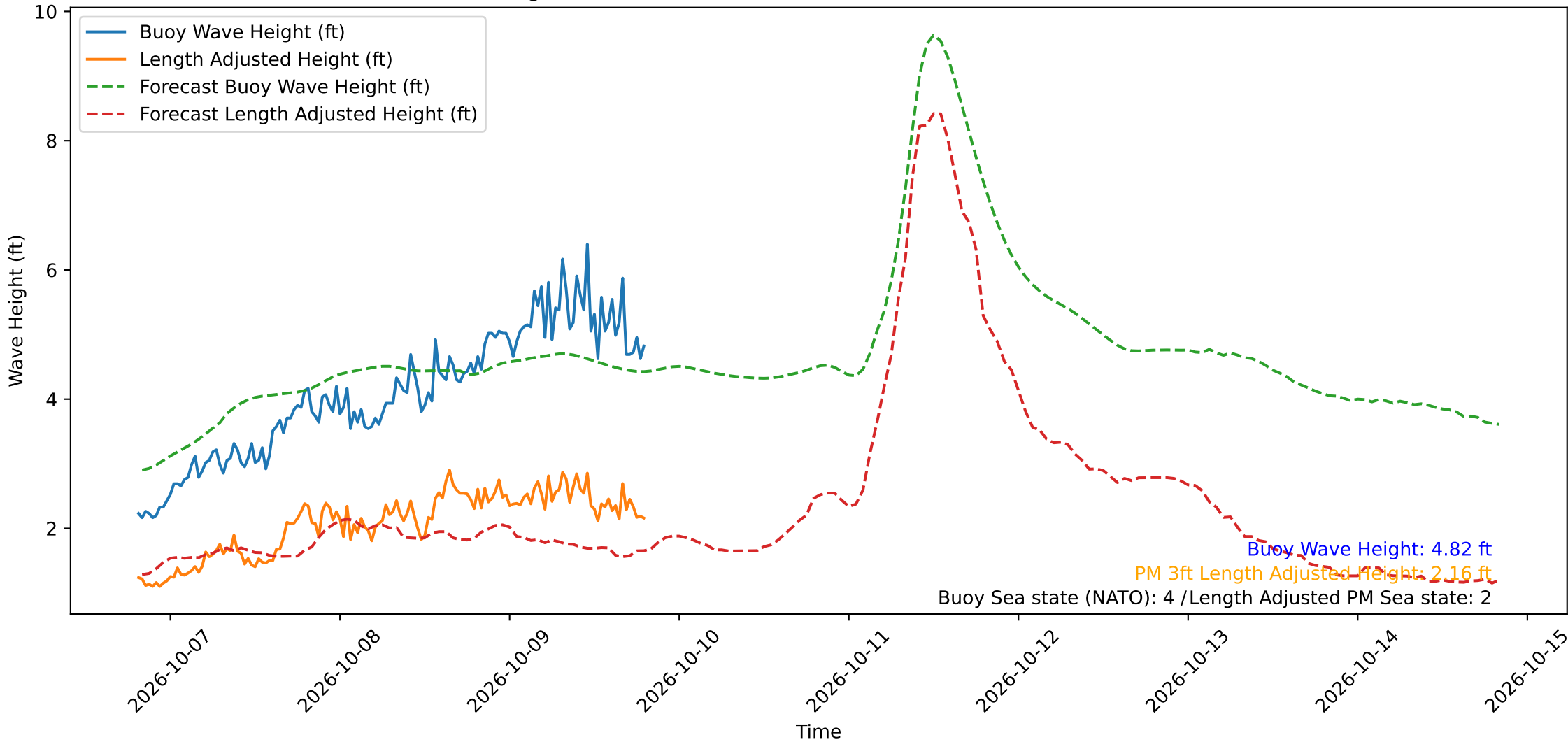
Wave Heights over Time for Oceanside Harbor at 2026-10-09 19:40:30
