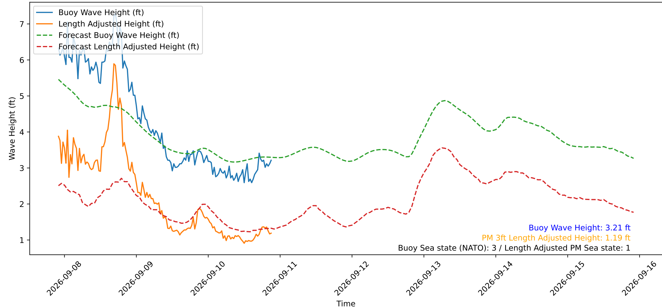
Wave Heights over Time for Green Beach at 2026-09-10 21:41:12
