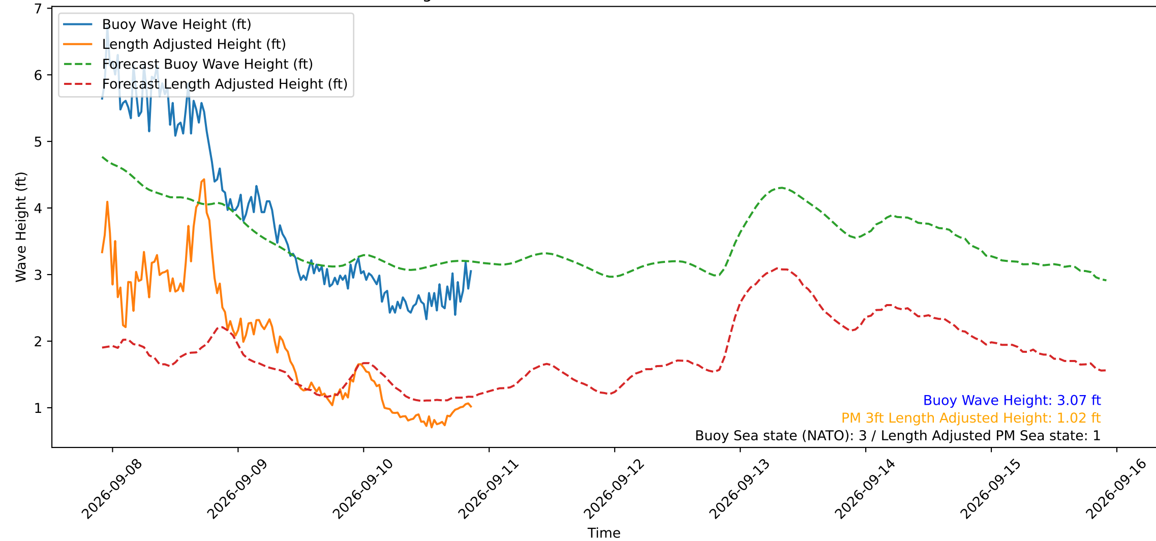
Wave Heights over Time for Red Beach at 2026-09-10 21:40:49
