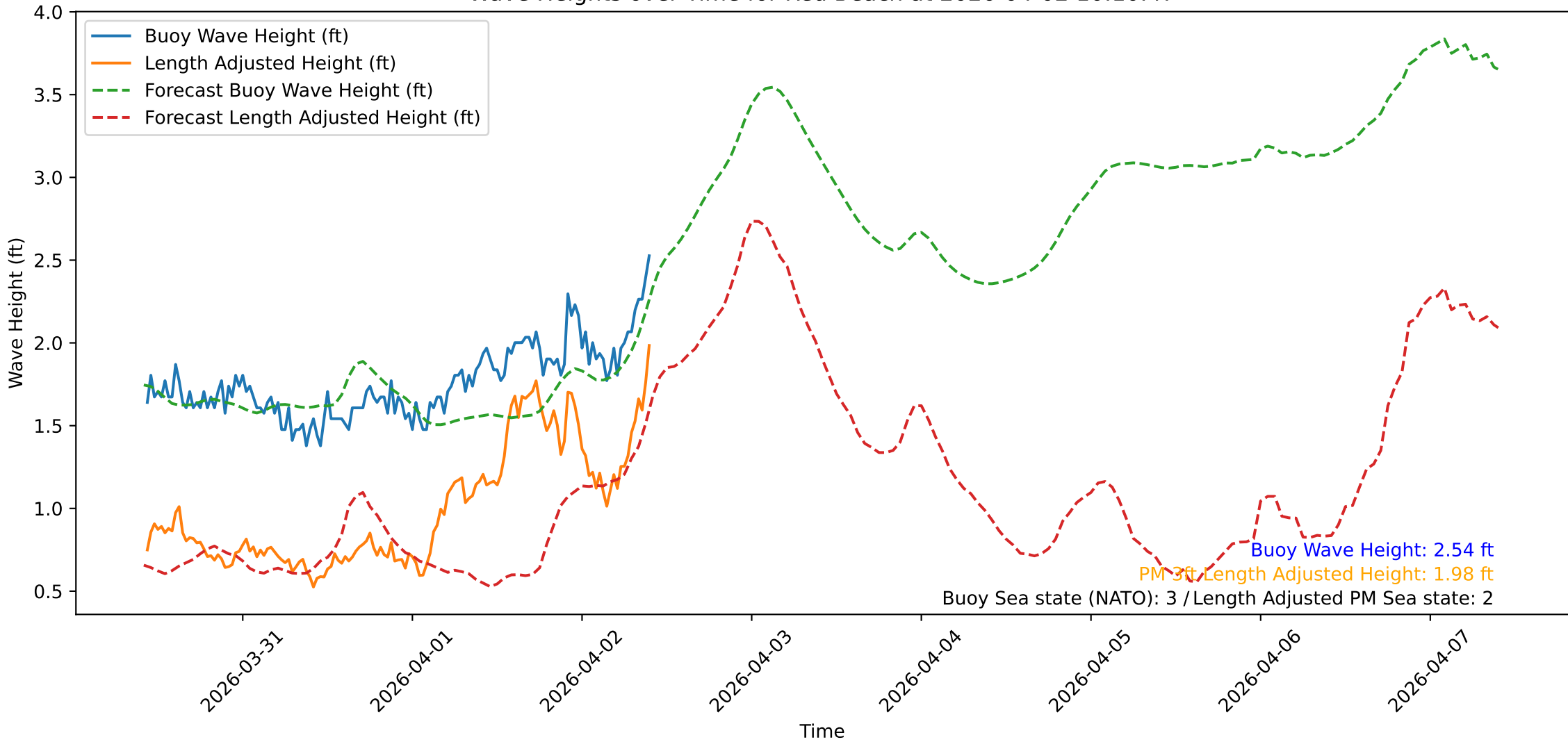
Wave Heights over Time for Red Beach at 2026-04-02 10:10:47
