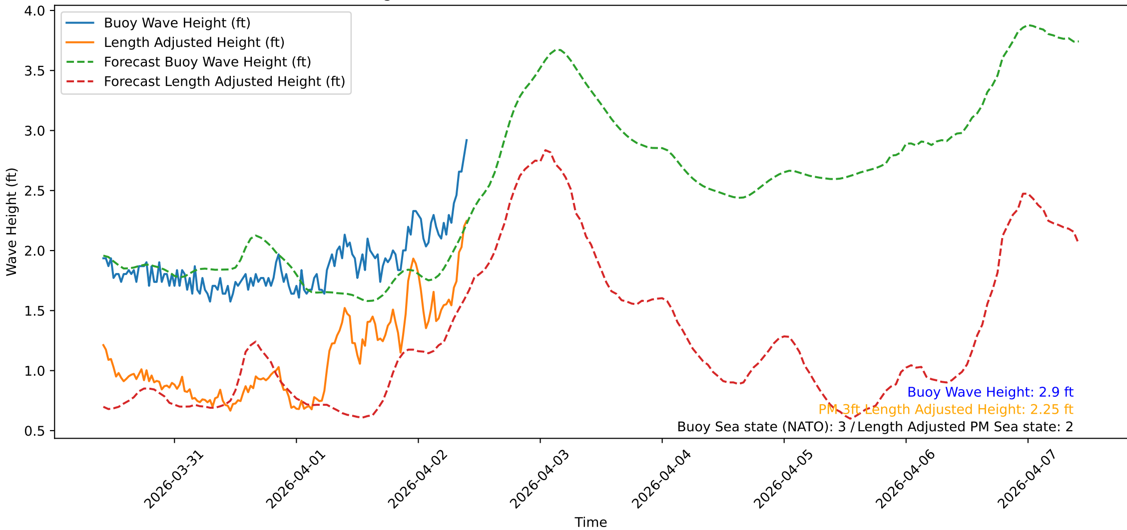
Wave Heights over Time for Oceanside Harbor at 2026-04-02 10:10:31
