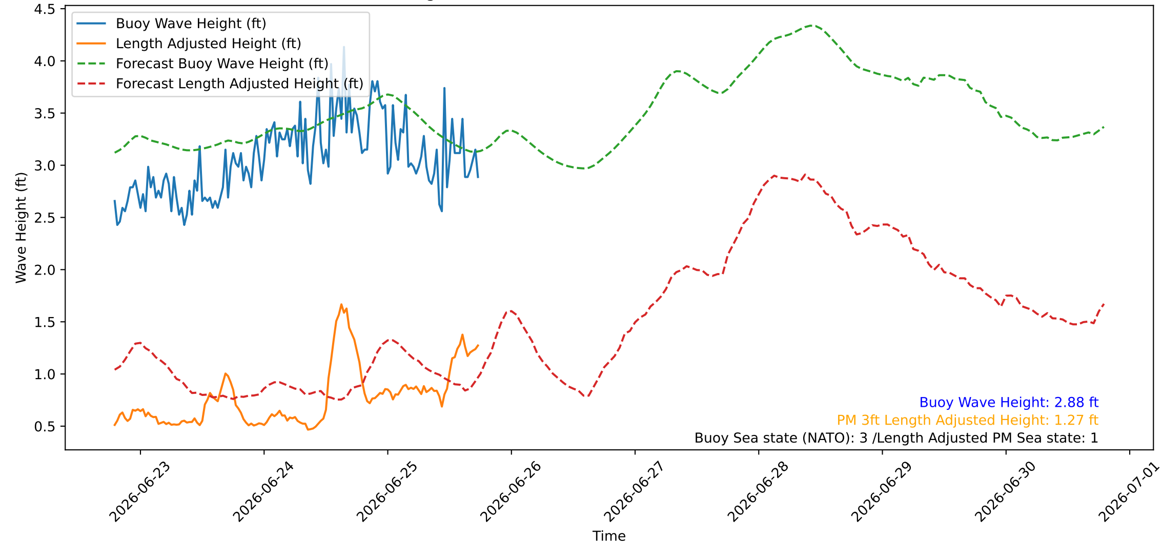
Wave Heights over Time for Red Beach at 2026-06-25 18:50:46
