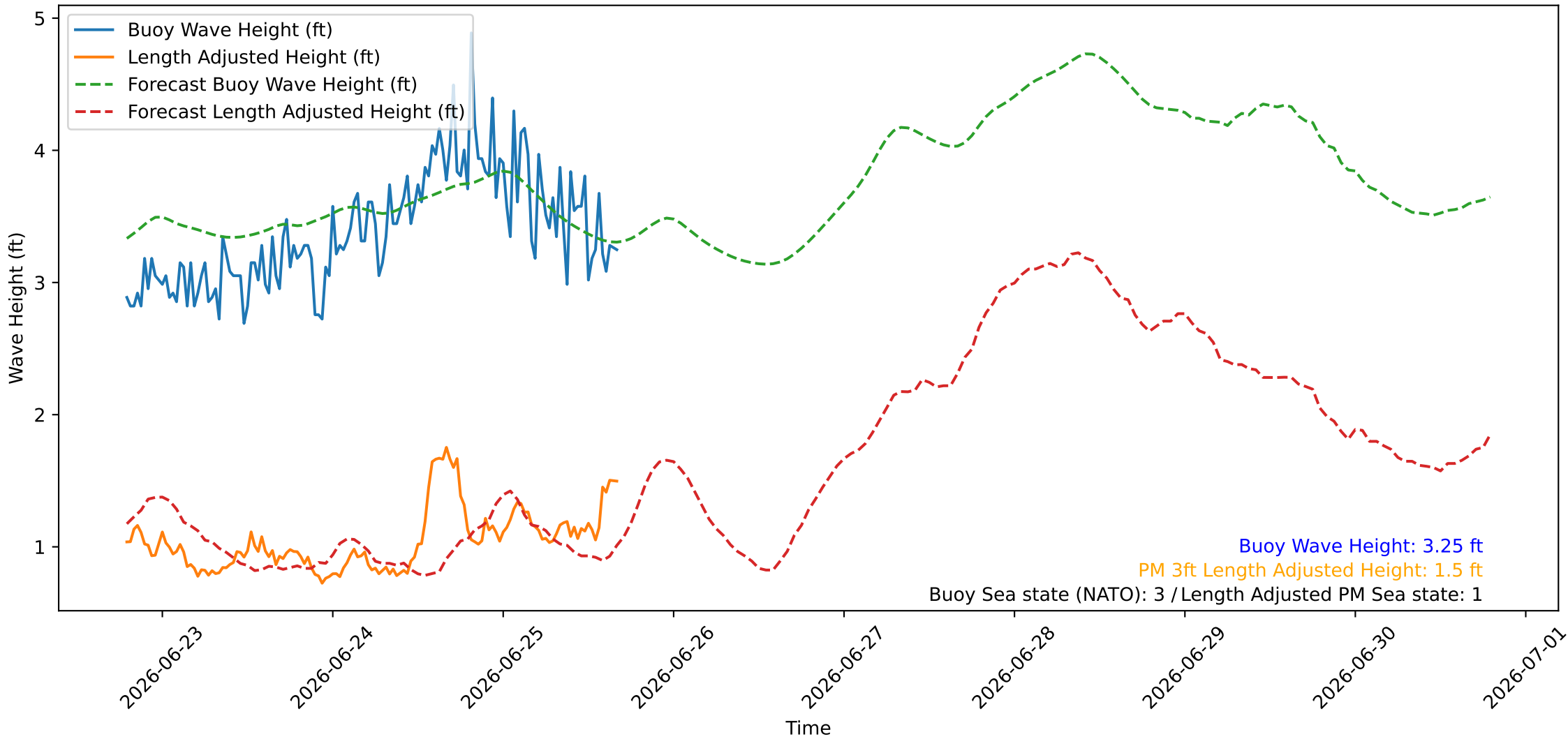
Wave Heights over Time for Oceanside Harbor at 2026-06-25 18:50:26
