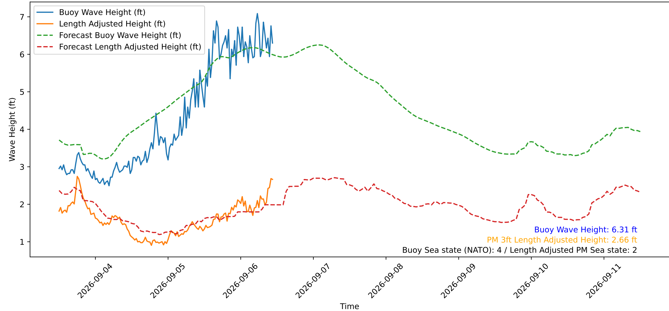
Wave Heights over Time for Green Beach at 2026-09-06 11:31:11
