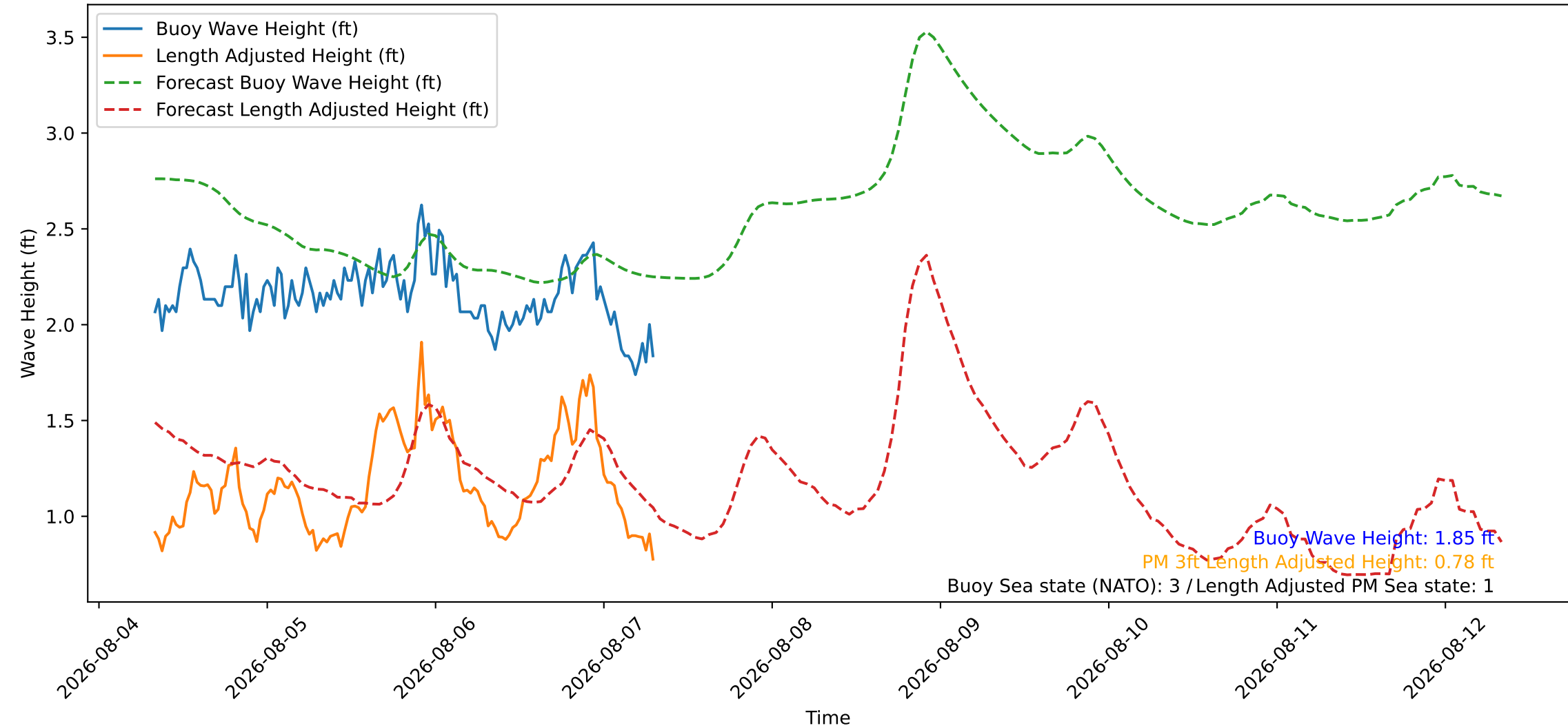
Wave Heights over Time for Green Beach at 2026-08-07 07:51:10
