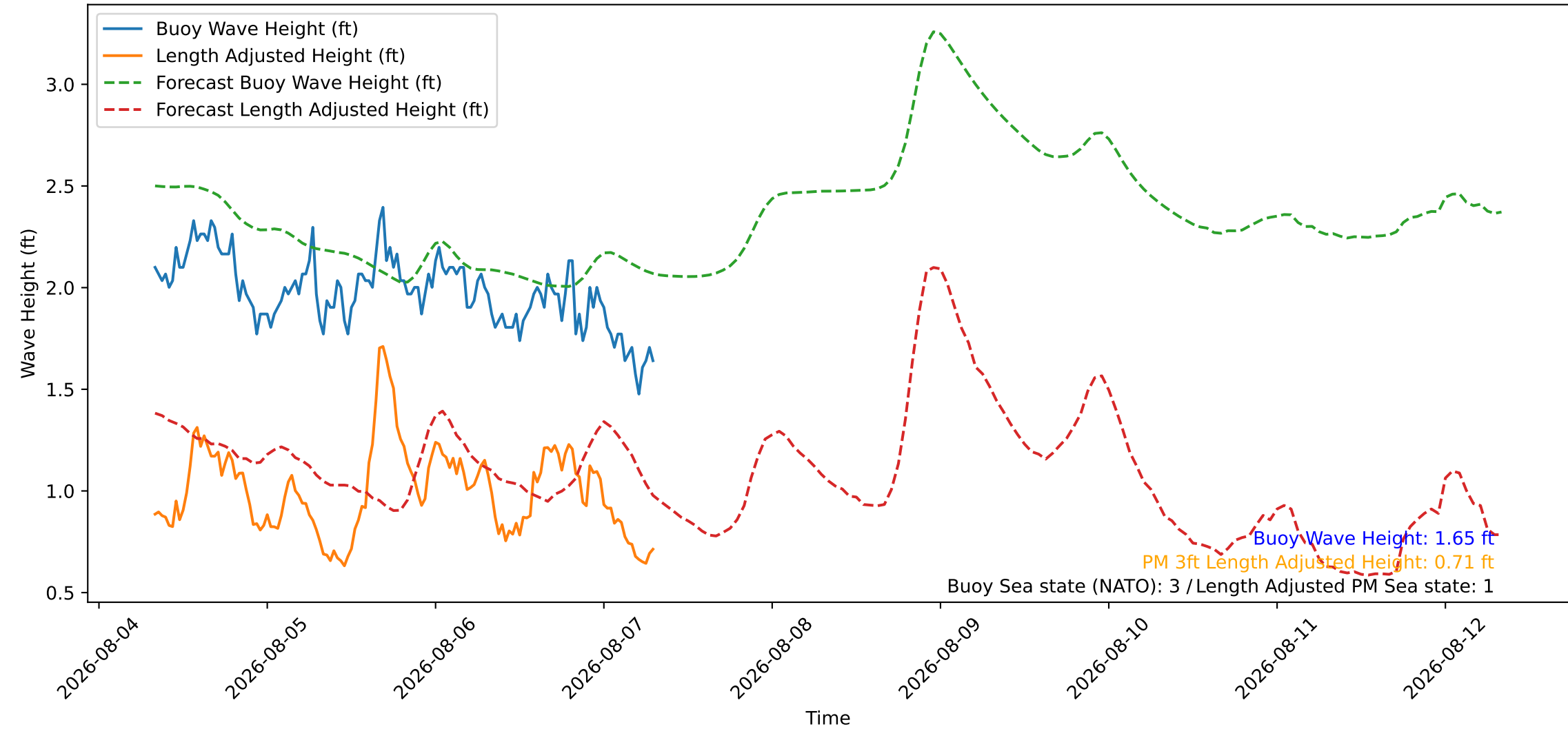
Wave Heights over Time for Red Beach at 2026-08-07 07:50:47
