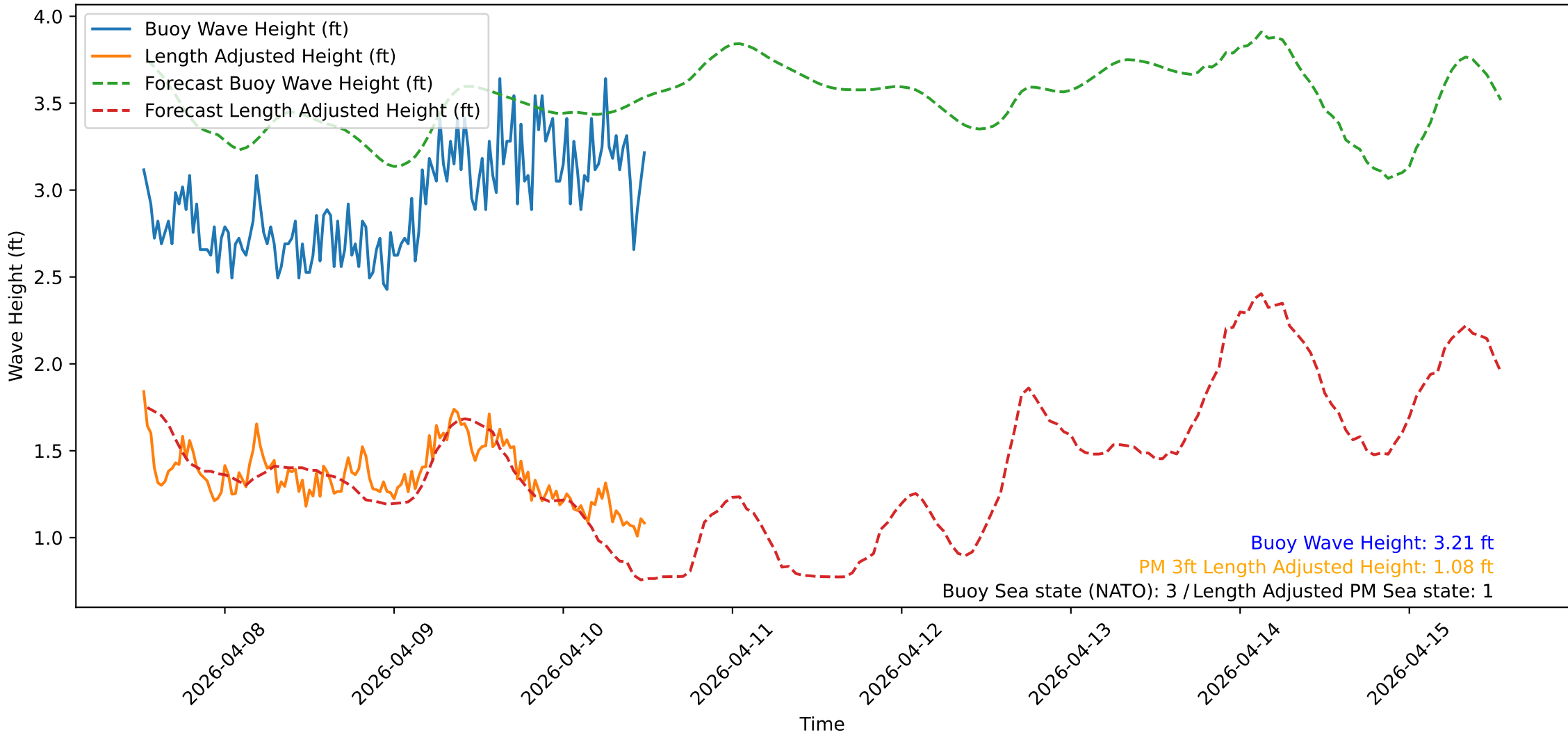
Wave Heights over Time for Oceanside Harbor at 2026-04-10 12:30:31
