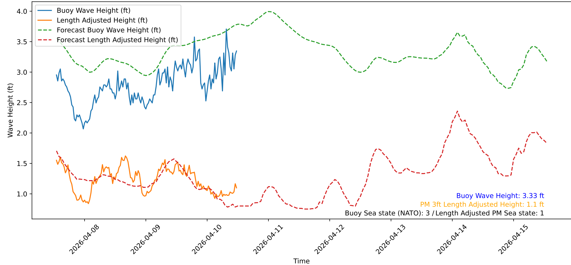
Wave Heights over Time for Red Beach at 2026-04-10 12:30:50
