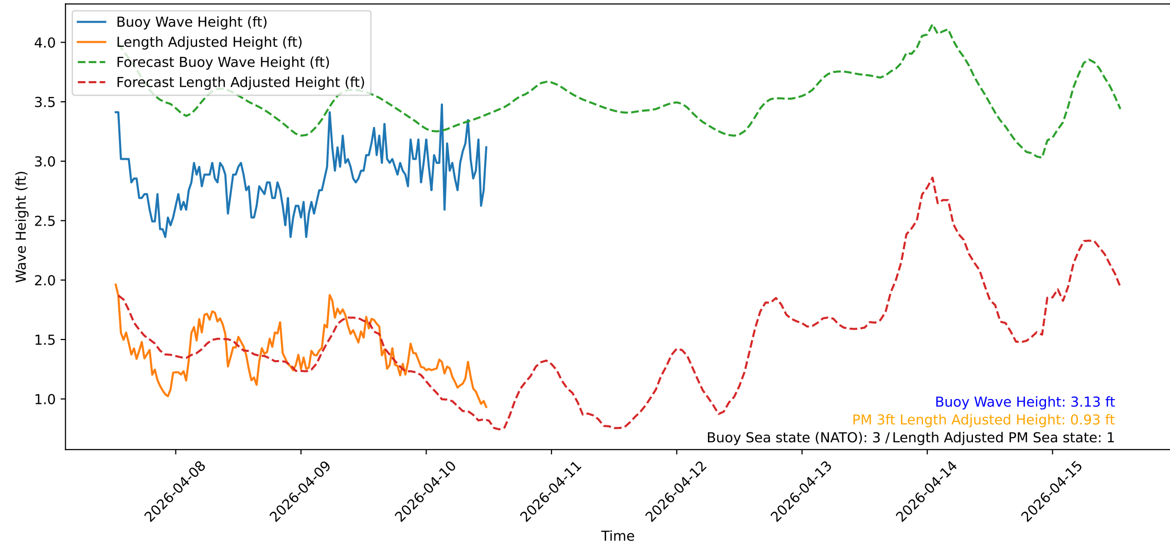
Wave Heights over Time for Green Beach at 2026-04-10 12:31:12
