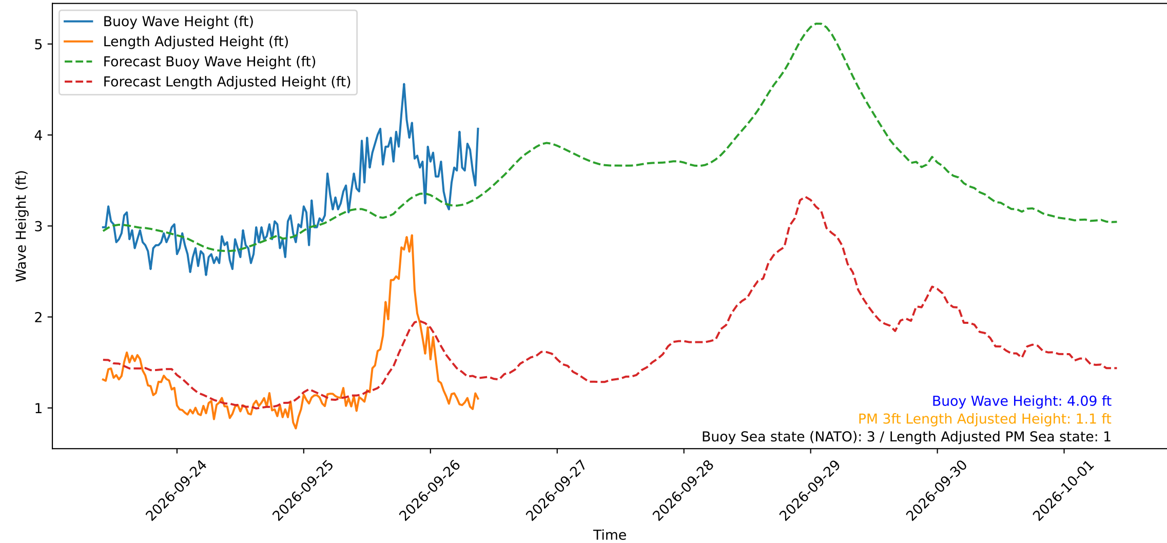
Wave Heights over Time for Green Beach at 2026-09-26 09:41:12
