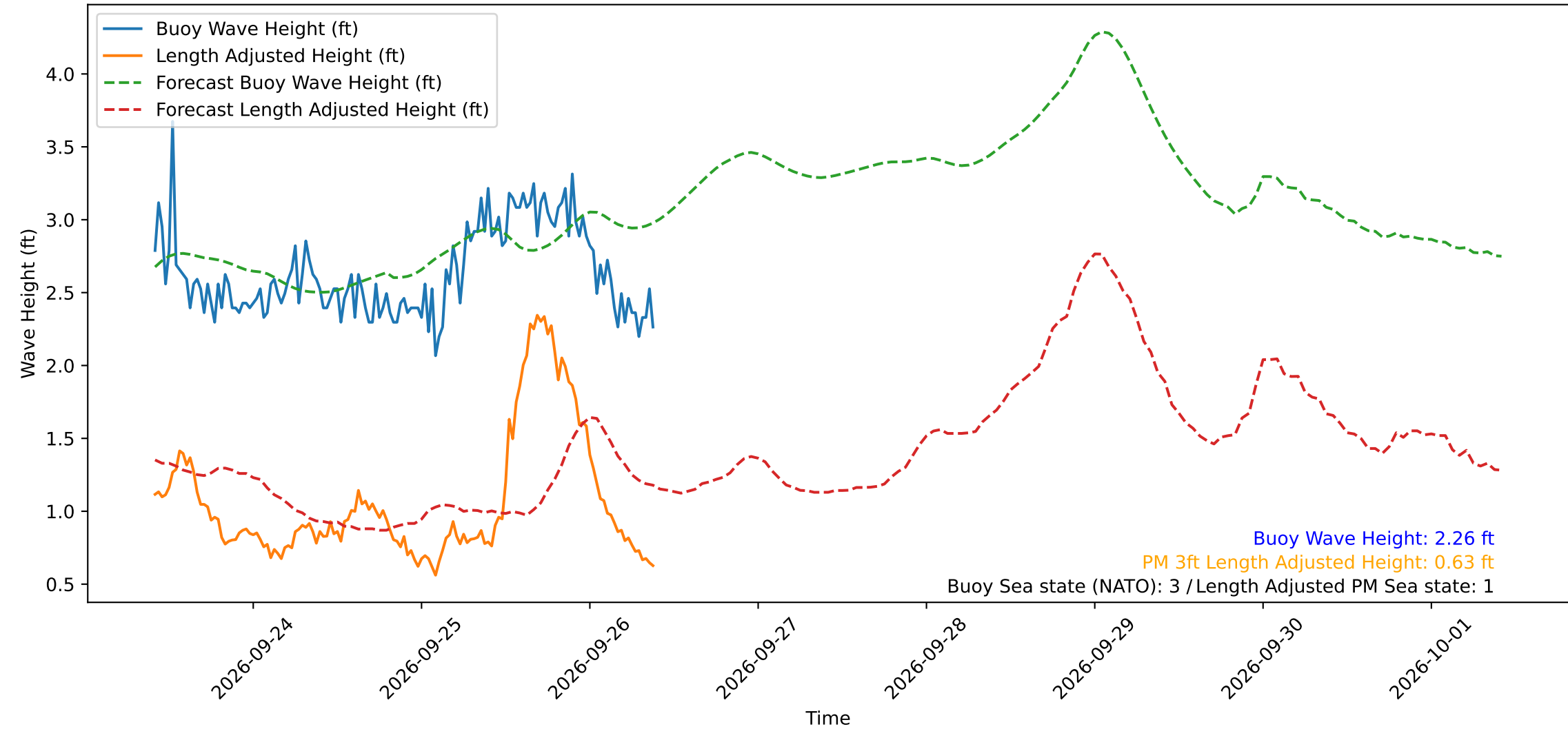
Wave Heights over Time for Red Beach at 2026-09-26 09:40:50
