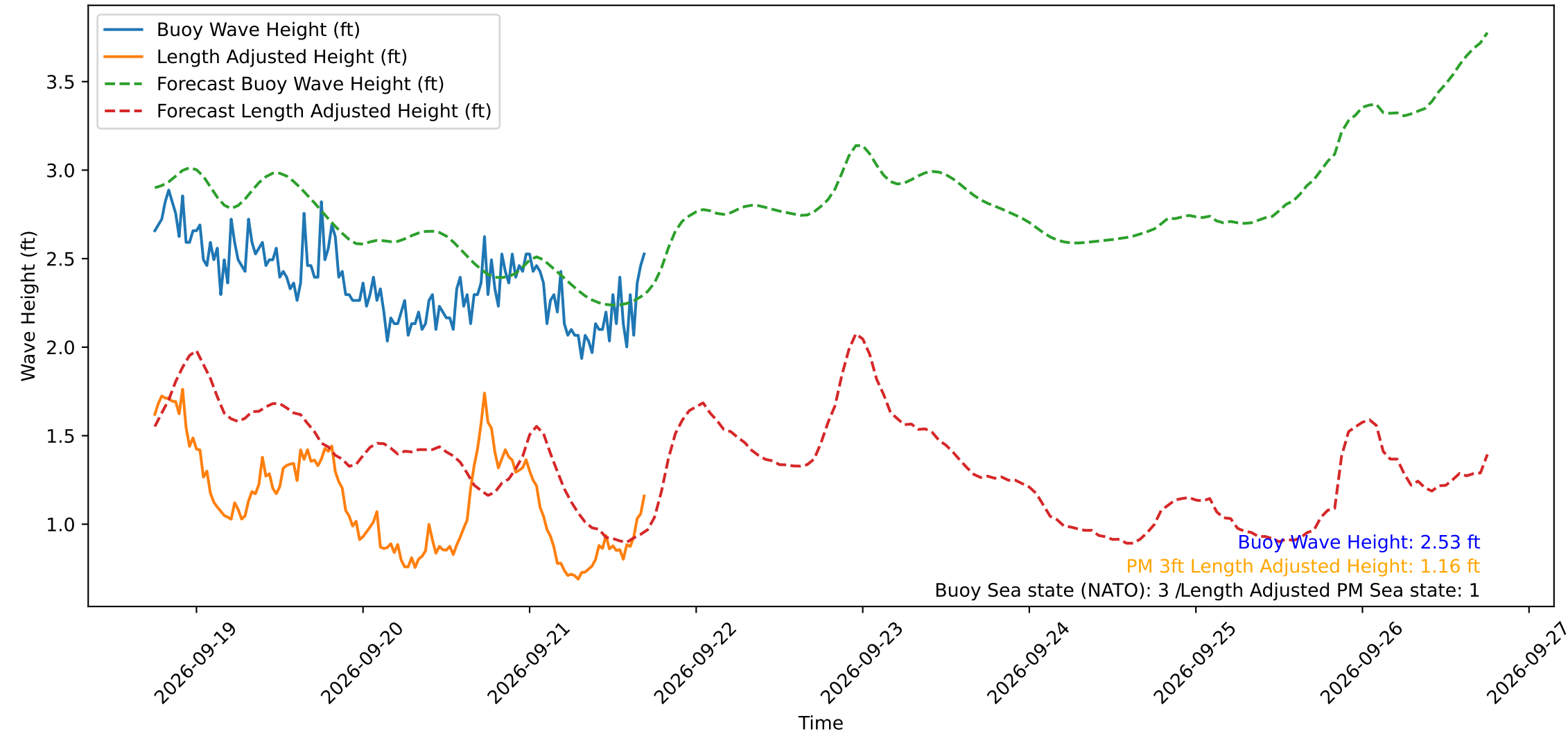
Wave Heights over Time for Red Beach at 2026-09-21 17:40:49
