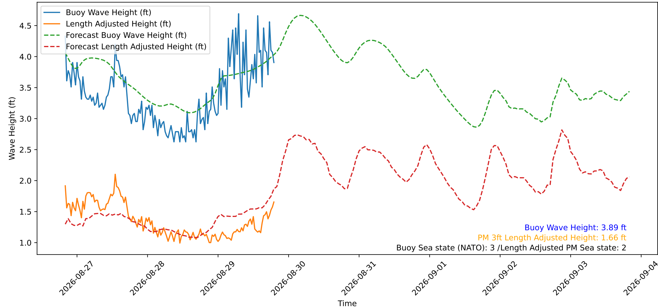
Wave Heights over Time for Red Beach at 2026-08-29 19:50:50
