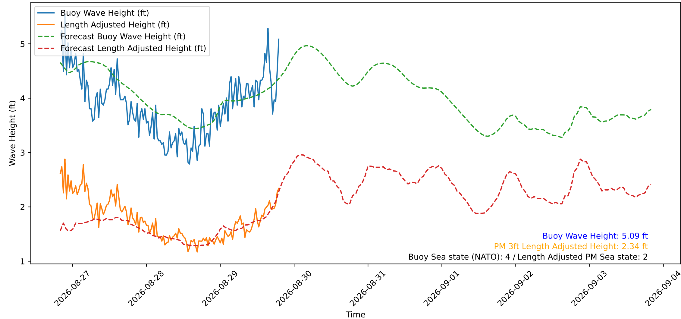
Wave Heights over Time for Oceanside Harbor at 2026-08-29 19:50:29
