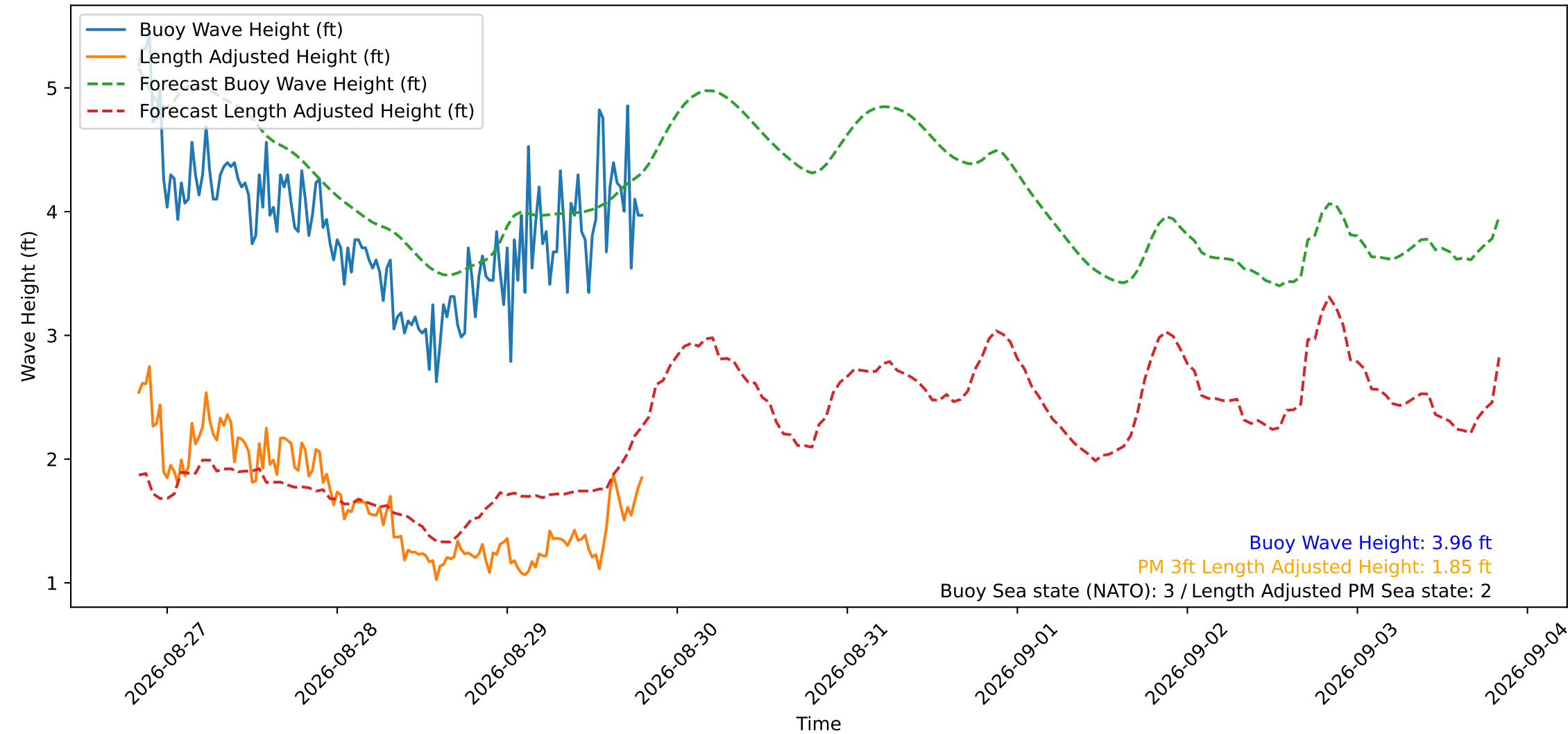
Wave Heights over Time for Green Beach at 2026-08-29 19:51:14
