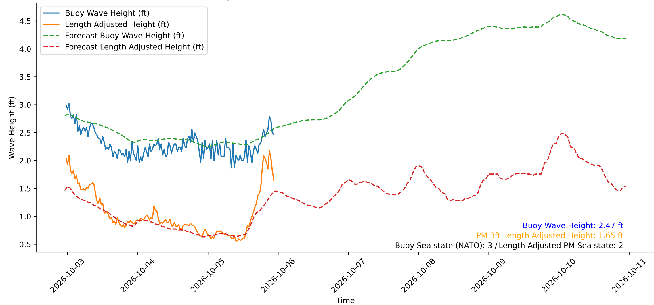
Wave Heights over Time for Oceanside Harbor at 2026-10-05 23:20:30
