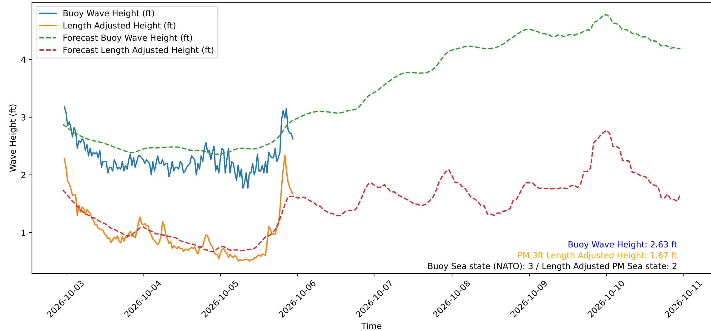
Wave Heights over Time for Green Beach at 2026-10-05 23:21:16
