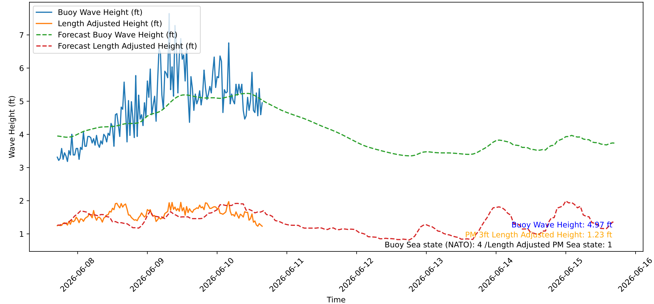
Wave Heights over Time for Red Beach at 2026-06-10 16:50:47
