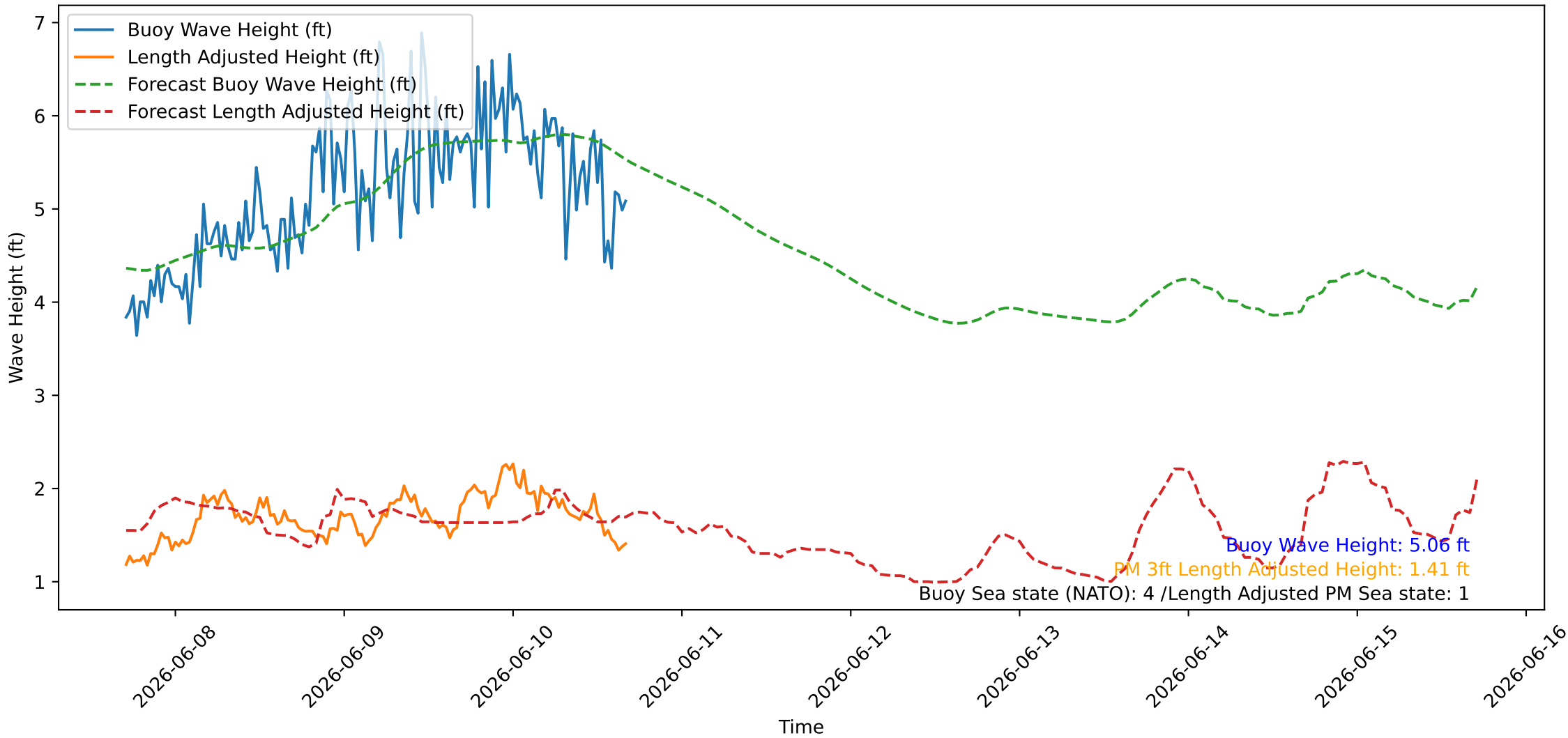
Wave Heights over Time for Green Beach at 2026-06-10 16:51:11
