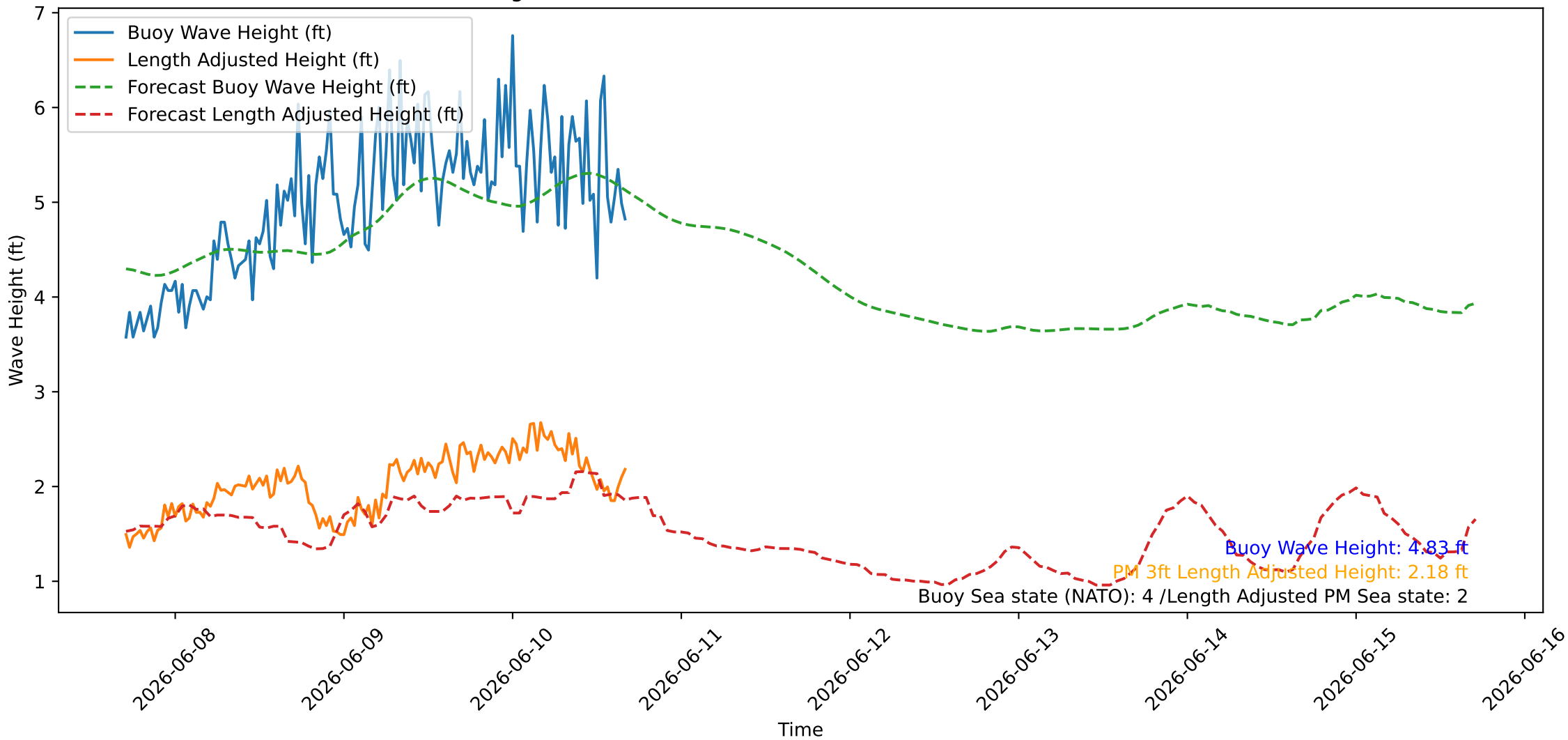
Wave Heights over Time for Oceanside Harbor at 2026-06-10 16:50:26
